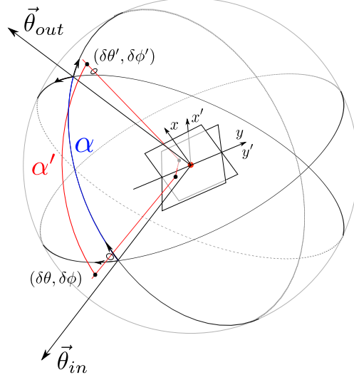
Figure 3.24 – If the parametrization of the BRDF, or BTDF, follows the equatorial plane, we can use additive notations of angles. To first order, the angular difference is \alpha' \simeq \alpha - (\delta\theta_1 - \delta\theta_2)
