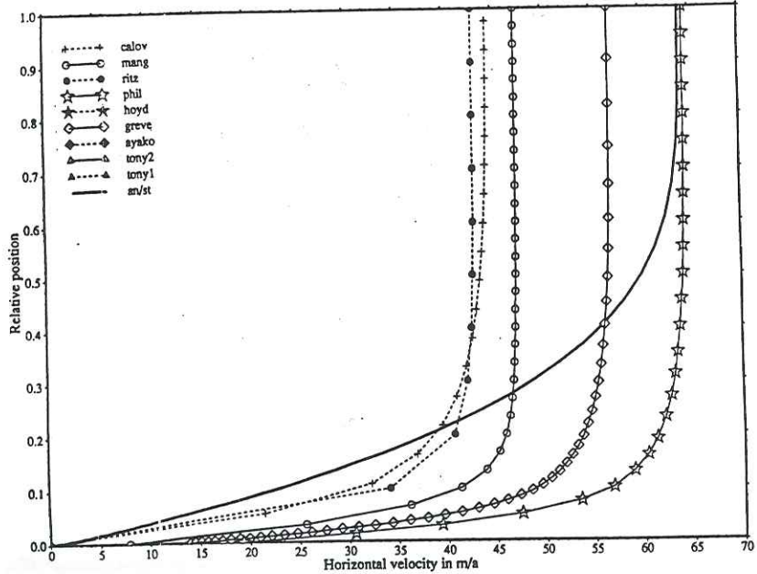
Horizontal velocity profile at the midpoint for SS-MM-L2
