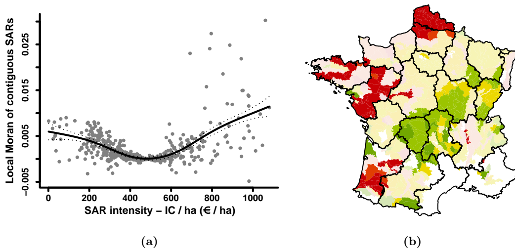
Figure V.3: Spatial aggregation (local Moran) of the intensity of Small Agricultural Regions (SARs). Intensity is expressed by the means of the Input Cost/ha indicator (“ IC/ha ”). (V.3a) Each point stands for a SAR. The value of the local Moran of contiguous SARs is plotted against the SAR IC/ha value. Black curve: generalized additive model determining the average relation between the SAR IC/ha and local Morans. Dotted curves: 95% confidence interval. (V.3b) Map of SARs IC/ha values and local Moran significance. The color indicates the IC/ha value of a SAR while the brightness reveals whether the IC/ha value is significantly auto-correlated with the ones of contiguous SARs. Legend is the same than in Fig. V.2, continuous IC/ha values are represented in 6 classes from lowest (green) to highest (red) level. Dark colors: significant auto-correlation with IC/ha of contiguous SARs, pale colors: no significant auto-correlation.
