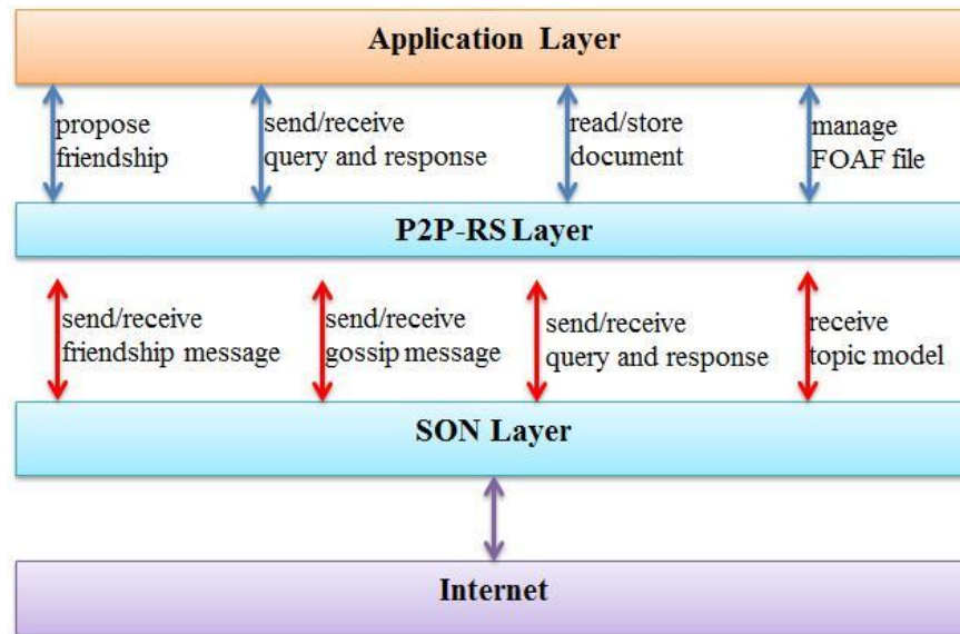
Figure 5.1. Layered architecture of P2P-RS
