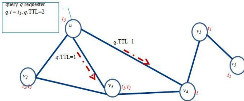
a) u submits and forwards q .
