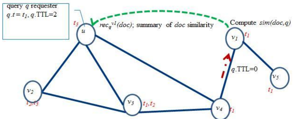
c) Receiver returns recommendations to u , and stops redirecting q , because q.TTL = 0 .
