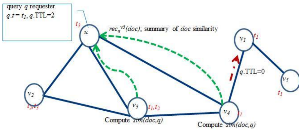
b) Receivers return recommendations to u , and redirect q while q.TTL \neq 0 .
