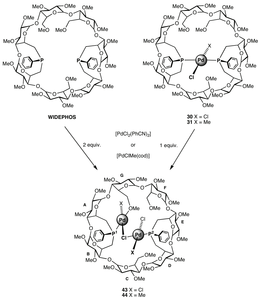
Scheme 5. Synthesis of dinuclear palladium(II) complexes 43 and 44 .
