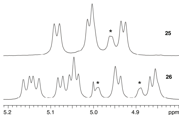
Figure 21. Partial view of the ^1\text{H} NMR spectra in \text{CDCl}_3 recorded at 300.1 MHz of compounds 25 (top) and 26 (bottom), showing the anomeric protons (H-1). Asterisks denote \text{H-6}^{\text{A,D}} protons.
