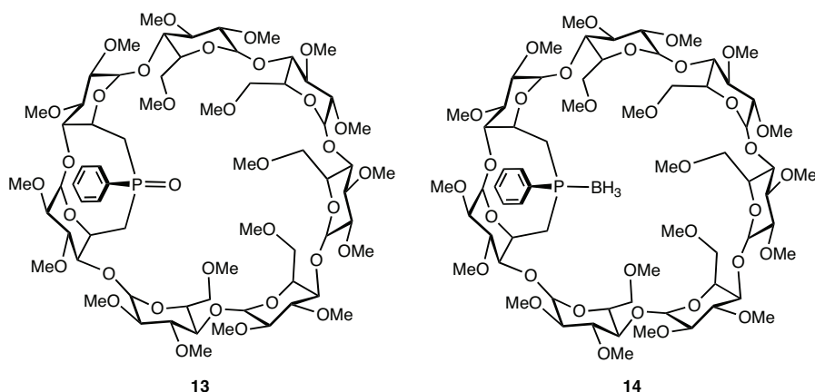
Figure 12. Compounds 13 and 14 .
