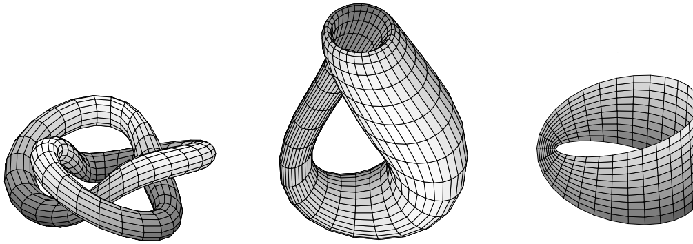
Figure 2.1: Examples of parametric surfaces. Left: the Knot surface is the only 2D-manifold of these examples. Middle and right: the Klein Bottle and the Möbius strip are non-orientable . The Klein bottle also contains self-intersections, whereas the Möbius strip is a bounded surface of genus 1 with only one edge.
