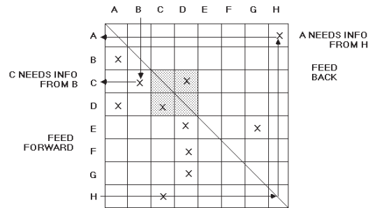
Figure 2-9 An example of a Design Structure Matrix (Holttä-Otto and de Weck 2007)
