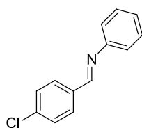
127 C 13 H 10 ClN M=215.68 g/mol
