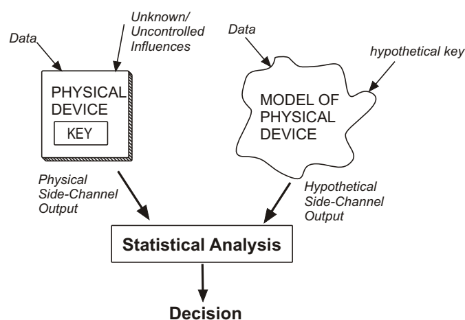
Figure 4.1.: Differential power analysis principle [80]
