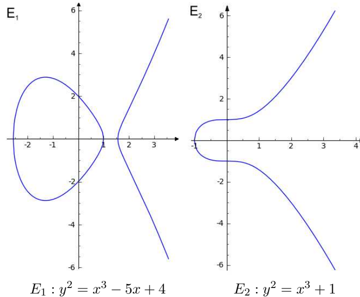
Figure 2.1.: Elliptic curves over \mathbb{R} .
