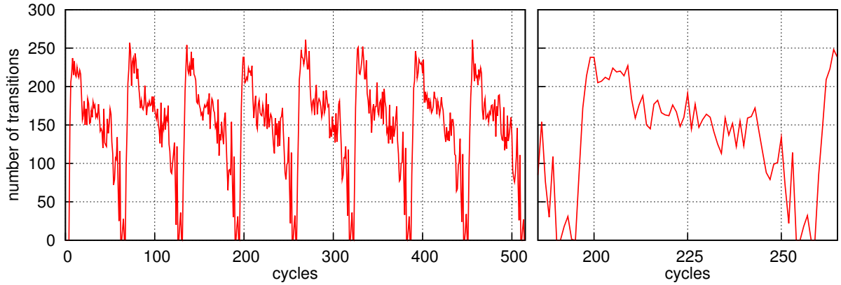
Figure 4.6.: Useful activity measurement results for random GF(2^m) multiplications with Maslov algorithm (left). Extract for a single representative multiplication (right).
