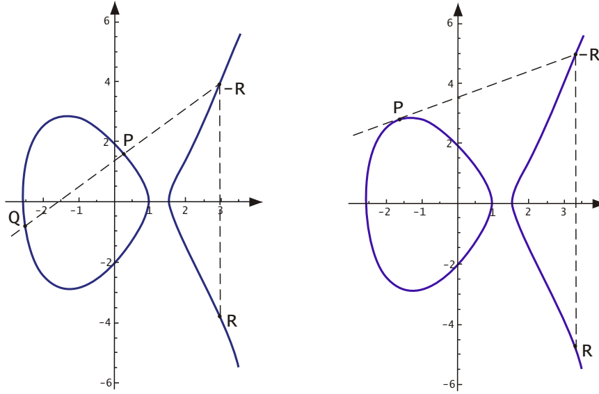
Addition P + Q = R
