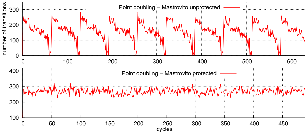
Figure 4.14.: Useful activity measurement results for 2P operation for unprotected (top figure) and protected (bottom figure) GF(2^m) operators.
