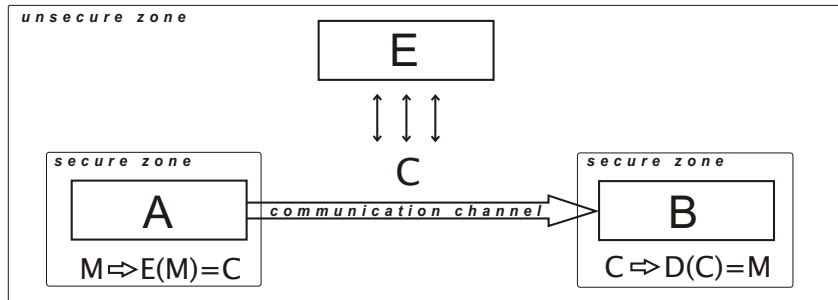
Figure 1.2.: Secure communication model
