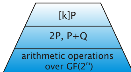
Figure 1.6.: ECC cryptosystem layers
