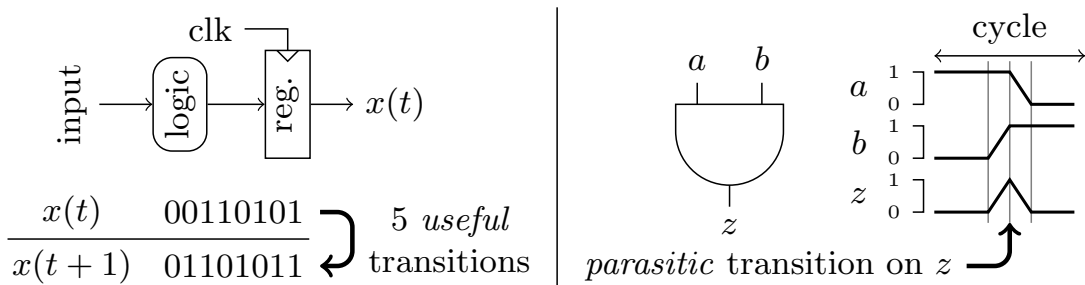
Figure 4.2.: Useful (left) and parasitic (right) transitions.
