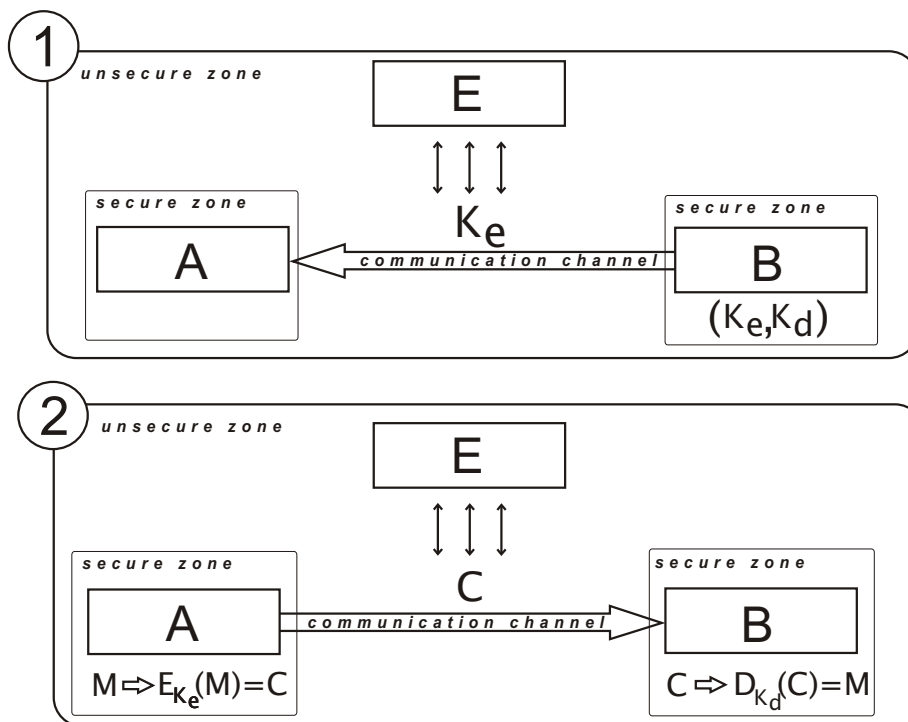
Figure 1.4.: PKC communication model
