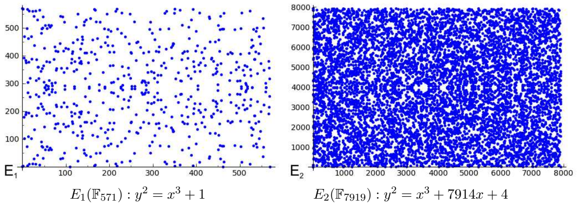
Figure 2.2.: Elliptic curves over \mathbb{F}_p .
