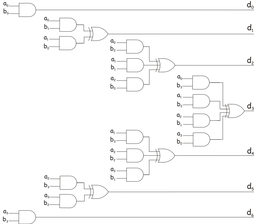
Figure 3.1.: Idea of circuit performing shift-and-add method for m = 4
