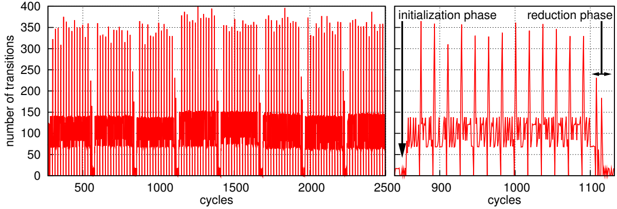
Figure 4.5.: Useful activity measurement results for random GF(2^m) multiplications with Montgomery algorithm (left). Extract for a single representative multiplication (right).
