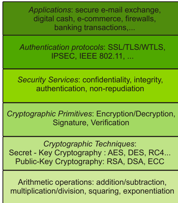
Figure 1.5.: Security layer model [8, 98]
