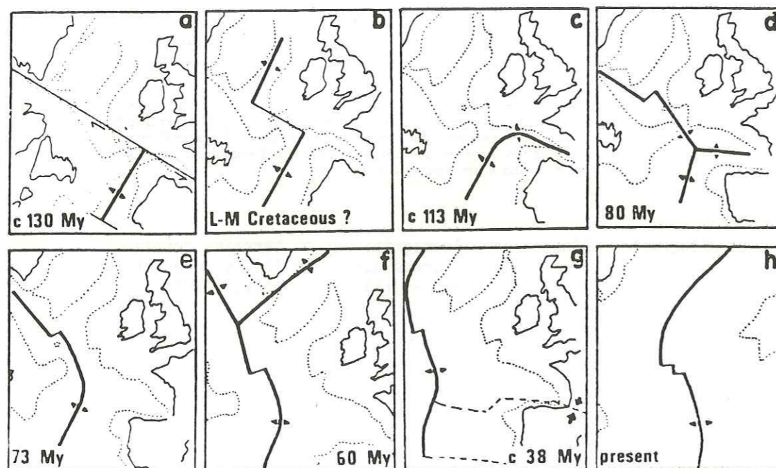
Fig. 15. The changing development of the Mid-Atlantic Ridge (a) at approximately 130 m.y. ago, the separation of Iberia and Newfoundland and the proposed truncation of the M.A.R. by a NW-SE trending transcurrent fault, possibly later modified into a transform fault (b) during the ridge extension into Rockall Trough [36]; (c) at approximately 113 m.y., the M.A.R. extends eastward and the rotation of Iberia away from France commences; (d) development of a triple ridge junction at 80 m.y., and (e) by 73 m.y., the Biscay arm of the triple junction has become extinct, but the M.A.R. remains convex to the east until a change in spreading direction occurs at 60 m.y., (f); (g) between 20 and 45 m.y. ago the compression between Iberia and France effects the Pyrenean orogeny; (h) the present situation.
