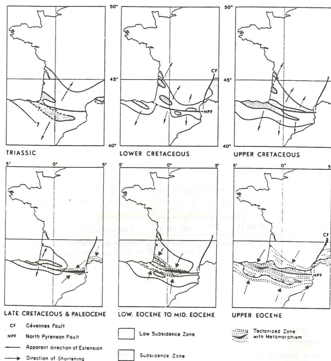
Fig. 2. Schematic diagrams showing the evolution of subsidence and the tectogenesis within the Pyrenean domain. There is no palaeogeographic reconstruction.
