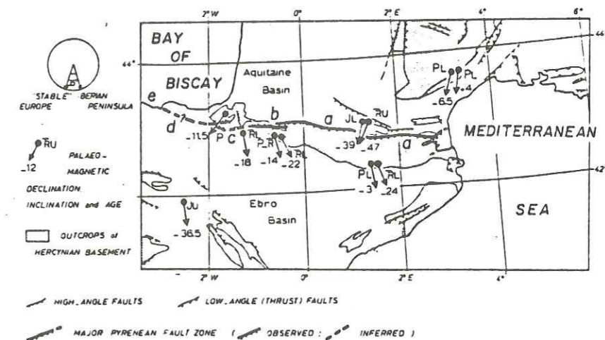
Fig. 5. Schematic tectonic map of the Pyrenees and surrounding areas. Paleomagnetic directions from Permian, Triassic, and Jurassic formations are plotted. The directions of the arrows, plotted where the rocks were collected, represent the declinations; the inclination values and the ages are indicated. Note the difference between the SW-SSW ('European') declinations and the SSE-SE ('Iberian') declinations. These paleomagnetic data are from Giriller (1968), Kruseman (1962), Schwarz (1963), Stauffer and Tarling (1971), Van der Lingen (1960), Van der Voo (1969), Van Dongen (1967), and the present paper. A major Pyrenean fault zone as the plate boundary between the Iberian Peninsula and stable Europe is proposed; the letters a, b, c, d, and e are explained in the text.
