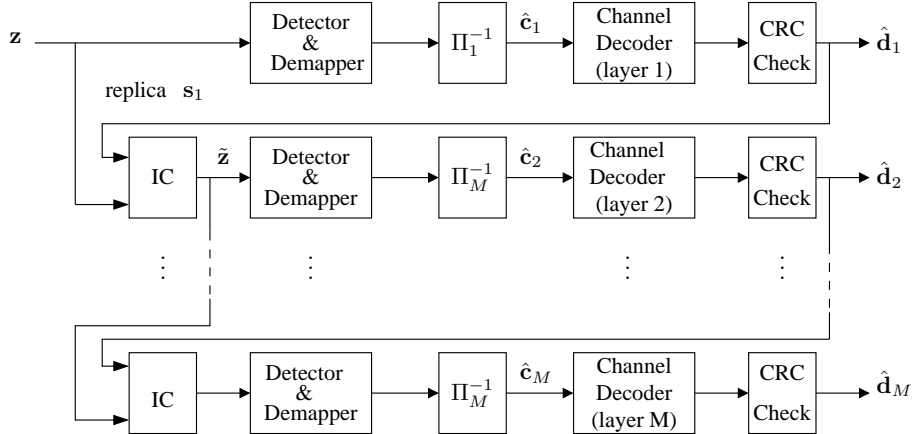
FIGURE 5.2: Successive interference cancellation receiver.
