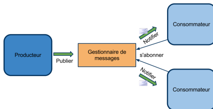
FIGURE 3.3 – Architecture publication/souscription
