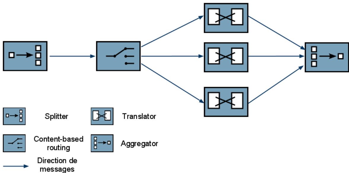
FIGURE 3.12 – Split/Aggregate - patron composé
