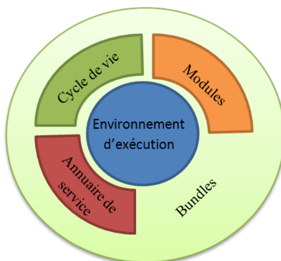
FIGURE 2.7 – Framework OSGi
