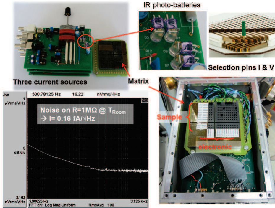
Figure 4.2.3: (a) Stacked electronic boards of our current sources on the left and the matrix on the right (b) LED and Infrared photobattery decouple the electronics from the power supply ground. (c) Cut image showing the principle of a matrix (d) Noise of the electronics at room temperature for R = 1 \text{ M}\Omega , I=0.16 \text{ fA}/\sqrt{\text{Hz}} above 100 Hz (e) Top view of utilized electronics.
