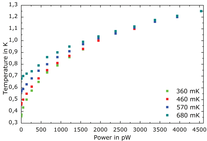
Figure 5.3.4: Electron thermometer: electronic temperature T_e versus injected power P_{\text{inj}} for different bath temperatures (different colors)
