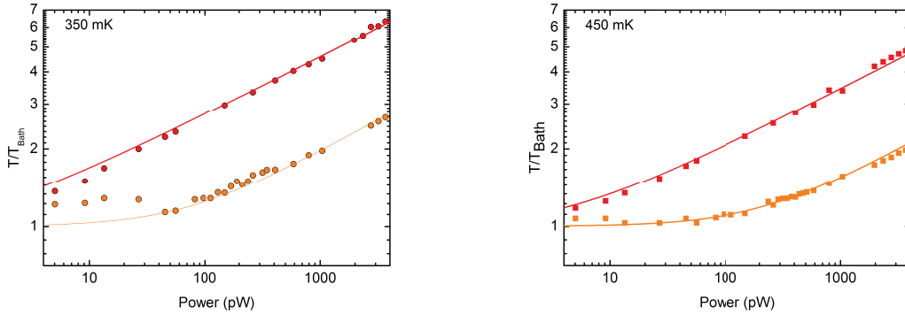
FIGURE 5.4.7: Experimental data of Electron thermometer (red symbols) at T_{\text{bath}} = 350 mK (left), 450 mK (right) fitted with the theoretical temperature evolution (red line) given by Eq. 5.3.1 for K = 80 \text{ pW}\cdot\text{K}^{-4}\cdot\mu\text{m}^{-2} and \Sigma = 2000 \text{ pW}\cdot\text{K}^{-5}\cdot\mu\text{m}^{-3} and phonon thermometer data (orange symbols) fitted by Eq. 5.2.2 (orange line) with K' = 700, \text{ pW}\cdot\text{K}^{-4}\cdot\mu\text{m}^{-2} .
