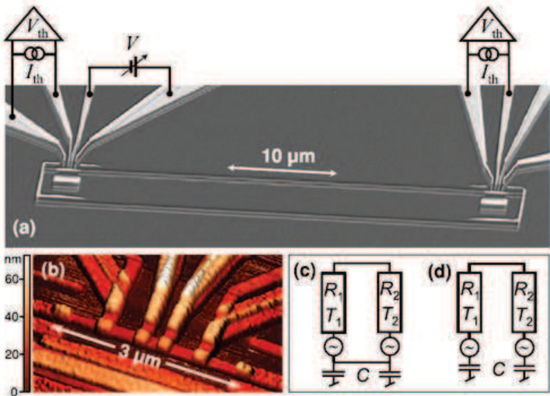
Figure 1.3.8: Experiment Ref. [89]: (a) Electron micrograph of sample A (matched impedances). Two normal islands are connected with superconducting lines into a loop to match the impedance between them and enable remote refrigeration. (b) Colored atomic force microscopy image of the island. The four NIS junctions, contacting each island in the middle part, are used to perturb and to measure the island temperature. (c) Equivalent electrical circuit of the matched (sample A) and (d) the mismatched (sample B) structures.
