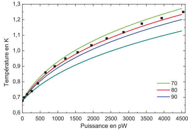
Figure 5.3.6: Experimental data of T_{bath} = 678 \text{ mK} (black square) and theoretical temperature evolution given by eq. 5.2.2 for K = 70, 80, 90, 120 \text{ pW} \cdot \text{K}^{-4} \cdot \mu\text{m}^{-2} (from the top to the bottom).
