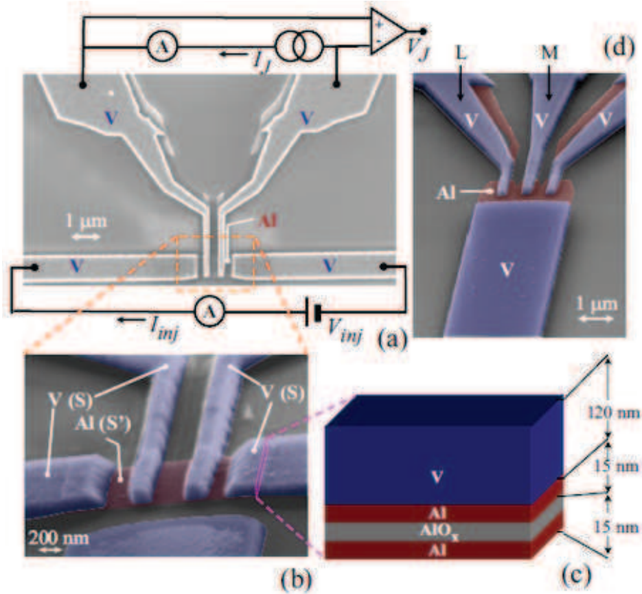
Figure 1.2.9: Vanadium-Aluminum-Vanadium micro-cooler [67]
