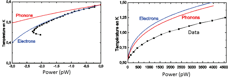
Figure 5.3.7: (a) Experimental data from Ref. [70] in the cooling regime (black linked squares) at T_{bath}=568 mK and (b) Experimental data in the heating regime (black linked squares) at T_{bath}=586 mK, theoretical T_e given by Eq. 5.3.1 and theoretical T_{ph} given Eq. 5.2.2 with fit parameters \Sigma = 2000 pW.K -5 .μm -3 , K = 40 pW.K -4 .μm -2 .
