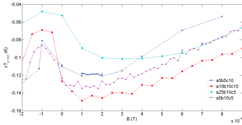
Figure 6.4.2: Electronic refrigeration \Delta T_{e\min} under B_{\perp} at T_{\text{bath}} = 300 \text{ mK} : comparison of different qp-trap geometry: a5b5c10, a10b10c10, a25b10c5 and a5b10c5
