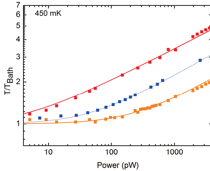
Figure 5.4.8: Experiment done at T_{\text{bath}} = 450 mK. Experimental data: electron thermometer T_e (red symbols), electron thermometer T_{\text{ph}} (orange symbols), inverted experiment T_i (blue symbols). Theoretical fit: complete thermal model (red line), strong electron-phonon coupling (orange line), strong electron-phonon coupling (blue line)
