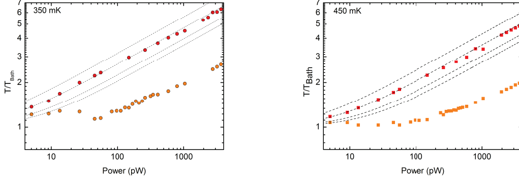
FIGURE 5.4.5: Experimental data of electron thermometer (red symbols) T_e(P_{inj}) and phonon thermometer (orange symbols) at T_{bath} = 350 mK and 450 mK and theoretical temperature evolution given by Eq. 5.2.1 for K = 10, 20, 40, 60 pW.K ^{-4} . \mu\text{m}^{-2} (black dashed lines from the top to the bottom).
