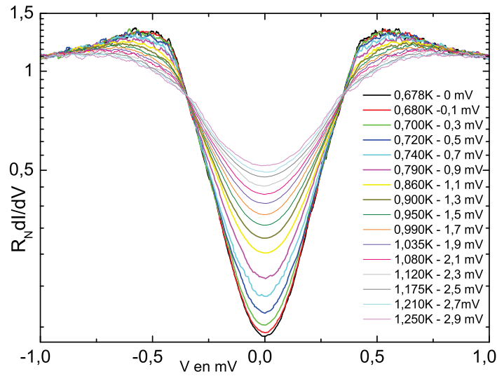
Figure 5.3.3: Electron thermometer response under voltage bias of N_1 Cu wire from 0 to 2.9 mV from the bottom to the top at T_{\text{bath}} = 0.6 K : differential conductances and T_e extracted from theoretical fits with fix parameters \Delta = 0.21 mV, R_N = 8800 \Omega , and T_0 = 0.678 K.
