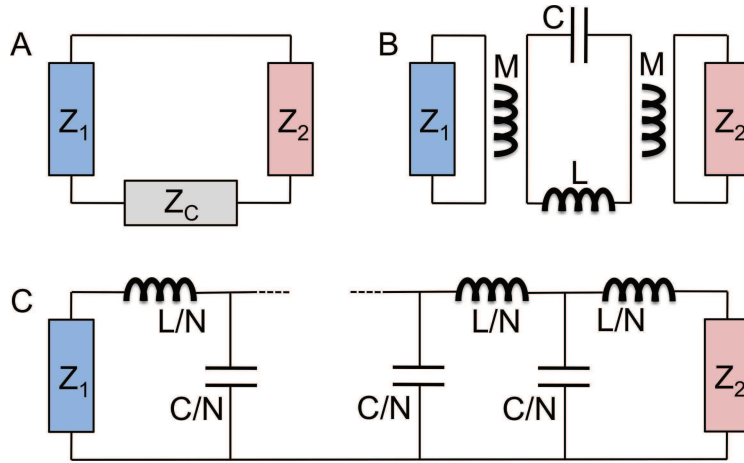
Figure 2.2.1: Top left panel, circuit A: two impedances Z_1 and Z_2 are coupled by a purely reactive coupling impedance Z_c . Top right panel, circuit B: two impedances Z_1 and Z_2 are coupled via mutual inductances to a purely reactive central circuit of total impedance Z_c (here an LC resonator). Bottom panel, circuit C: two impedances Z_1 and Z_2 are coupled via a transmission line.
