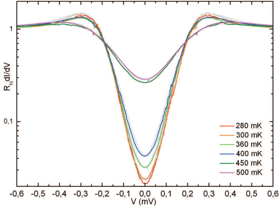
FIGURE 4.3.1: Experimental normalised conductance (continuous colorful lines) fitted with isotherm (black dotted lines) to extract the electronic temperature, for different bath temperatures.
