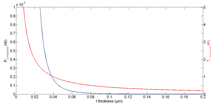
Figure 5.2.4: Crossover temperature T_{\text{crossover}} and power P_{\text{crossover}} evolution with the thickness t for parameters: \Sigma = 2000 \text{ pW } \mu\text{m}^{-3} \text{ K}^{-5} , K = 80 \text{ pW } \mu\text{m}^{-2} \text{ K}^{-4} , length = 70 \mu\text{m} , width = 0.3 \mu\text{m} , and T_{\text{bath}} = 0.3 \text{ K} .
