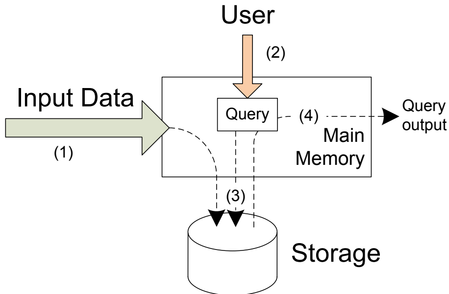
Figure 1.1: DBMSs information processing.
