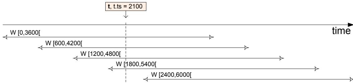
Figure 4.2: Example of tuple contributing to several windows
