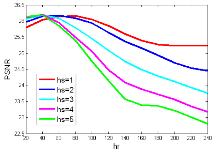
Figure 5.6: PSNR assessment according to h_s and h_r .
