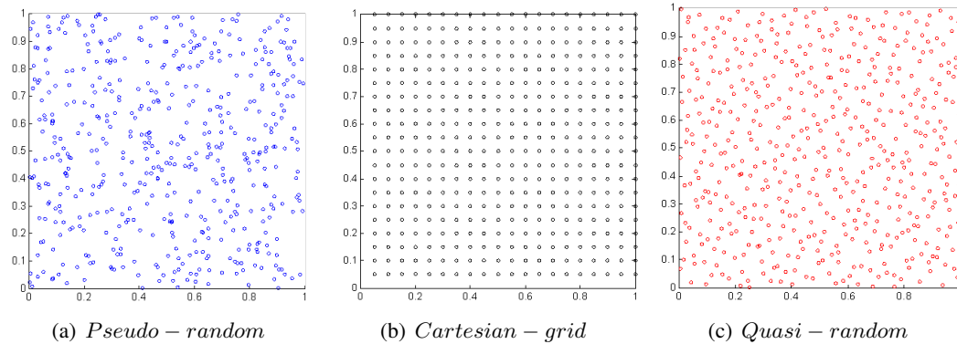
Figure 6.8: Illustration of the three studied random number generators.
