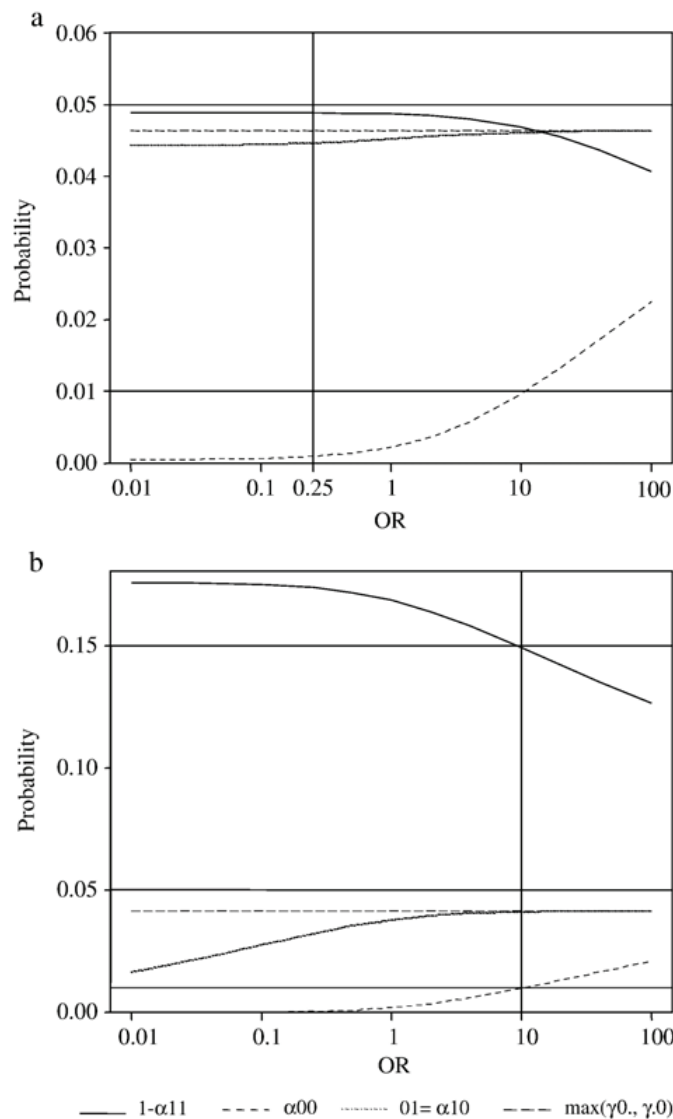
Fig. 5. Actual risks values (Probability) \alpha_{00} , \alpha_{01} , \alpha_{10} , \gamma_{0.} , \gamma_{10} and 1-\alpha_{11} in the case of a deviation from the assumption made on \Phi ( \Phi=0.25 , a and \Phi=10 , b) according to different hypotheses on risks ( \alpha , \gamma and \beta ) and rates for Conaway and Petroni designs. a: \alpha=1\% ; \gamma=5\% ; \beta=5\% ; P_{RO}=0.75 ; P_{TO}=2.75 . b: \alpha=1\% ; \gamma=5\% ; \beta=15\% ; P_{RO}=0.40 ; P_{TO}=0.40 .
