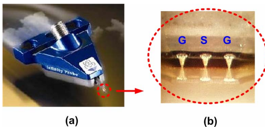
Figure 3. 5. Infinity probe.
