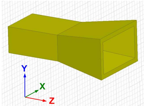
Figure 5. 2 Simulation model of the horn antenna
