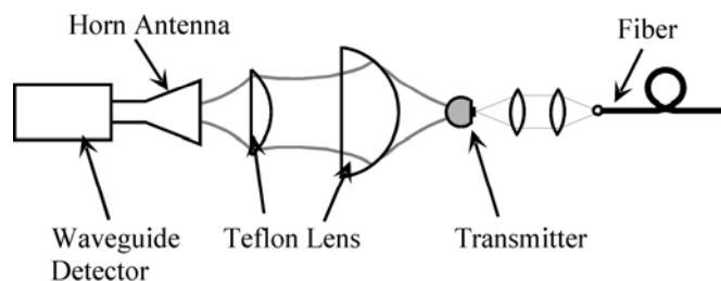
Figure 1. 17 Measurement setup of the transmitter [72].
