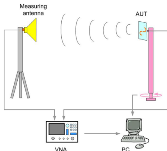
Figure 1. 3 Classical radiation pattern characterization setup.
