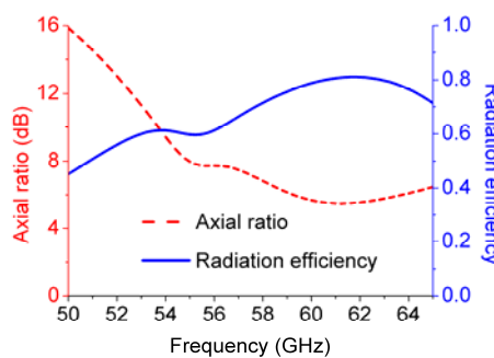
Figure 2. 12 Simulated axial ratio and radiation efficiency in the broadside direction ( \theta = 0^\circ ) as a function of frequency.
