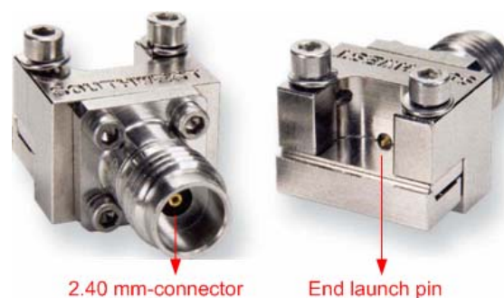
Figure 4. 7 Front view and back view of the 2.40 mm-connector [14].
