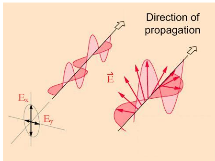
Figure 2. 5 Elliptical polarization.
