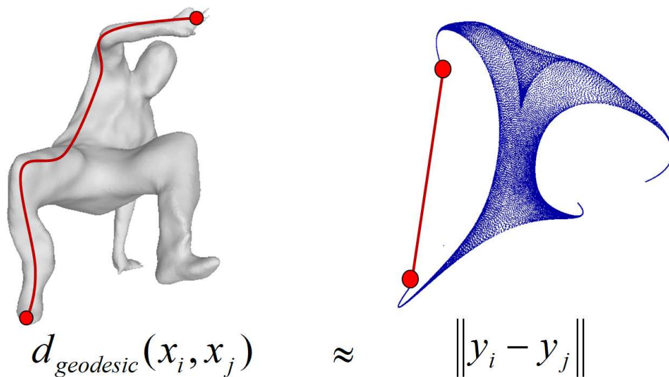
Figure 3.3: Distance preserving isometric embedding of a visual shape. The geodesic distance d_{\text{geodesic}}(x_i, x_j) between two points x_i, x_j \in \mathcal{M} on visual shape is equivalent to the Euclidean distance between their mapped images (y_i, y_j) \in \mathcal{Y} in the embedding space \mathcal{Y} \subset \mathbb{R}^n
