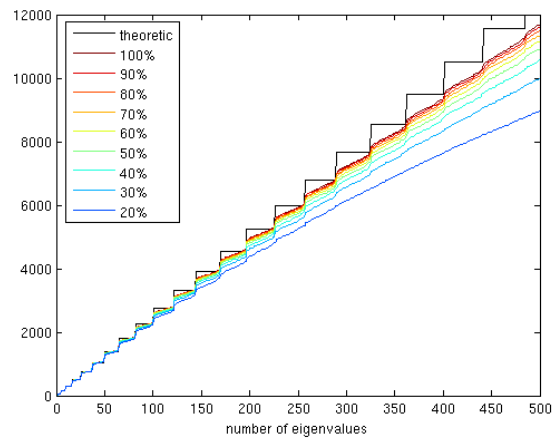
Figure 3.12: The eigenvalues of many discrete triangulated meshes of a sphere with decreasing resolution are compared with the theoretical eigenvalues using the cotangent weighting.
