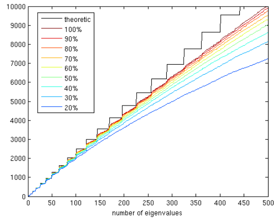
Figure 3.11: The eigenvalues of many discrete triangulated meshes of a sphere with decreasing resolution are compared with the theoretical eigenvalues using the Gaussian weighting.
