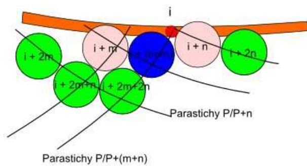
Figure 13: Geometrical scheme explaining transitions of phyllotaxis in the Fibonacci branch upon decrease of parameter \Gamma . (A) Transition from a (3,5) phyllotaxis to a (5,8) phyllotaxis. The blue organ become closer to the initium i , defining new direct neighbors and new parastichies. (B) Generalization to the transition of a Fibonacci spiral of order ( m,n ) to order ( n, m+n ).
