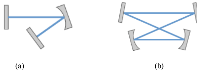
Fig. 2.1 A simple linear optical resonator with a curved folding mirror (a) and a four-mirror bow-tie ring resonator (b) [41].
