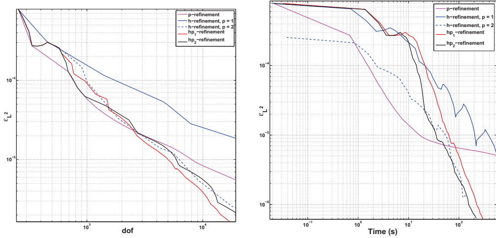
Figure 7.9: L^2 -error versus dof (left) and time (right) for the MMS1 benchmark with different refinement strategies
