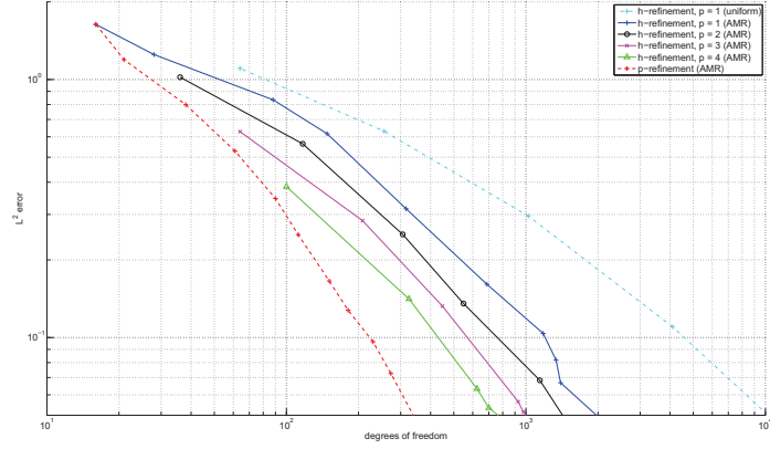
Figure 2.26: Comparison of different refinement strategies
