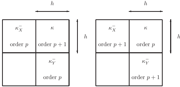
Figure 2.19: Configuration with a local increase of the basis order C_{p \rightarrow p+1} (left) and decrease C_{p+1 \rightarrow p} (right)
