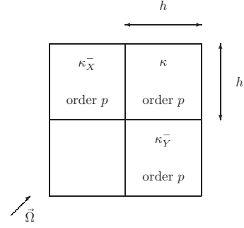
Figure 2.16: Configuration with a conforming mesh and a uniform basis order
