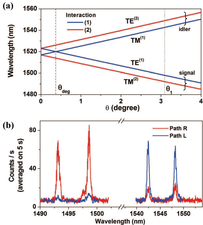
Fig. 2. Tunability curves and emission spectra. (a) Line: Calculated tuning curves as a function of the pump incident angle for a pump wavelength of 760 nm and the structure described in the text. Dashed lines show the selected incident angles for the experiments. (b) SPDC spectra for an angle of incidence of \theta_1 = 3.1^\circ in the photon-counting regime. The peaks correspond to the four kinds of photons that can be generated via the two possible interactions. The background noise here is due to the dark counts of the detectors. Path R(L) denote the detection path of photons exiting the right (left) facet.
