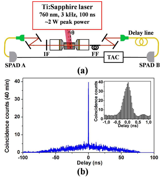
Fig. 8. (Color online) (a) Experimental setup for coincidence counting. IF and FF represent an interference filter (10 nm bandwidth) and a fibered filter (1 nm bandwidth), respectively, used to reduce luminescence noise. SPAD A and B are two single-photon avalanche photodiodes. (b) Coincidence histogram acquired in 40 min for a pump peak power of 2 W. Inset: zoom on the coincidence peak.
