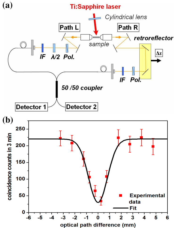
Fig. 3. Two-photon interference set-up and HOM dip. (a) Sketch of the experimental setup used for the two photon interference. The two photons generated in the selected interaction are combined in a fibered 50/50 coupler, where quantum interference occurs. The polarization of one of the two photons is rotated of 90^\circ with a half-wave plate. A retroreflector placed in one arm of the interferometer is used to adjust the relative delay of the two photons. (b) Coincidence counts in 3 min (total counts - accidental counts) as a function of the relative length of the two arms. The accidental coincidence counts accounts for 14% of the total coincidence counts outside the dip. The coincidence windows taken into account is 400 ps. The error bars are determined by the Poisson distribution (the square-root sum of the total coincidence counts) and the solid line is the numerical fit.
