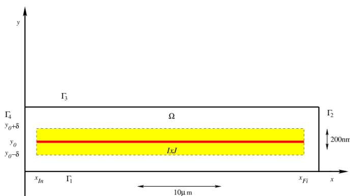
Figure 2.1: Area of the cytoplasm where intracellular transport is modelled: \Omega = [0, L_x] \times [0, L_y] . The yellow rectangle ( \mathbf{I} \times \mathbf{J} = [x_{I_n}, x_{F_i}] \times [y_0 - \delta, y_0 + \delta] ) represents the attraction area of the microtubule filament, the red strip is the microtubule, positioned in y_0 .
