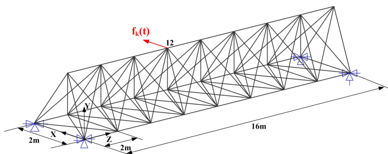
FIGURE 3.10: Mass-spring model
