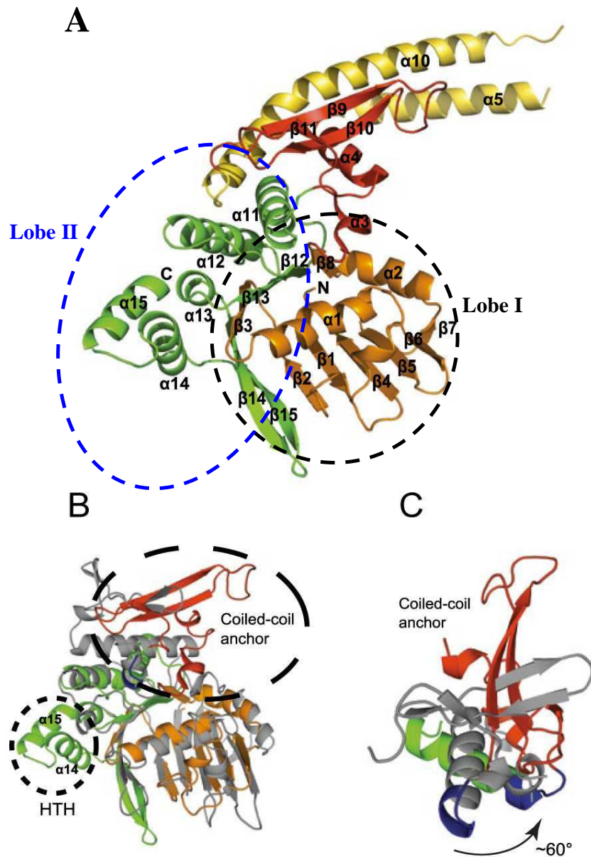
Figure 45: RecNhead domain crystal structure. A) RecNhead domain crystal structure adopts a Rossman fold, typical for nucleotide binding proteins, and shares structural similarity with the SMC and SMC-like proteins. B) Superposition of RecNhead domain (colored as shown in A) with pfRad50 head domain (grey) also referred to as the ATPase domain. An HTH at the C-terminus of RecNhead, which is not conserved in pfRad50, represented a unique feature. C) Different orientation of the RecN-Rad50 overlay, with the coiled-coil anchor motif (in red) and the signature sequence (in blue) of RecNhead domain rotated \sim 60 degrees to respect to their corresponding in Rad50. The different orientation of the signature sequence, crucial for ATP-binding, might reflect differences in nucleotide binding mechanism between these two homologous proteins.
