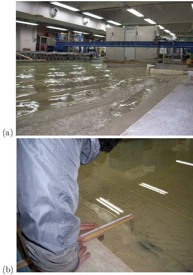
FIG. 9.3 – Wave basin experiments of 17 and 18 January 2011, Coastal Engineering Laboratory, the University of Tokyo; (a) Propagation of southern waves near the port (b) Measurements of shoreline position.
