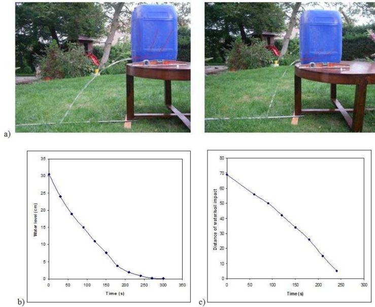
FIG. 8.2 – Example of atypical experiments in fluid mechanics : Emptying of a 35 liters plastic jerry can. (a) Experiments. Evolution of water level (b) and distance of water/soil impact (c) vs time.
