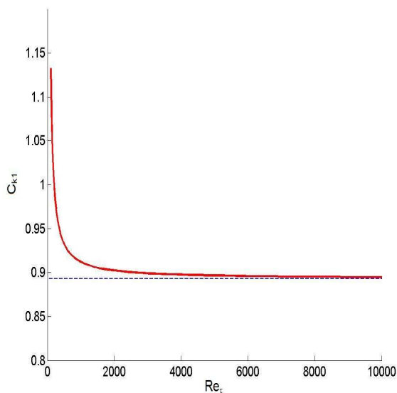
FIG. 5.3 – Variation of coefficient C_{k1} , Eq. (5.22).
