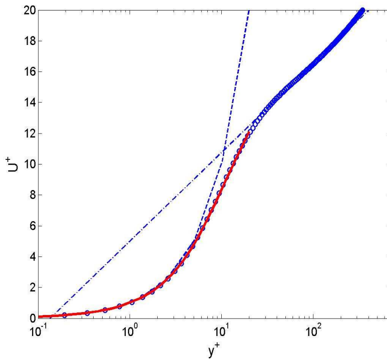
FIG. 6.1 – Mean streamwise velocity profile U^+(y^+) for Re_\tau = 642 . o, DNS data [60]. Curves : bold red solid line, solution of Eq. (6.2) with Eq. (6.10) ( C_\nu = 0.3 , A_l^+ = 26 , A_k^+ = 8 and B = 0.14 ); dashed line, U^+ = y^+ ; dash-dotted line, U^+ = 2.5 \ln(y^+) + 5.0 .
