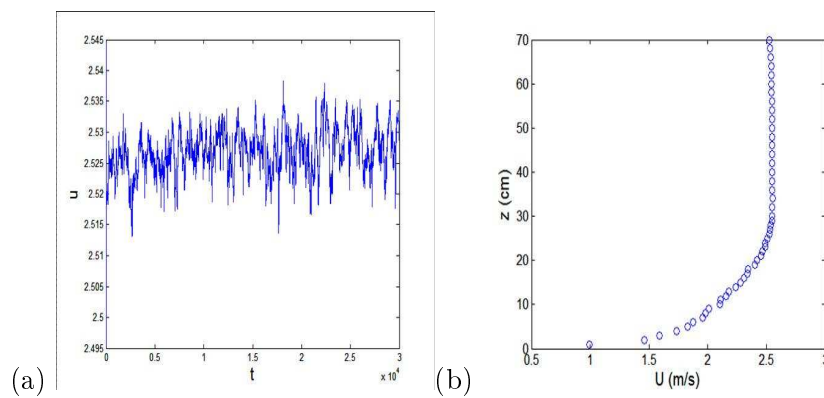
FIG. 9.2 – (a) Sample of velocity measurement; (b) experimental mean streamwise velocity profile.
