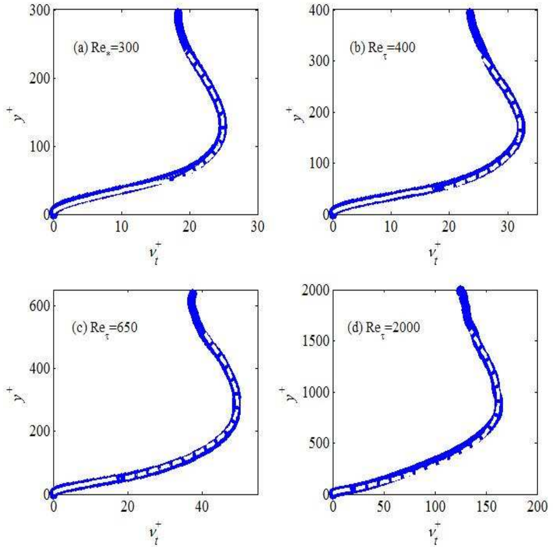
FIG. 6.4 – Eddy viscosity profiles for different Reynolds numbers Re_\tau . Symbols (bold blue lines) : DNS data ; white dashed lines : Eq. (6.16) ; white solid lines : Eq. (6.8).
