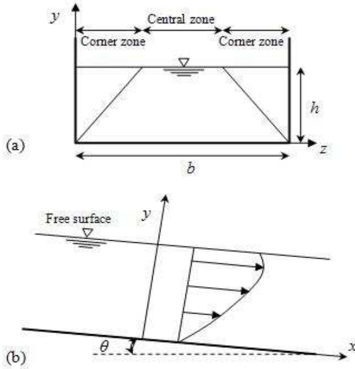
FIG. 6.8 – Definition sketch for steady uniform open-channel flow.
