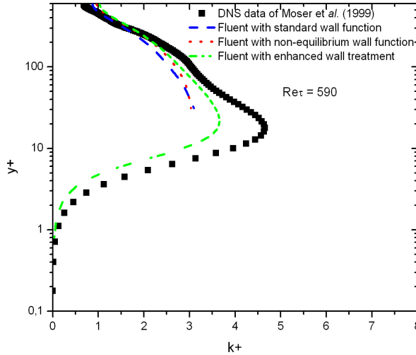
FIG. 5.7 – Comparison between predicted profiles of turbulent kinetic energy using standard k - \varepsilon model with different wall treatments : Standard Wall Functions, Non Equilibrium Wall Function and Enhanced Wall Treatment and DNS data.
