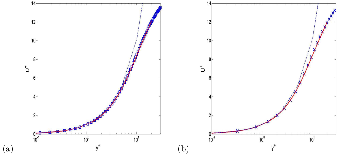
FIG. 6.2 – Mean streamwise velocity profiles U^+(y^+) for Re_\tau \geq 395 . Symbols, DNS data. Curves, Thin dashed line, U^+ = y^+ . Red solid lines, solution of Eq. (6.2) with Eq. (6.10) ( A_l^+ = 26 , A_k^+ = 8 ); (a) Re_\tau = 395 , squares [60], solid line ( C_\nu = 0.3 , B = 0.132 ); (b) Re_\tau = 2003 , \times [58], solid line ( C_\nu = 0.3 , B = 0.158 ).
