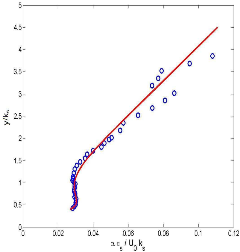
FIG. 7.6 – Comparison of the mean measured normalized \alpha \varepsilon_s (symbols) over medium sand bed [106], with calculations from proposed equations (curve).
