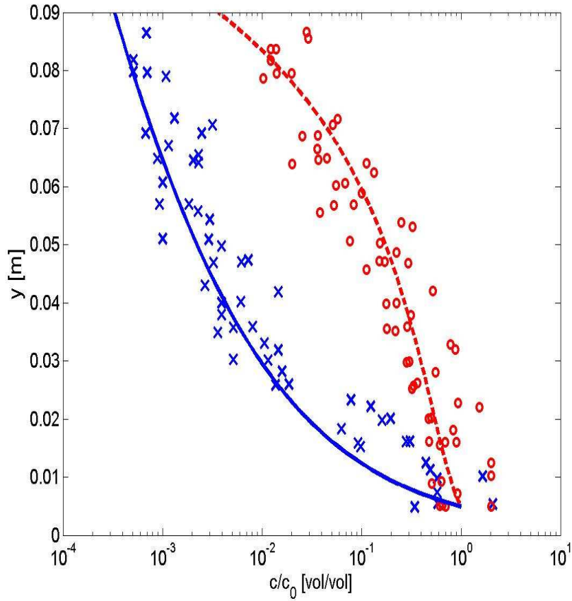
FIG. 7.4 – Time-averaged concentration profiles over wave ripples : gradient (Fickian) diffusion model with proposed \beta(y) -function. symbols, measurements [76], o, Fine sand ( \omega_s = 0.65 \text{ cm/s} ); \times , coarse sand ( \omega_s = 6.1 \text{ cm/s} ). Curves, model with \alpha_s = 0.025 \text{ m/s} ; dashed line (fine sand) \delta_s = L_v = \frac{\delta}{C_1} = 0.022 \text{ m} ; solid line (coarse sand) \delta_s = \frac{\delta}{(C_1 - C_\beta)} = 0.24 \text{ m} .
