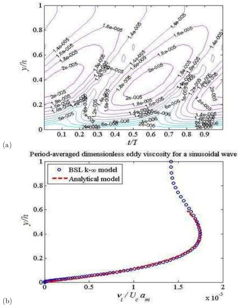
FIG. 7.1 – Dimensionless eddy viscosity ; (a) : Temporal and Spatial Variation ; (b) : Period-averaged dimensionless eddy viscosity ; for a sinusoidal wave [10].
