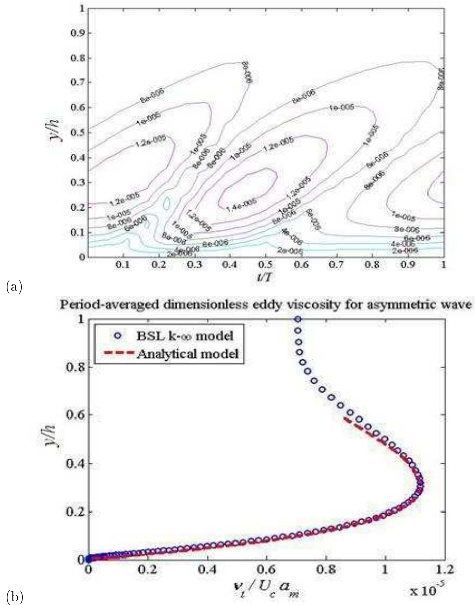
FIG. 7.2 – Dimensionless eddy viscosity ; (a) : Temporal and Spatial Variation ; (b) : Period-averaged dimensionless eddy viscosity ; for an asymmetric wave [10].
