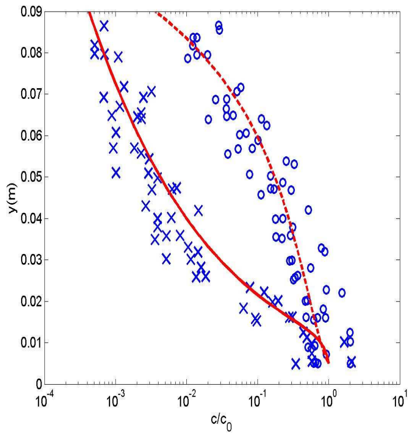
FIG. 7.5 – Time-averaged concentration profiles over wave ripples. Symbols, measurements (McFetridge and Nielsen, 1985), (o) fine sand; (x) coarse sand. Curves are solutions of gradient diffusion model with proposed \beta(y) and \alpha(y) ( = 1/f_s(y) ) functions.
