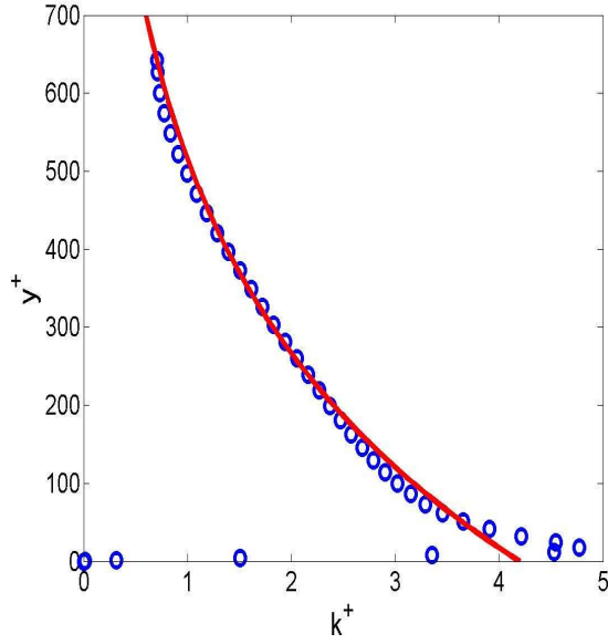
FIG. 5.1 – Turbulent kinetic energy. o, DNS data [60] for Re_\tau = 642 ; Curve, Eq. (5.20) with A_1^+ = 360 and D_1 = 4.2 .
