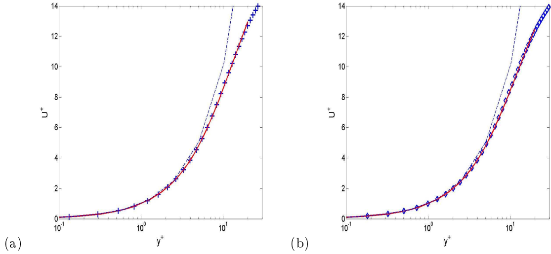
FIG. 6.3 – Mean streamwise velocity profiles U^+(y^+) for Re_\tau < 395 . Symbols, DNS data; Curves, Thin dashed line, U^+ = y^+ ; Red solid lines, solution of Eq. (6.2) with Eq. (6.10) ( A_l^+ = 26 , A_k^+ = 8 ); (a) Re_\tau = 109 , + [60], solid line ( C_\nu = 0.2 , B = 0.11 ); (b) Re_\tau = 150 , diamonds [60], solid line ( C_\nu = 0.25 , B = 0.116 );
