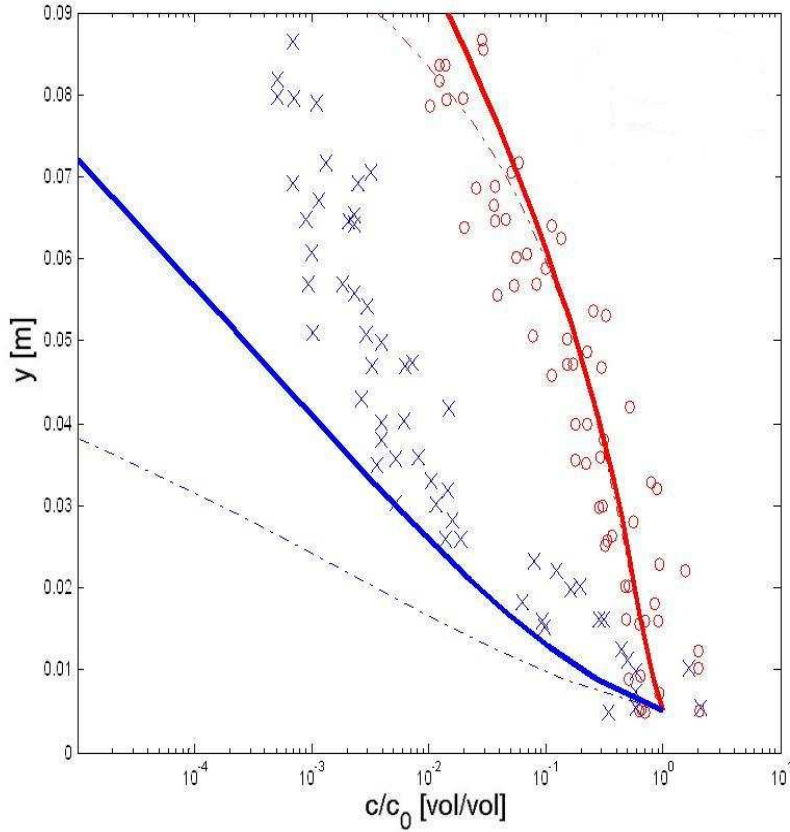
FIG. 7.3 – Time-averaged concentration profiles over wave ripples : gradient (Fickian) diffusion model versus finite-mixing-length model. symbols, measurements [76], o, Fine sand ( \omega_s = 0.65 \text{ cm/s} ); \times , coarse sand ( \omega_s = 6.1 \text{ cm/s} ). Dash-dotted lines are solutions of gradient (Fickian) diffusion model (Eq. 7.13) while solid lines are solutions of finite-mixing-length model (Eq. 7.16), \lambda = 1 , y_0 = 0.005 \text{ m} , v_{m0} = 0.025 \text{ m/s} , L_v = 0.022 \text{ m} .
