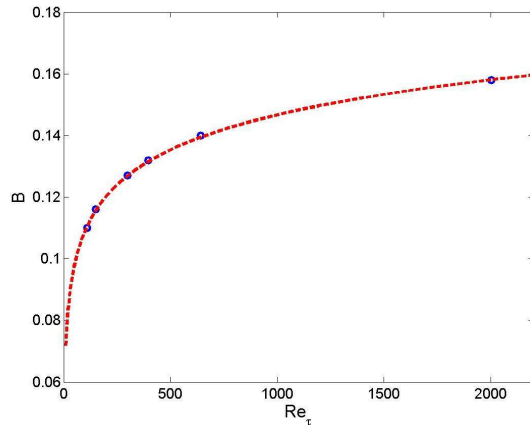
FIG. 5.6 – Dependency of the coefficient B on the Reynolds number Re_\tau . o, values obtained from DNS data ; Curve, proposed function (5.35).
