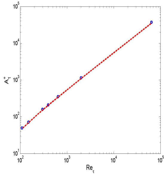
FIG. 5.2 – Calibration of A_1^+ by DNS data. o, DNS data; Curve, Eq. (5.21).
