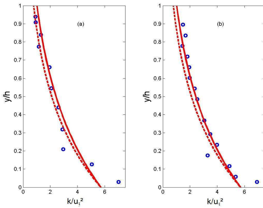
FIG. 5.4 – Comparison of TKE profiles from Eq. (5.8) with : dashed lines, C_{k1} = 1 ; solide lines, C_{k1} = 0.86 and o, experimental data of Sukhodolov et al. [101].
