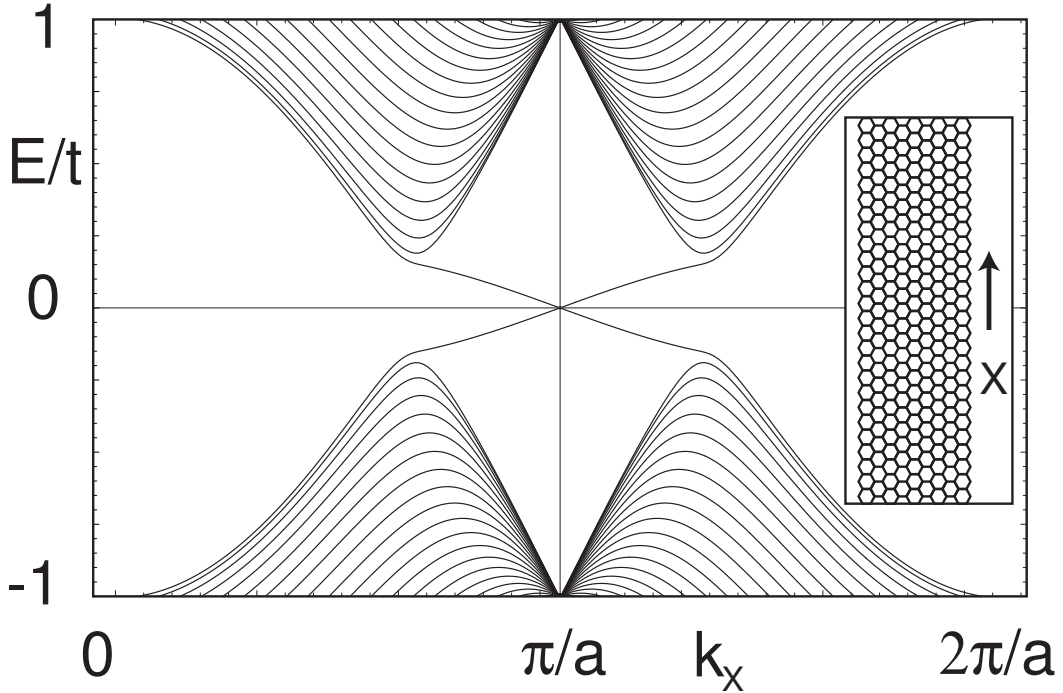
Figure 7.8: One dimensional energy bands for a zigzag ribbon (shown in inset) modeled by (7.12) with \lambda_{\text{so}} = 0.03t . The bands crossing the gap are spin filtered edge states. Adapted from [23].
