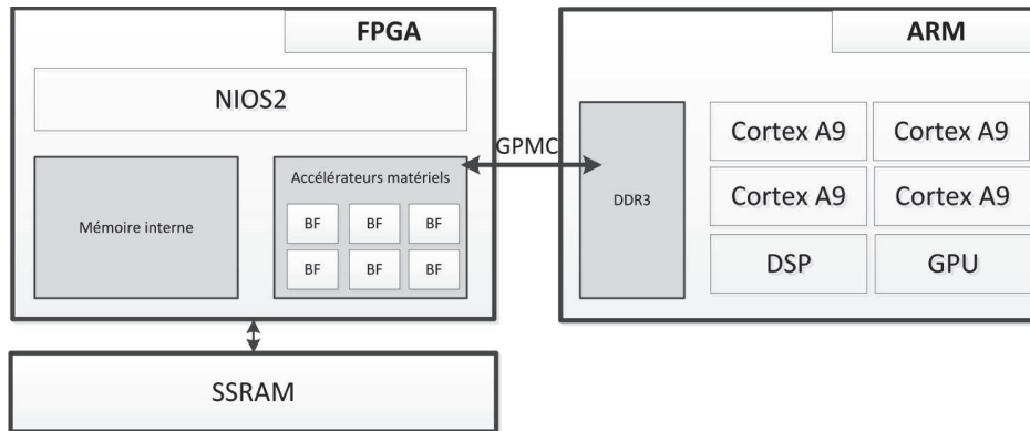
FIGURE 4.27: Architecture envisageable
