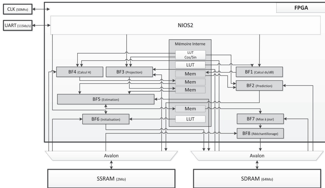
FIGURE 4.21: Architecture proposée
