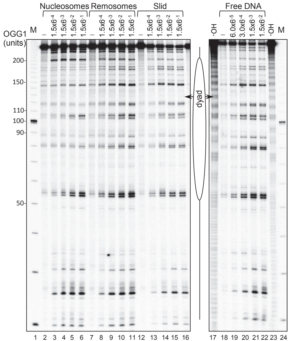
Supplementary Figure 5: Remosomes are capable of performing the same extent of Base excision repair initiation as that of slid. Centrally positioned nucleosomes were reconstituted on ^{32}\text{P} 5' labeled 255bp 601 DNA fragment which is UV irradiated. (A) Analysis of hOGG1 enzymatic activity within the nucleosomal and the linker DNA. The nucleosomal species including nucleosomes, remosomes and slid were gel eluted and then subjected to enzymatic treatment by increasing amounts of hOGG1. The nucleosome species were incubated with hOGG1 at 29°C for 90 minutes. The DNA was purified before treating with APE1. This enzymatic cleavage of the apurinic sites was carried out at 37°C for 2 hours. The cleavage pattern of the isolated DNA was analysed using an 8% denaturing PAGE. (B) RSC promotes hOGG1 cleavage of the lesions that are at the edge and are exposed to the solution. Lane numbers 17 and 23 represent a hydroxyl radical footprint of the nucleosomes and helps us determine the parts of the fragment that are facing inside at the octamer and those that are facing the solution. (C) Increasing amounts of hOGG1 gives rise to a signature cleavage pattern in the DNA. Lanes 18-22 represent the DNA that is subjected to hOGG1 treatment as mentioned in (A).
