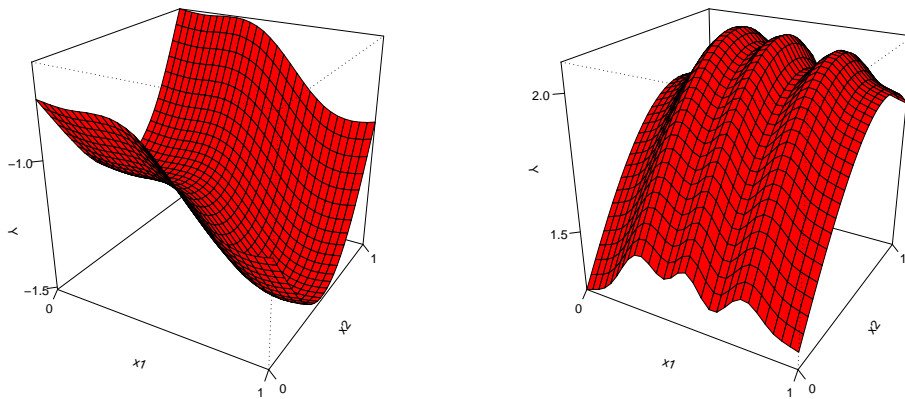
(a) (\sigma_1^2, \theta_1) = (1, 0.4) et (\sigma_2^2, \theta_2) = (1, 0.4) (b) (\sigma_1^2, \theta_1) = (0.01, 0.1) et (\sigma_2^2, \theta_2) = (1, 0.4)
