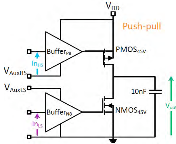
FIGURE 3.12 – Configuration PushPull
