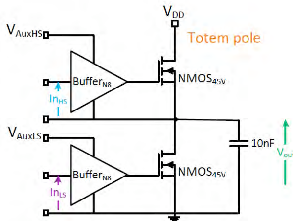
FIGURE 3.16 – Configuration Totempole
