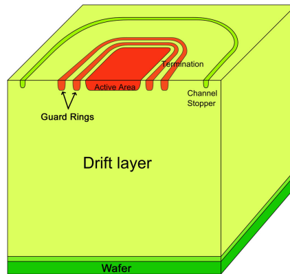
FIGURE 2.6 – Guard rings on vertical PiN Diode termination
