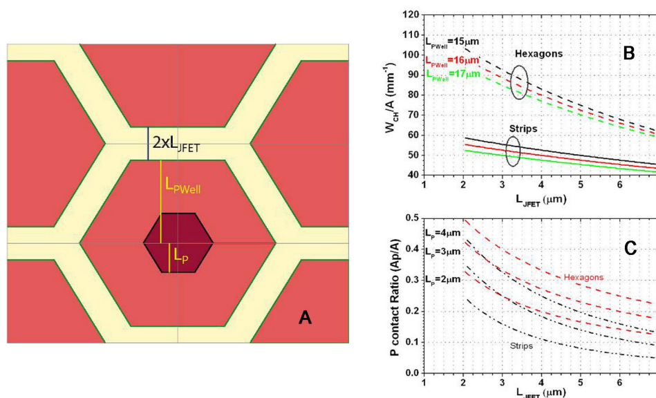
FIGURE 4.2 – Top view of an hexagonal cell (A) and comparison of the channel integration factor (B) and source contact integration factor (C) between hexagonal and stripped designs as a function of the JFET area length for different cell's design parameters
