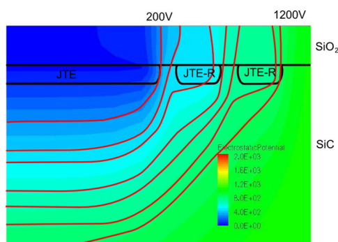
FIGURE 2.18 – Simulated potential on the JTE with JTE Rings at 1200 V
