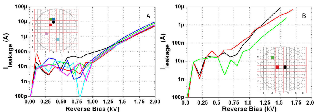
FIGURE 3.5 – Reverse characteristics of the first class (A) and second class (B) of 19\text{mm}^2 diodes from ALS5
