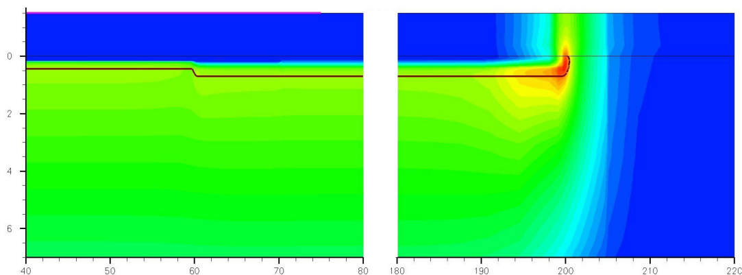
FIGURE 2.17 – Simulated electric field at V_{KA} = 1.2 \text{ kV} in a simple JTE termination implanted with a dose of 1.3 \cdot 10^{13} \text{ cm}^{-2} on a 4H-SiC PiN diode with a 12 \mu\text{m} 5 \cdot 10^{15} \text{ cm}^{-3} n-type drift layer
