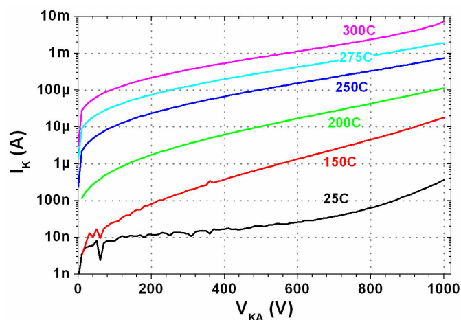
FIGURE 3.23 – Static reverse bias characteristics JBS1 diode from ALS11 at different temperatures
