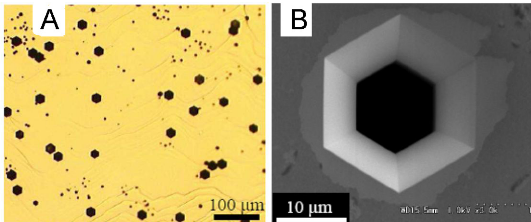
FIGURE 1.24 – Pictures of a TSD revealed by selective chemical etching taken with (a) optical microscope and (b) SEM after chlorine thermal etching during 30min at 980^{\circ}C , pictures from [12]
