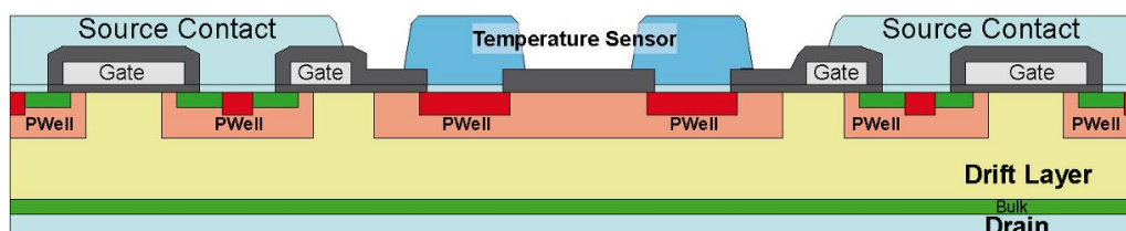
FIGURE 4.30 – Integrated Temperature Sensor within VMOS structure
