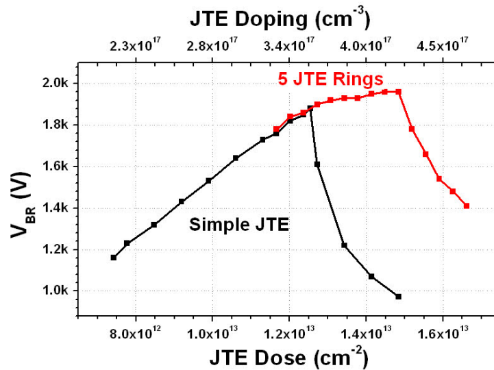
FIGURE 2.20 – Breakdown voltage as a function of JTE dose for a PiN Diode with a 12 \mu\text{m} 2 \cdot 10^{15} \text{ cm}^{-3} n-type drift layer with a simple JTE (black) and JTE Rings (red)
