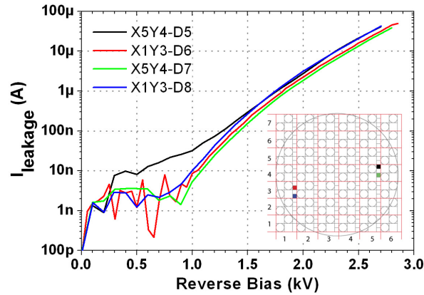
FIGURE 3.6 – Reverse capability of small diodes (2.48 mm 2 ) on ALS5
