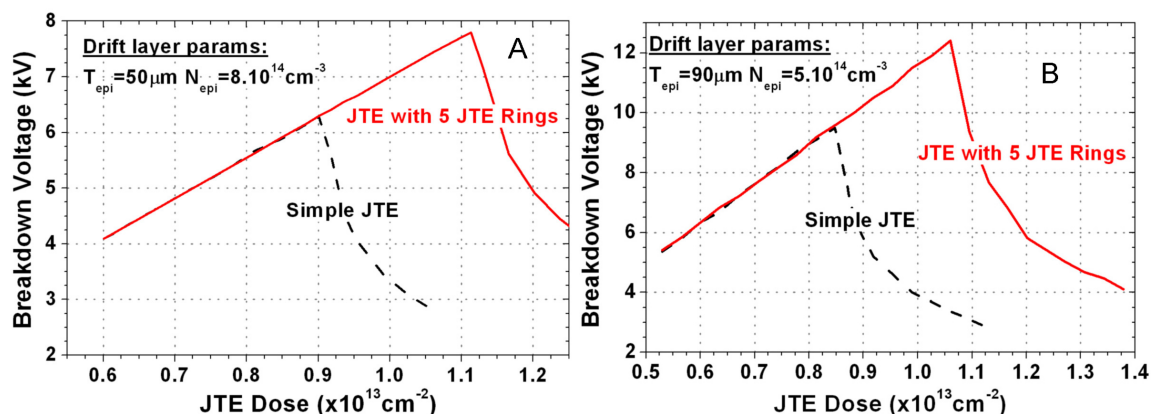
FIGURE 2.21 – Breakdown voltage as a function of the JTE dose for two different drift layer parameters with a simple JTE and 5 JTE Rings
