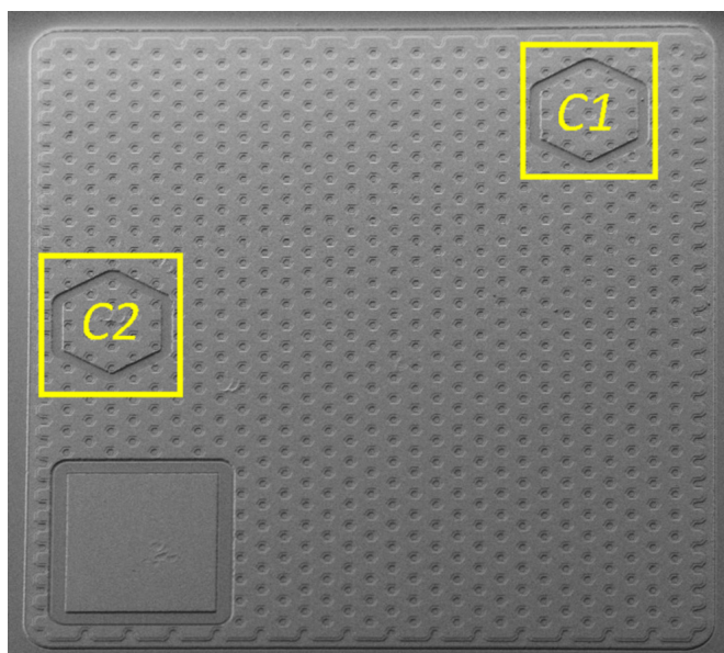
FIGURE 4.35 – SEM picture of VMOS with two current sensors
