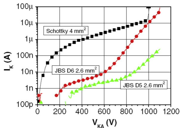
FIGURE 1.9 – Reverse characteristics of 1.2kV 4H-SiC Schottky and JBS diodes, picture from [4]
