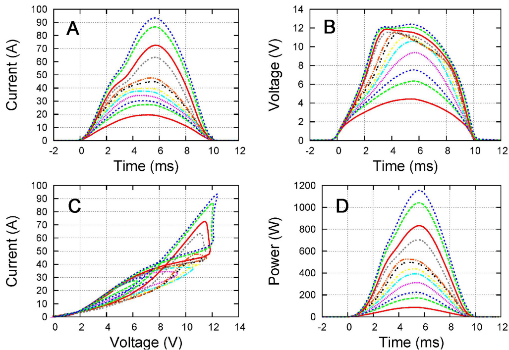
FIGURE 3.36 – Surge current tests on a JBS1 Diode from ALS11
