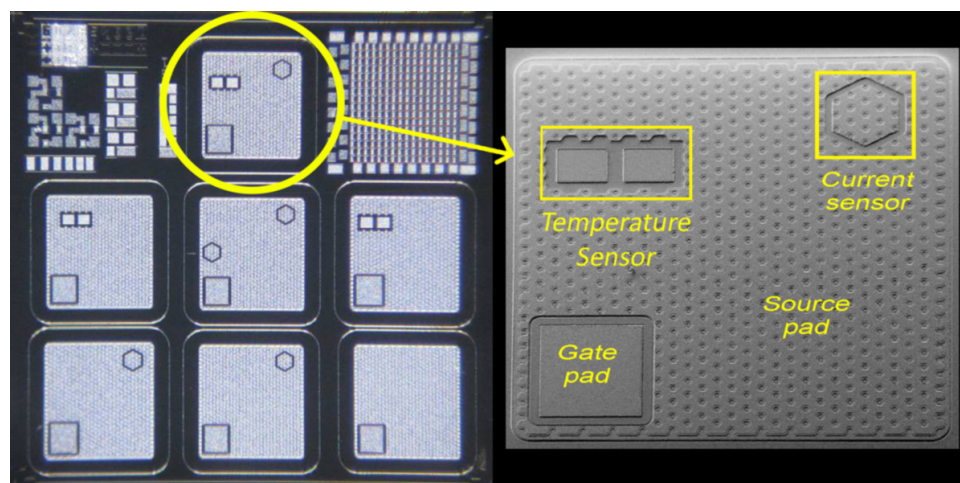
FIGURE 4.29 – SEM picture of VMOS with a temperature and a current sensors and optical photography of the Area 6 after fabrication
