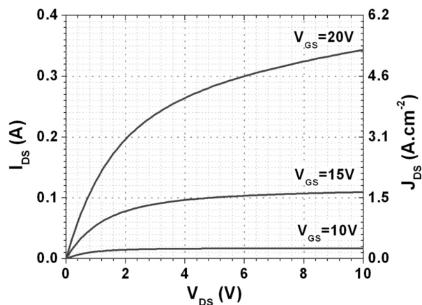
FIGURE 4.10 – I-V curve of a 6.5\text{mm}^2 MOSFET of the third generation
