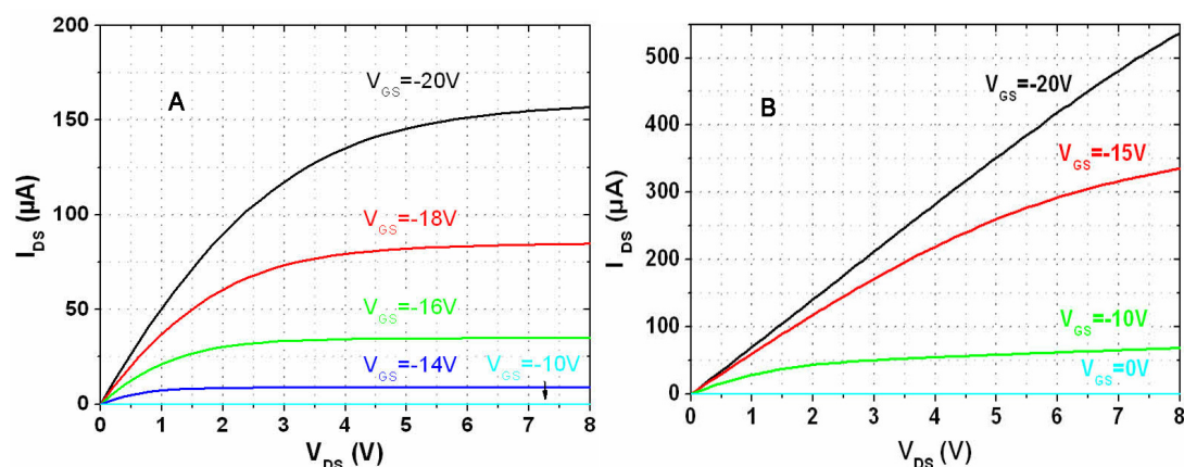
FIGURE 4.42 – I-V characteristics of the lateral PMOS on ALS7 (a) and on ALS8 (b) at different gate biases
