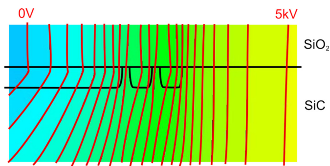
FIGURE 2.22 – Equipotential lines in termination with two JTE Rings on a 6 kV diode reverse biased at 5 kV
