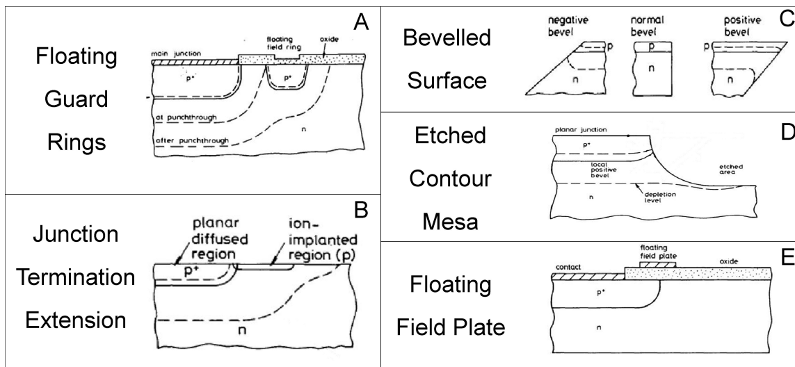
FIGURE 2.2 – Terminations used on High voltage Silicon devices
