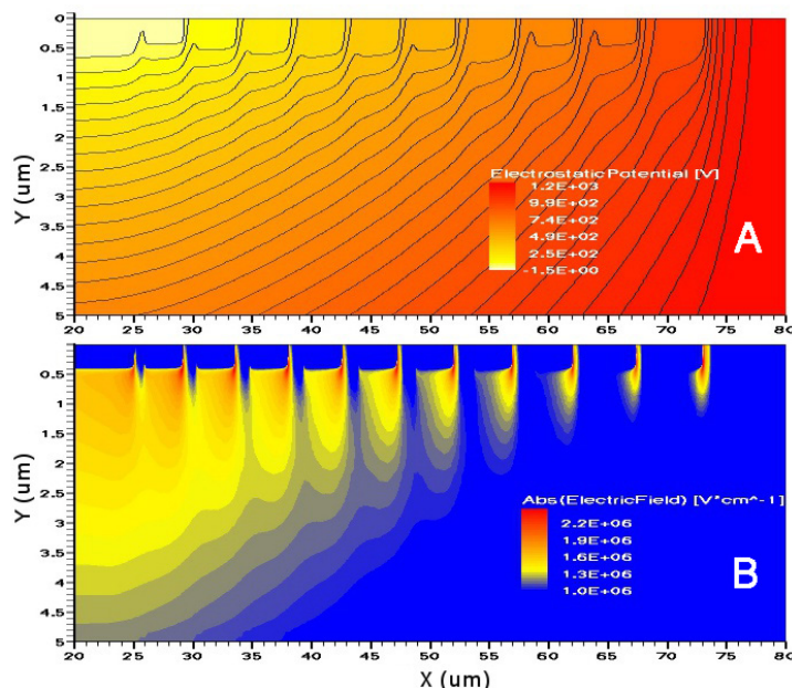
FIGURE 2.9 – Simulated potential (a) and electric field (b) in a guard ring termination at 1.2 kV for a vertical 4H-SiC PiN diode with a n-type drift layer of 12\mu\text{m } 2\cdot 10^{15}\text{cm}^{-3}
