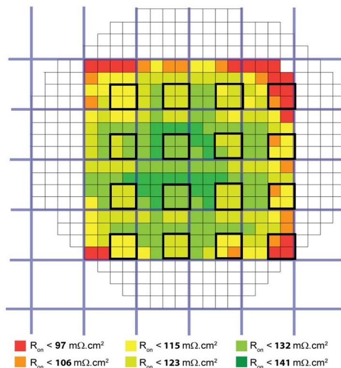
FIGURE 3.18 – mapping of the \rho_{sp} on MAX7, the areas containing the JBS diodes with a honeycomb design are surrounded by a black square
