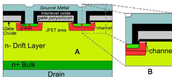
FIGURE 4.5 – Vertical cut of the VDMOS cell structure (A) with an etching step between the source and the channel seen on ESCAPEE wafers and zoom in the channel region (B)
