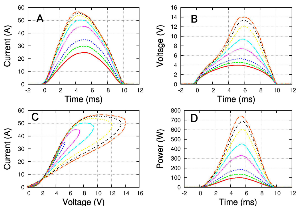
FIGURE 3.35 – 10ms Surge current tests at room temperature on a packaged Schottky diode from ALS11 wafer
