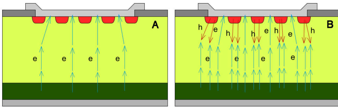
FIGURE 1.8 – Schematic view of JBS (A) and MPS (B) diodes operated at nominal current
