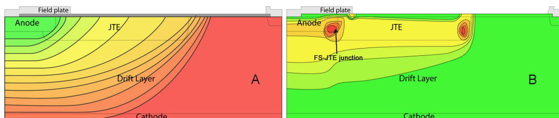
FIGURE 2.4 – Equipotential lines (A) and Electric field (B) repartition in a vertical PiN diode with JTE Termination when reverse biased
