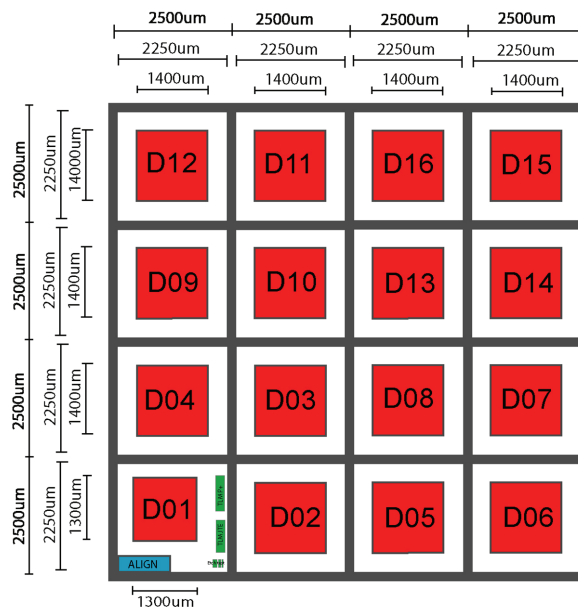
Figure 3 – basic layout used in CNM_SiC027
