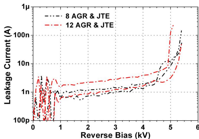
FIGURE 4.14 – Reverse characteristics of PiN diodes with JTE and AGR termination
