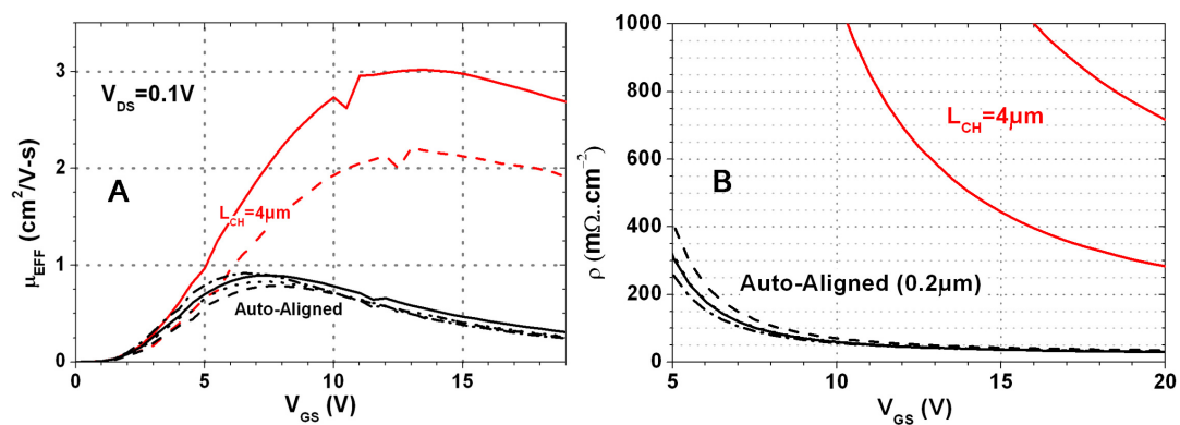
FIGURE 4.21 – Mobility (a) and Resistance (b) of multiple stripped channel VDMOS with self-aligned channel on PHL5
