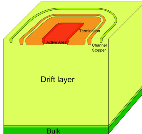
FIGURE 2.16 – JTE Rings termination structure
