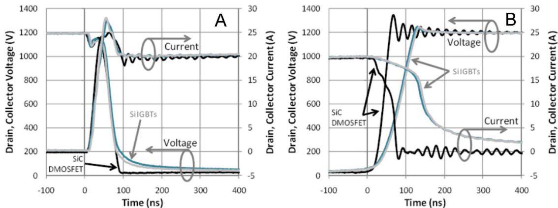
FIGURE 1.19 – Turn-on (A) and turn-off (B) waveform at 100^{\circ}\text{C} of a 20A, 1.7kV 4H-SiC VMOS ( V_{GS} = 20\text{V} ) compared to 16A and 32A, 1.7kV IGBTs ( V_{GS} = 15\text{V} ) in a clamped inductive load circuit with 4H-SiC JBS diode as freewheeling diode, graphs from [9]
