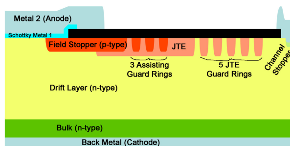
FIGURE 3.39 – Schematic view of the Schottky diodes' vertical structure and termination on CNM_SiC027
