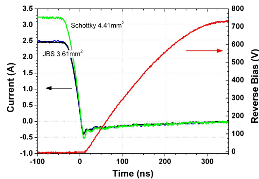
FIGURE 3.31 – reverse recovery waveforms of 6kV SiC diodes
