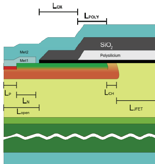
Figure 4 - Vertical cut of the VDMOS Cell
