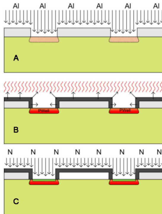
FIGURE 4.18 – Self-aligned source and p-well implantation on the VDMOS
