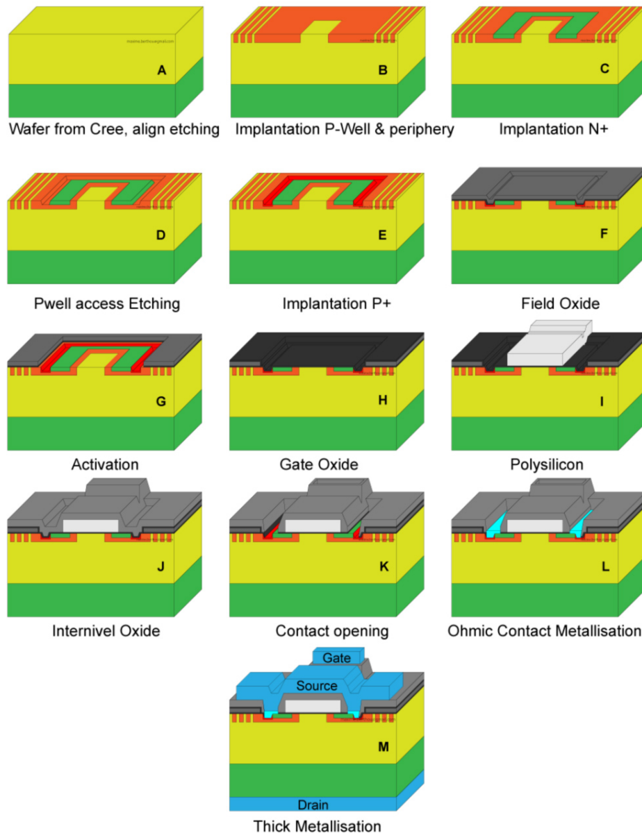
FIGURE 4.3 – Major steps of the SiC VDMOS fabrication process
