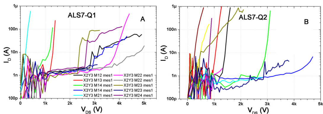
FIGURE 4.15 – Reverse characteristics of VDMOS on ALS7, Quarter 1 (A) and Quarter 2 (B)
