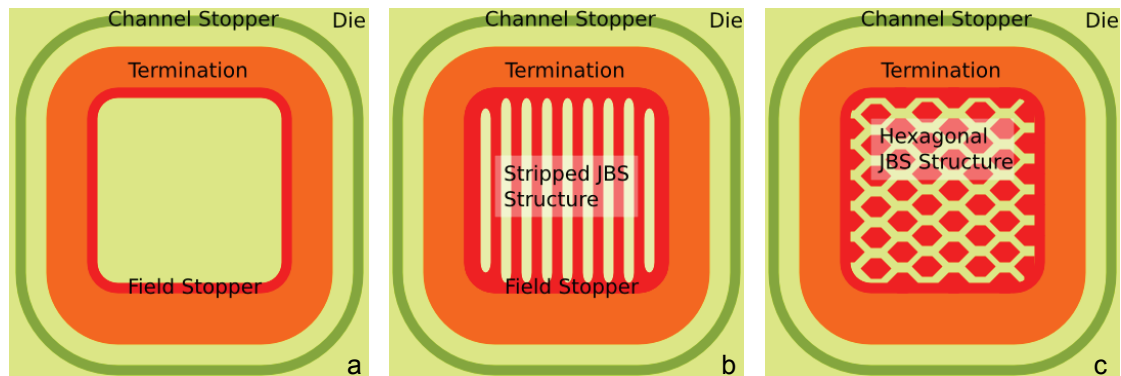
Figure 2 – Schematic top view of (a) a Schottky with field stop, (b) a stripped JBS and (c) an hexagonal JBS implemented in the various versions of CNM_SIC026 mask set
