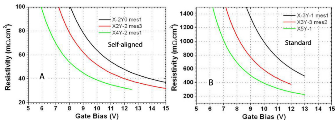
FIGURE 4.26 – Resistivity of standard channel (B) and self-aligned (A) vertical MOSFETs of 14\text{mm}^2
