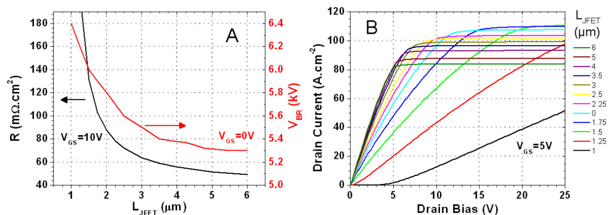
FIGURE 2.29 – JFET Area length influence on reverse and forward characteristics of the VIEMOS
