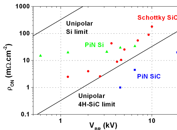
FIGURE 1.3 – Position of the state of the art SiC power diodes on the \rho_{ON} vs V_{BR} graph
