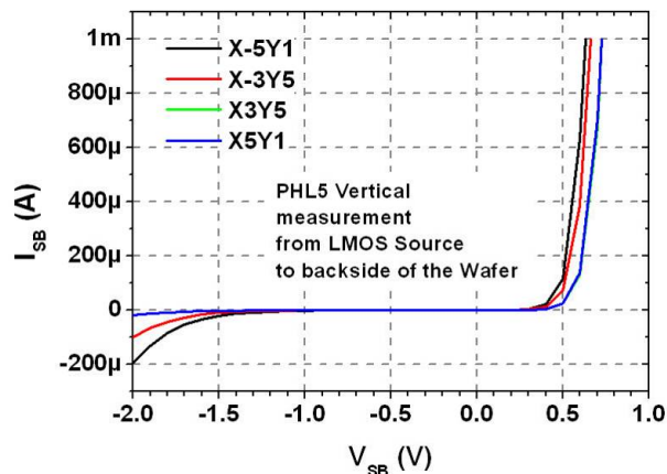
FIGURE 4.11 – Drain to source leakage current on LMOS of PHL5
