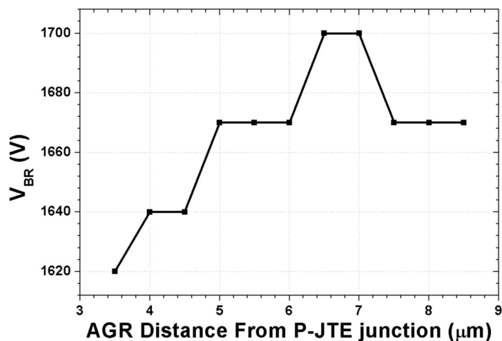
FIGURE 2.15 – Breakdown voltage as a function of the Assisting Ring distance from the FS-JTE junction
