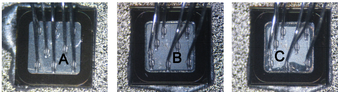
FIGURE 3.37 – Pictures of the Schottky diodes (a) before and (b,c) after failure during surge current tests
