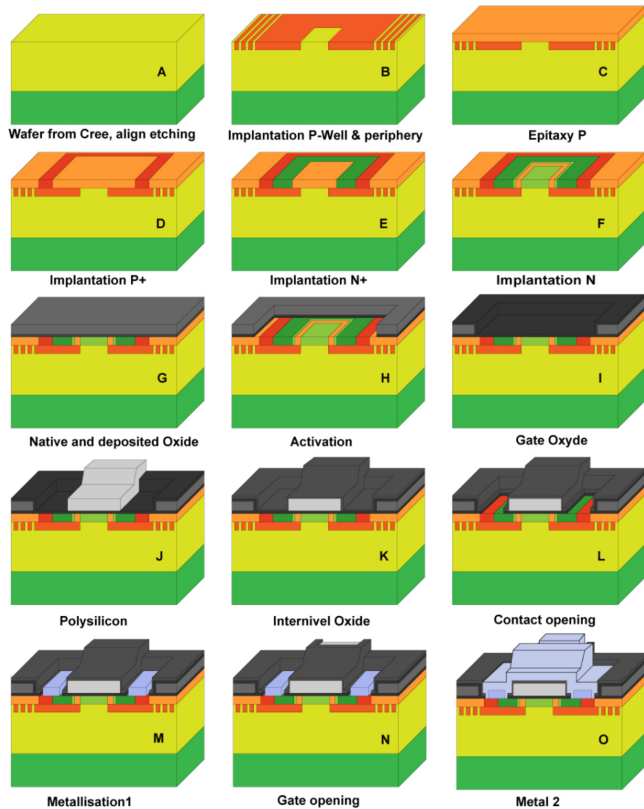
FIGURE 4.38 – Major VIEMOS fabrication process steps
