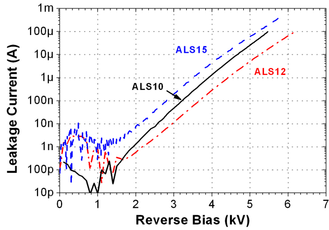
FIGURE 3.14 – Typical reverse characteristics of Schottky diodes on ALS10, ALS12 and ALS15
