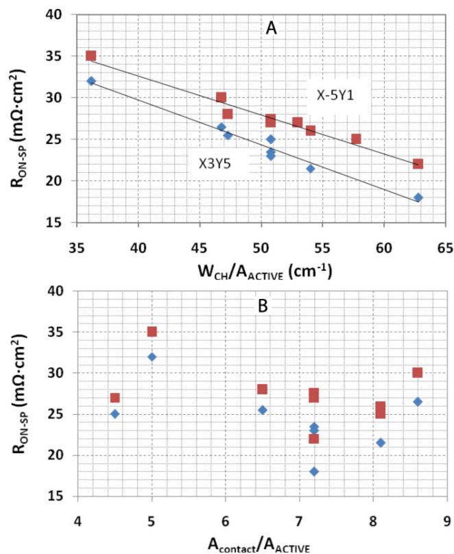
FIGURE 4.23 – Resistivity of VMOS with self-aligned channel as a function of the channel width to active area ratio (a) and contact to active area ratio (b), the squares represent devices in the situated on the left side (X-5Y1) of the wafer and the losanges represent devices on the right side (X3Y5) of the wafer
