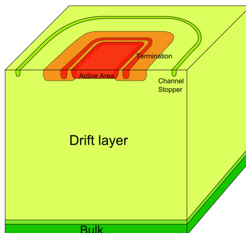
FIGURE 2.12 – PiN Diode with a JTE and an Assisting Guard Ring implanted with the anode implantation level
