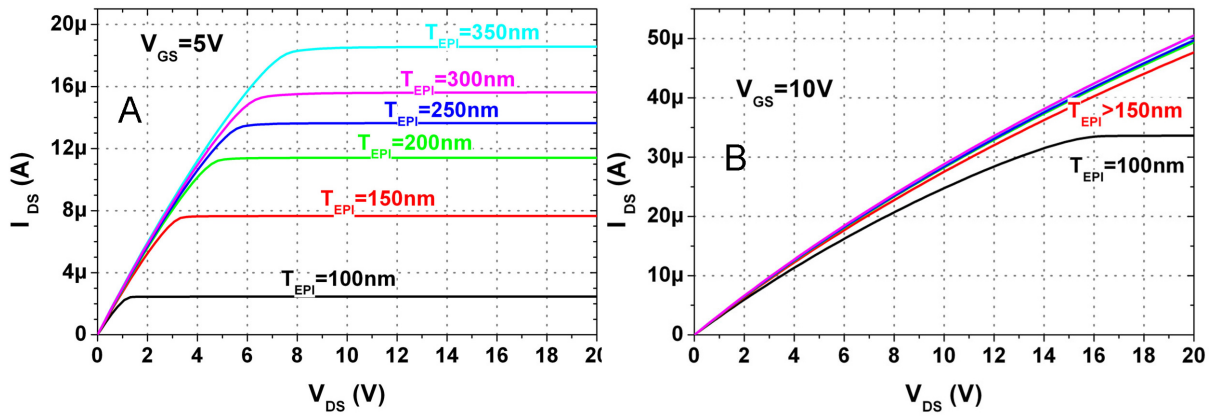
FIGURE 2.26 – Forward characteristics of VIEMOS for different P-type epitaxial layer thickness
