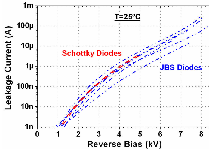
FIGURE 3.24 – Reverse characteristics of the diodes on MAX7 at room temperature under vacuum
