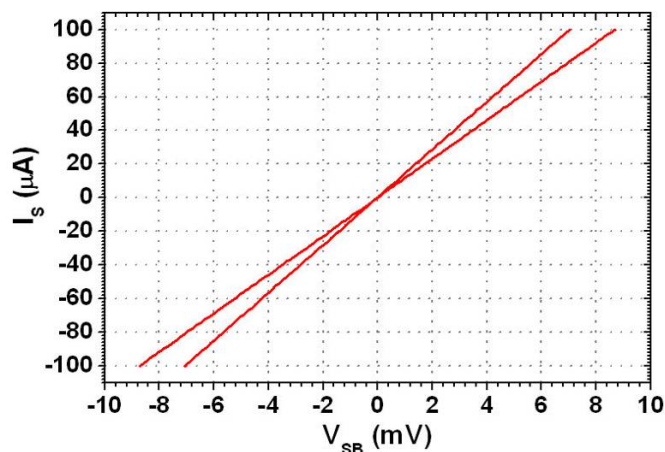
FIGURE 4.39 – Vertical leakage current from Source of a lateral MOS to the bulk at different positions on the wafer
