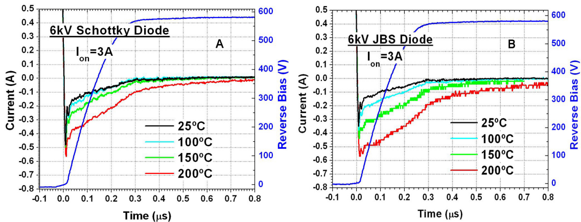
FIGURE 3.32 – Reverse recovery of the Schottky (A) and JBS (B) diodes at different temperatures
