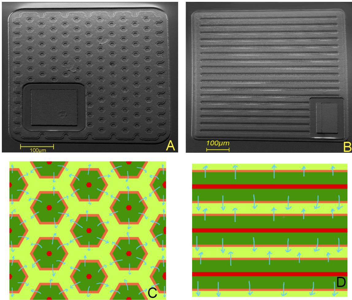
FIGURE 1.15 – Different geometries of VMOS channel fabricated at CNM; (A) SEM picture of a VMOS with hexagonal cells, which doping structure is shown in (C) with red to represent the p-type impurities and green for the n-type. A SEM picture of VMOS with striped channel is shown in (B), the doping structure is represented in (D)
