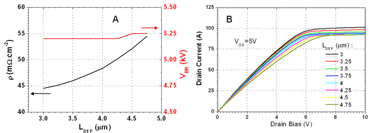
FIGURE 2.31 – P-well overlap dimensions influence on MOSFETs reverse and forward characteristics
