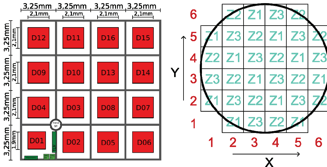
Figure 1 – (a) Basic field with 16 different diodes and (b) fields variation distribution used in mask set CNM_SIC026
