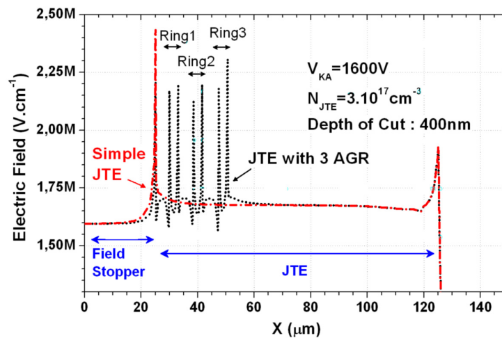
FIGURE 2.14 – Simulated Electric Field inside the termination for a JTE and a JTE with Assisting Guard Rings
