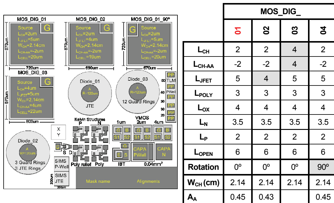
Figure 7 – Schematic layout of Area 2
