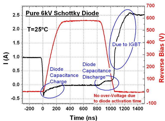
FIGURE 3.30 – full switching waveform of a 6 kV pure Schottky diode
