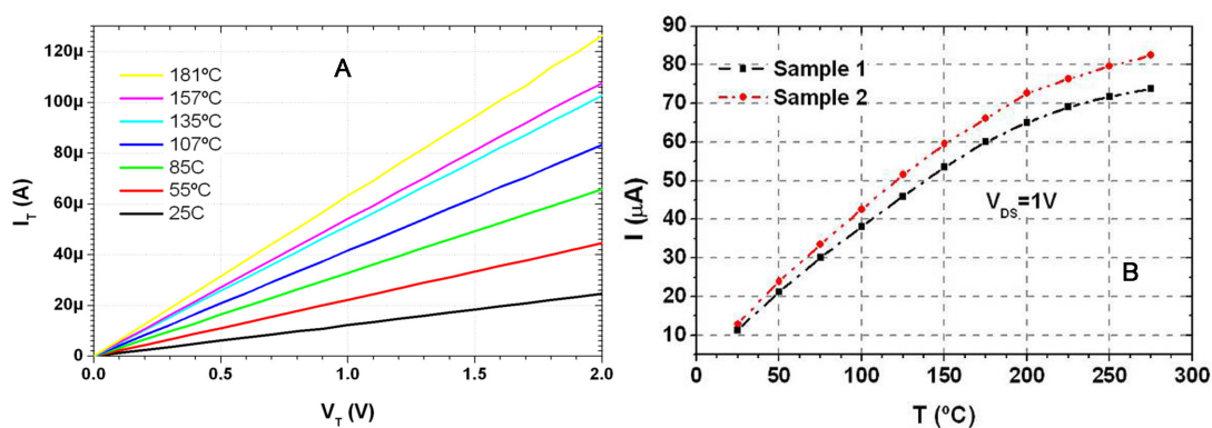
FIGURE 4.31 – Temperature sensor characteristics as a function of the temperature
