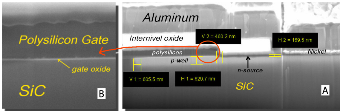
FIGURE 4.43 – SEM image of a vertical cut of a VDMOS cell on ALS7
