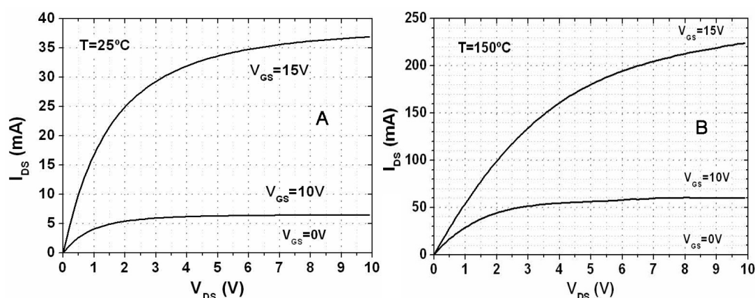
FIGURE 4.27 – I-V characteristics of a 1mm 2 4H-SiC VMOS on PHL8 at 25°C (a) and 150°C (b), and different gate biases
