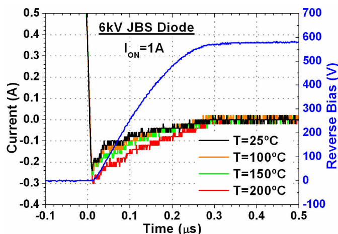
FIGURE 3.33 – Reverse recovery of the JBS diode at 1A and different temperatures
