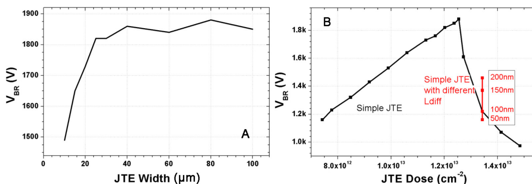
FIGURE 2.5 – Simulated Breakdown voltage as a function of the JTE length (a) and dose (b) for a 4H-SiC PiN Diode with a 12\mu\text{m} 2\cdot 10^{15}\text{cm}^{-3} N-type drift layer
