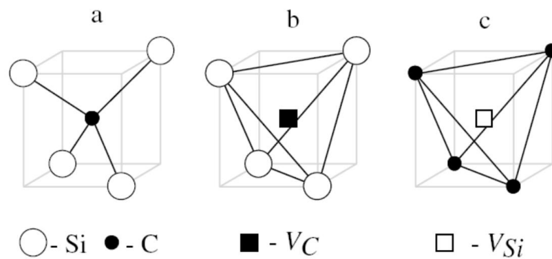
FIGURE 1.28 – Vacancies in SiC ; (a) defect free, (b) carbon Vacancy, (c) silicon vacancy. Pictures from [13]
