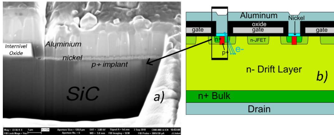
FIGURE 4.44 – FIB cut on VIEMOS structure on ALS8 (a) and schematized structure (b) created without the p-well and p-type epitaxial layer
