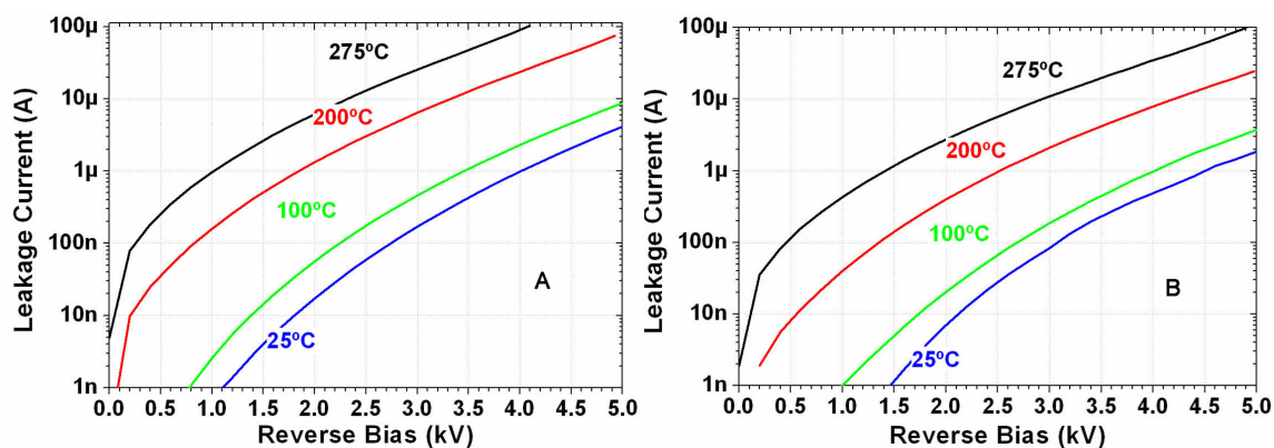
FIGURE 3.25 – Typical reverse characteristics of Schottky and JBS (Stripped 3P/4N) diodes on MAX7 at different temperatures
