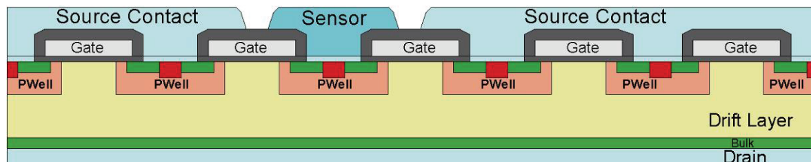
Figure 10 - Current Sensor
