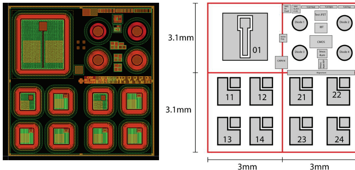
Figure 2 - VDMOS layout, screenshot of the layout on the left and schematic view on the right
