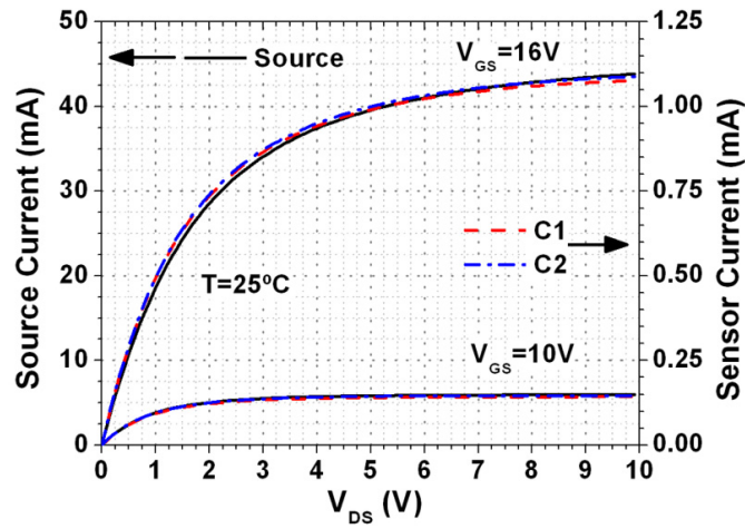
FIGURE 4.36 – Double current sensor VMOS forward characteristics
