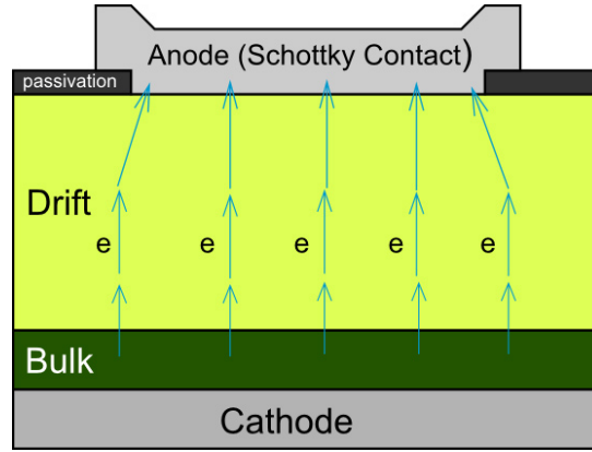
FIGURE 1.4 – Schematic view of a Schottky diode’s vertical cut
