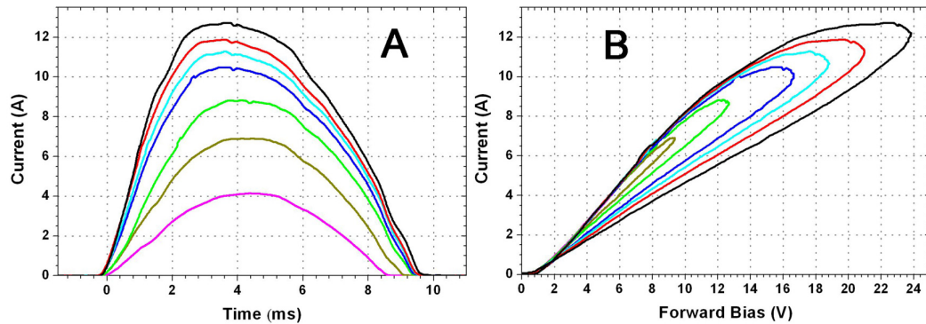
FIGURE 3.38 – Surge Current Waveforms on 6kV Schottky diodes
