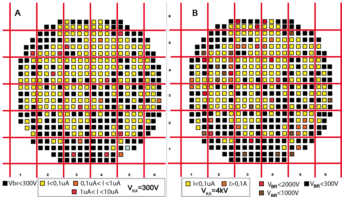
FIGURE 3.15 – ALS10 reverse current mapping at (a) 300V and (b) 4kV
