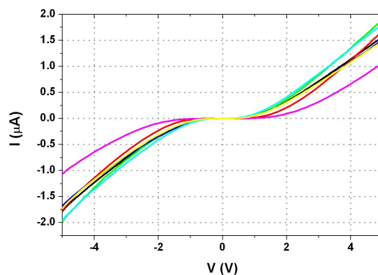
FIGURE 3.21 – TLM characteristics of W contacts on implanted p^+ at different positions of wafer ALS11
