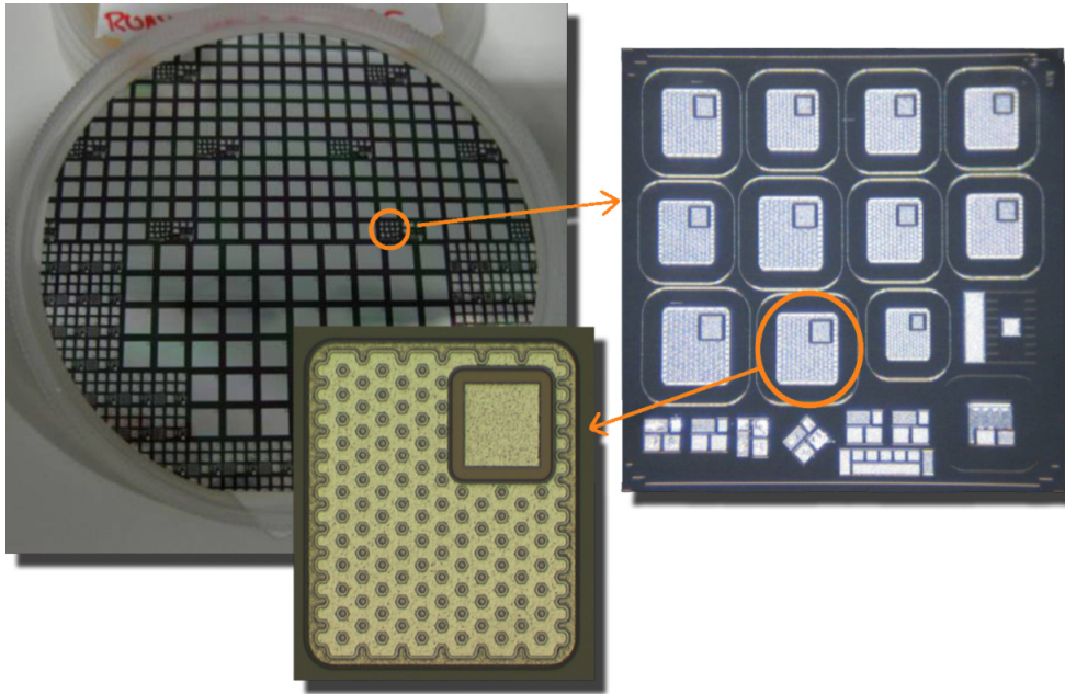
FIGURE 4.22 – Pictures of the VMOS with different cell dimensions in area 3 on PHL5
