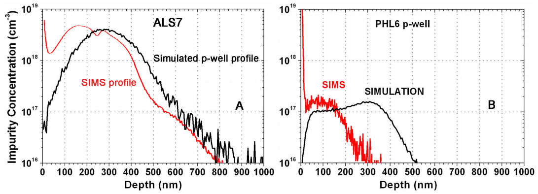
FIGURE 4.12 – SIMS measurement of the p-well profile on ALS7 (a) and PHL6 (b)
