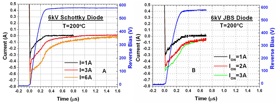
FIGURE 3.34 – Turn-off waveforms of the Schottky and JBS diodes at 200°C for different switched currents
