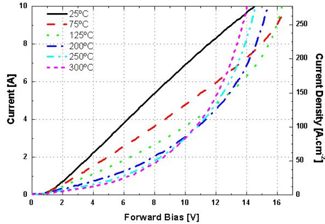
FIGURE 3.22 – Forward Bias JBS characteristics at different temperatures
