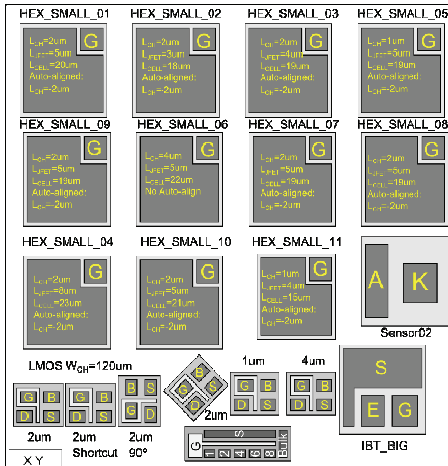
Figure 8 – Schematic Layout of Area 3
