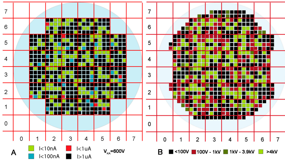
FIGURE 3.12 – (A) Preliminary leakage mapping at reverse bias of 600V and (B) blocking capability of all diodes on PHL3
