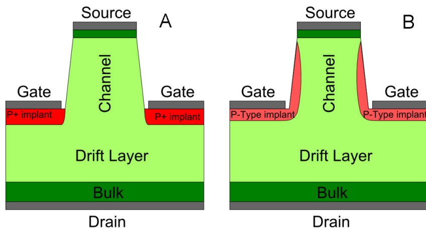
FIGURE 1.20 – Schematic view of a vertical cut through the active cell of a BG-JFET (A) and a TI-JFET (B)
