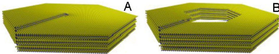
FIGURE 1.23 – Illustration of (A) a closed-core and (B) open-core screw dislocation with a Burgers vector \vec{b} = 1c in the crystal lattice of 4H-SiC, illustration from [11]
