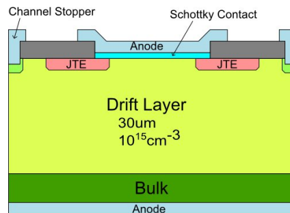
FIGURE 3.3 – Structure of the Schottky diode fabricated with the mask set CNM_SiC016
