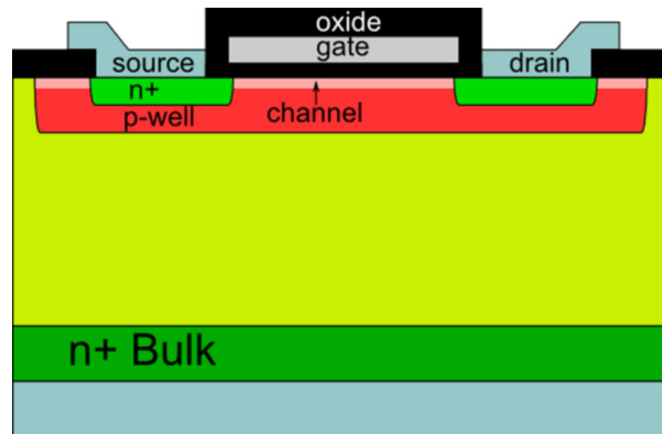
FIGURE 4.6 – implanted LDMOS test structure
