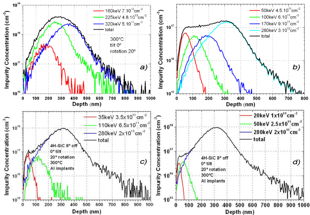
FIGURE 4.9 – Simulated p-well implantation profile used for the VDMOS process on AL8 for (a), PHL5 and PHL6 for (b), PHL7 and PHL9 for (c), and PHL8 for (d)
