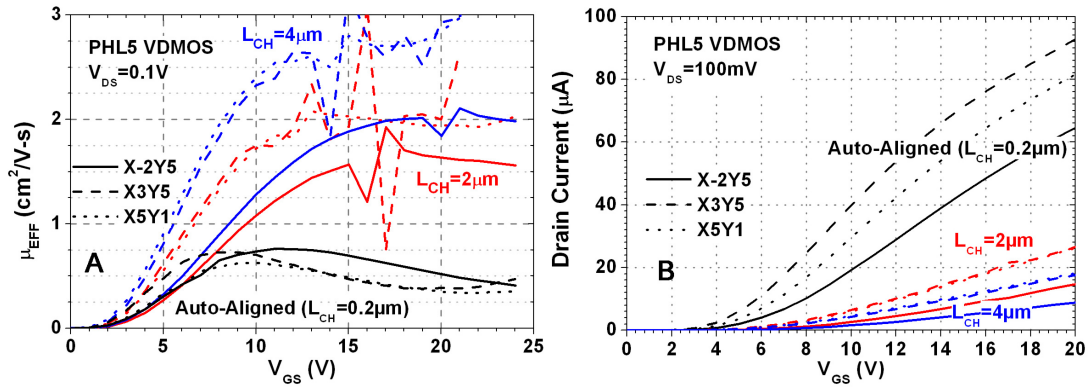
FIGURE 4.19 – Self-aligned channel characteristics compared to classical VDMOS channels on the single channel VDMOS
