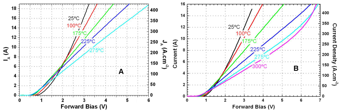
FIGURE 3.20 – Forward bias characteristics of Schottky diode (a) and JBS diode (b) at different temperatures
