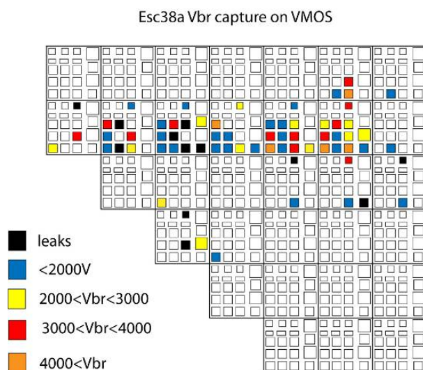
FIGURE 4.8 – Reverse bias mapping on ESC38a
