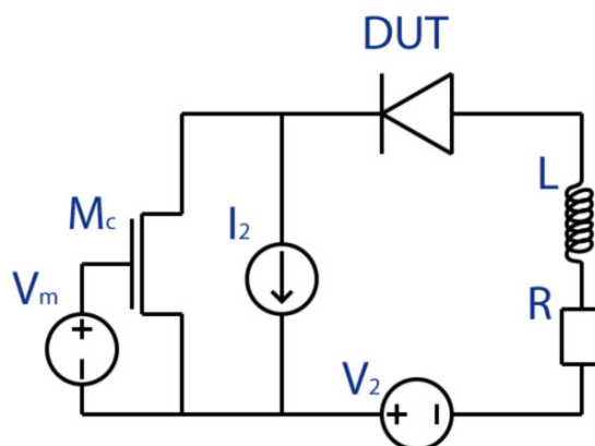
FIGURE 3.27 – Electrical schematic of the setup used to characterize the switching behaviour of the diodes
