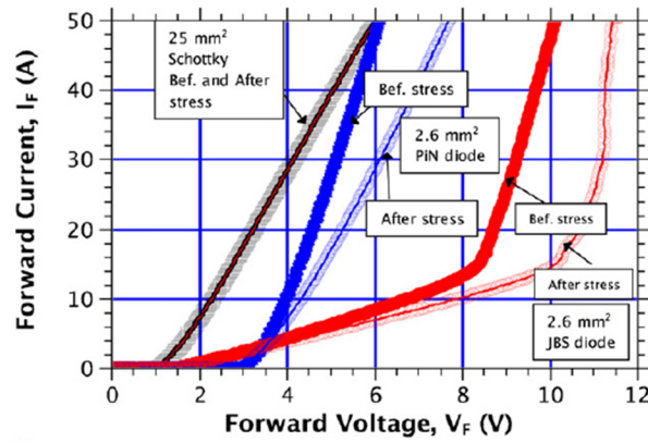
FIGURE 1.11 – Degradation of different types of 3.3kV diodes after stress, pictures from [5]
