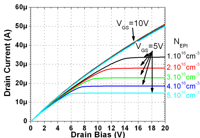
FIGURE 2.28 – forward characteristics of the VMOS simulated with different doping concentration of the thin surface p-type epitaxial layer
