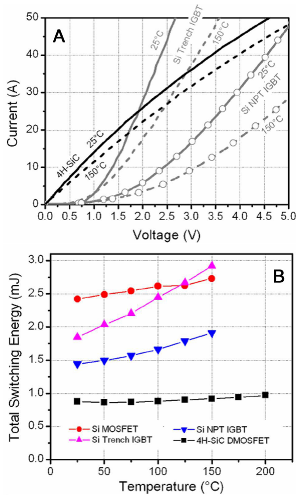
FIGURE 1.16 – Forward I-V characteristics (A) of a 1.2 kV SiC MOSFET by CREE and Si-IGBT at 25°C and 150°C. (B) Total switching energy as a function of the temperature for 20 A, 1.2 kV rated devices. Curves from [7]
