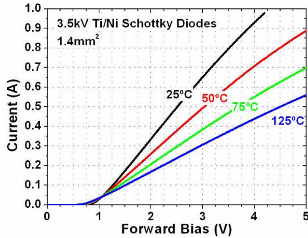
FIGURE 1.6 – Forward I-V characteristics of a 3.5kV Ti-Ni/4H-SiC Schottky diode at different temperatures
