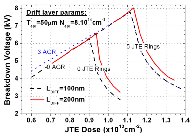
FIGURE 2.24 – Simulated breakdown voltage of different planar termination with a 4H-SiC vertical PiN diode
