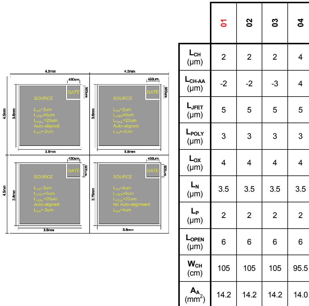
Figure 9 - Schematic View and Design parameter of VDMOS in Area 5
