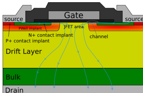
FIGURE 1.14 – Schematic view of the vertical cut of a VMOS cell
