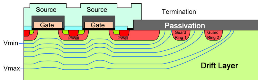
FIGURE 2.7 – Guard rings on VMOS structure
