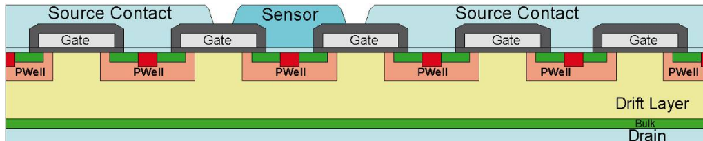
FIGURE 4.32 – Vertical cross section of the integrated Current Sensor within the VMOS structure
