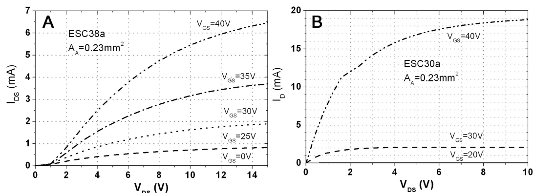
FIGURE 4.7 – Kellog's network for same device with a channel length of 3\mu\text{m} (MV03) on wafer ESC38a and ESC30a
