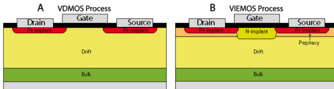
FIGURE 4.40 – Schematic view of the PMOS structure fabricated with the layout CNM.SiC025, for the VDMOS process used on ALS7 (a) and the VIEMOS process (b) used on ALS8
