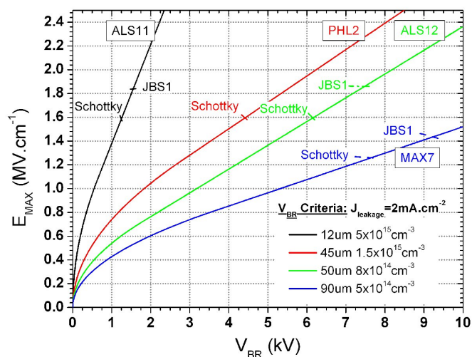
FIGURE 3.41 – Representation of E_{max} as a function of V_{BR} (lines) for the different epitaxial layer parameters employed for the diodes fabricated during this work and situation of these diodes
