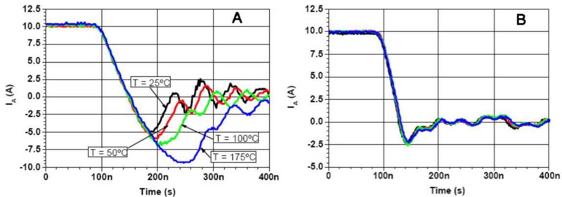
FIGURE 1.7 – Turn-off current waveforms of (a) a 1.2kV Si-PiN diode (A) and a 1.2kV SiC Schottky diode (B) at different temperatures, pictures from [3]
