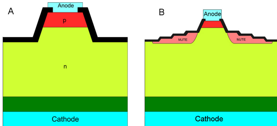
FIGURE 2.11 – mesa (a) and modified JTE (b) structures
