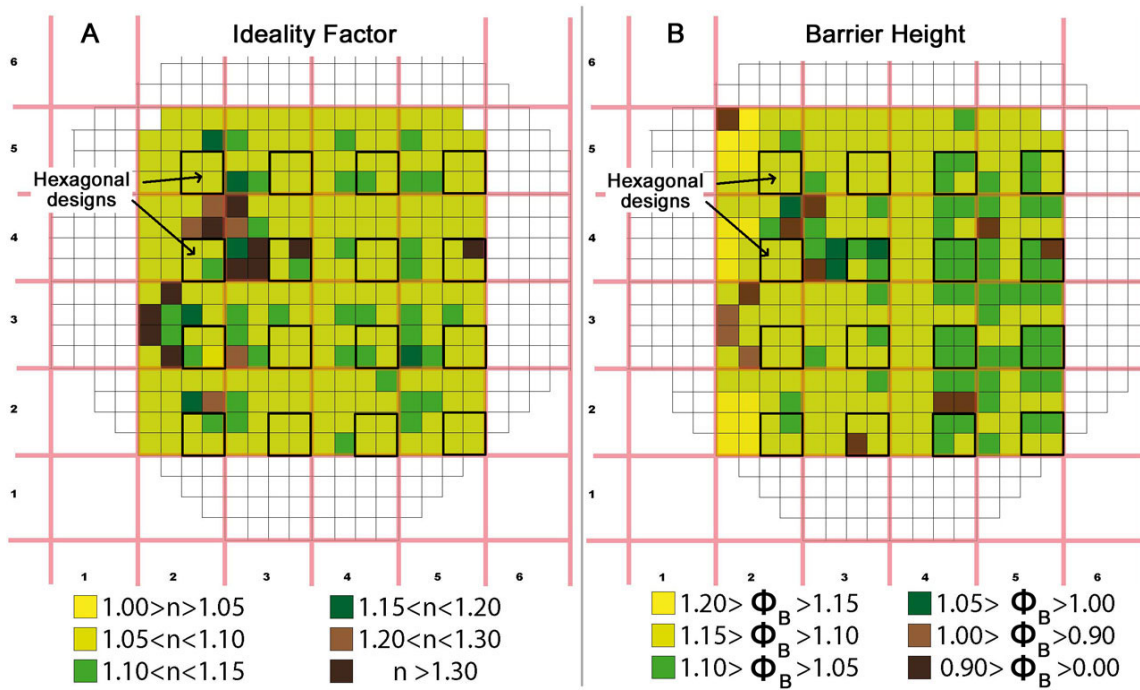
FIGURE 3.17 – mapping of the ideality factor (A) and barrier height of the Schottky contacts on MAX7, the areas containing the JBS diodes with a honeycomb (Hexagonal) designs are surrounded by a black square
