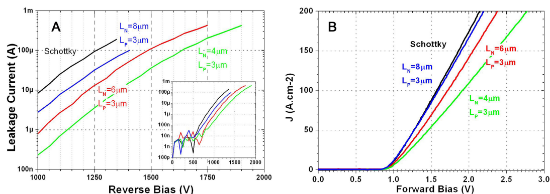
FIGURE 3.9 – Reverse (A) and forward (B) characteristics of JBS and Schottky diodes on ALS11 wafer
