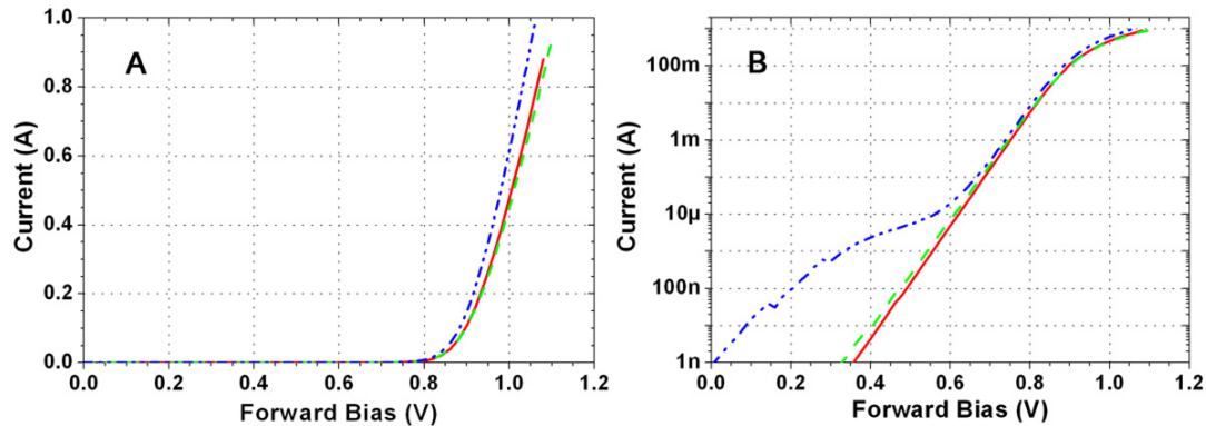
FIGURE 3.7 – Forward characteristics of Schottky diodes on ALS11 represented on (A) linear scale and (B) logarithmic scale
