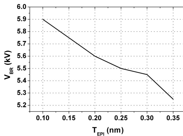
FIGURE 2.27 – Breakdown characteristics of the active area of the VIEMOS for different P-type epitaxial layer thickness
