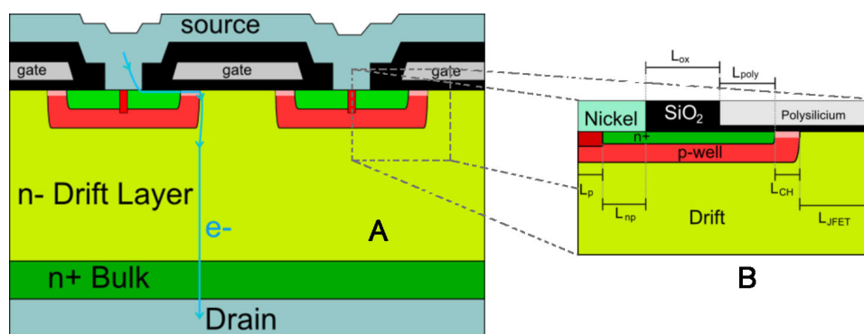
FIGURE 4.1 – Vertical cross section of a simplified VDMOS cell (A) and zoom in the channel region (B); the n-type areas are represented in green and the p-type ones are colored in red
