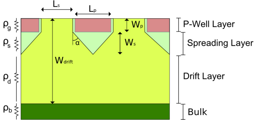
FIGURE 1.10 – Schematic view of a JBS diode' vertical cut in its active region with the equivalent resistances of the different regions
