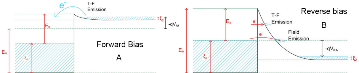
FIGURE 1.5 – Electronic structure of a Schottky contact on n-type semiconductor when forward biased (A) and reverse biased (B)
