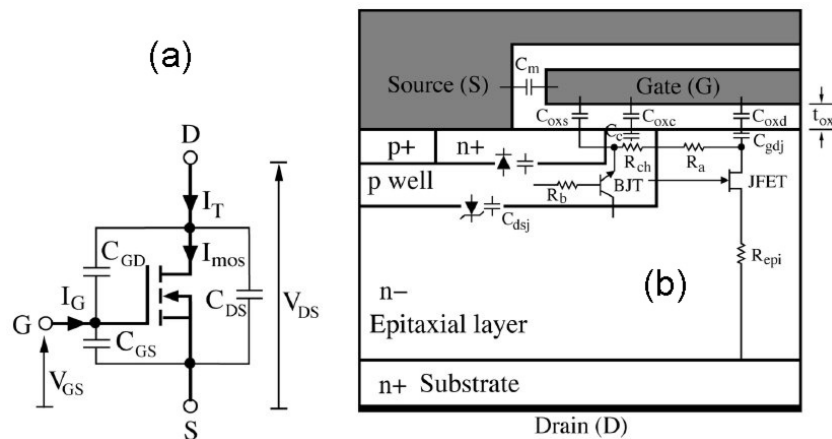
FIGURE 1.17 – (a) Equivalent capacitance between terminal of a VMOS, (b) cross section and associated parasitic components of the VMOS. Pictures from [8]
