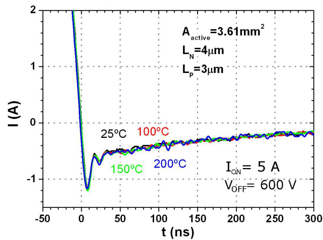
FIGURE 3.29 – Reverse Recovery Current of a 4H-SiC JBS Diode from ALS11 at different temperatures
