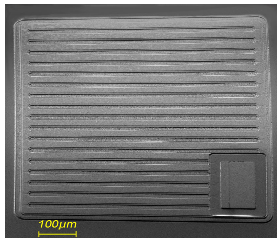
FIGURE 4.20 – 0.25mm 2 VDMOS with multiple stripped channels
