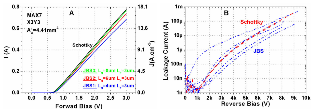
FIGURE 3.16 – (A) Forward and (B) reverse characteristics of Schottky and JBS diodes fabricated on MAX7
