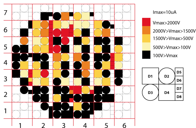
FIGURE 3.4 – Reverse leakage current mapping of wafer ALS5
