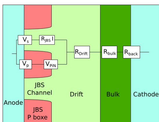
FIGURE 3.19 – Equivalent resistances in the JBS diode
