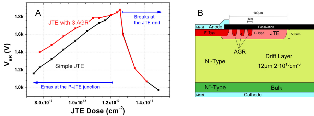
FIGURE 2.13 – (a) Simulated breakdown voltage of a PiN diode with a JTE or a JTE with 3 AGR for different JTE doping concentrations and (b) schematic view of the PiN diode with a JTE and 3 AGR
