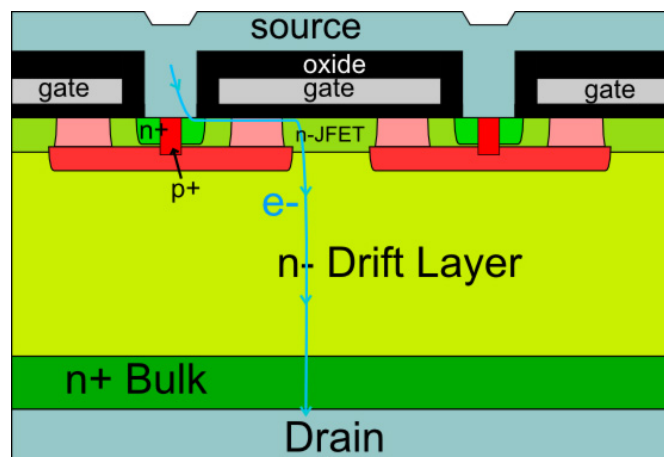
FIGURE 4.37 – Schematic view of the VIEMOS structure
