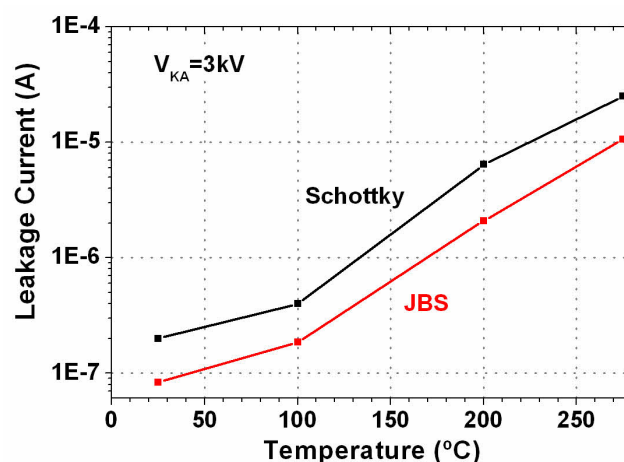
FIGURE 3.26 – Extracted leakage current dependence with temperature at 3kV
