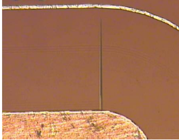
FIGURE 1.27 – Inverted pyramid defect in the termination of a vertical power diode
