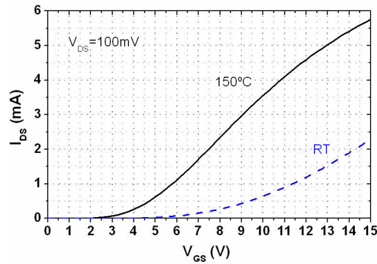
FIGURE 4.28 – Transconductance characteristics at V_{DS}=100\text{mV} for the same VMOS device at room temperature and 150^\circ\text{C}
