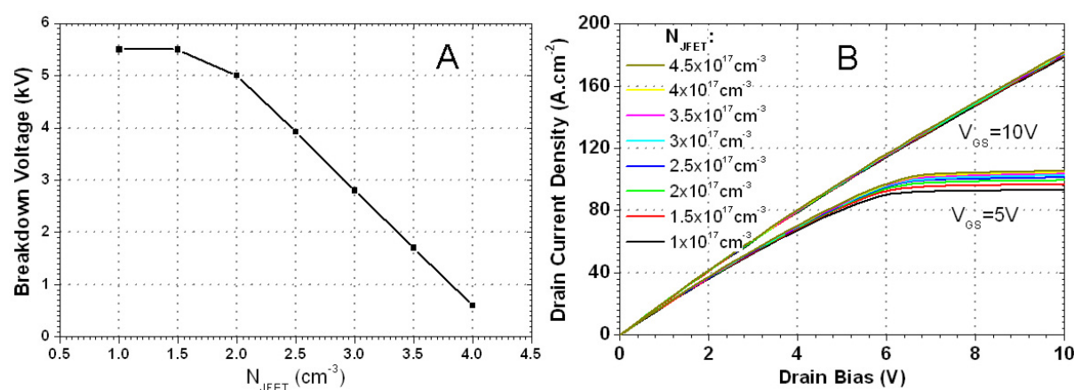
FIGURE 2.30 – JFET doping concentration influence on reverse (a) and forward (b) characteristics
