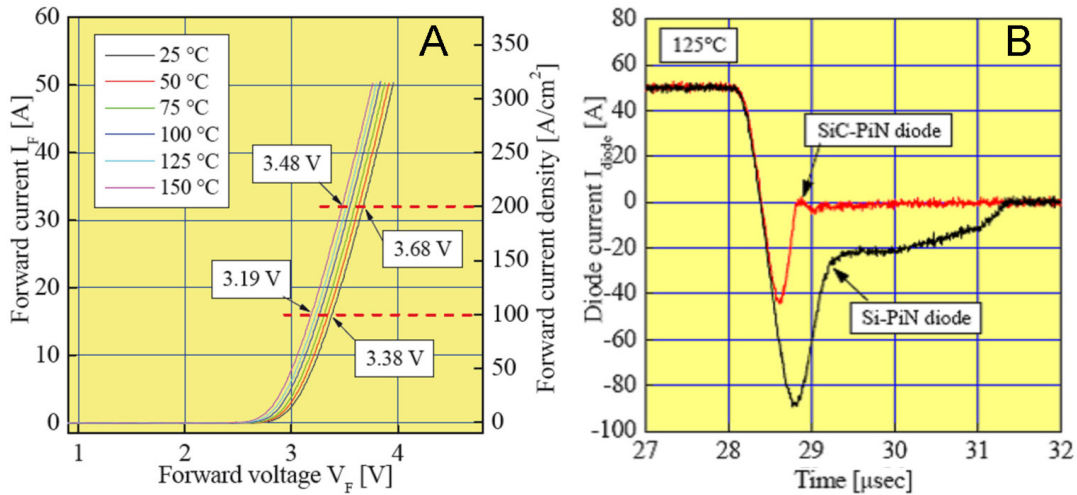
FIGURE 1.12 – (a) Forward I-V characteristics from room temperature up to 150°C of a 6kV 4H-SiC PiN diode and (b) turn-off current waveform at 125°C for the same diode, showing a recovery charge of 11 \mu C, compared to a 6kV Si-PiN diode, showing a recovery charge of 83 \mu C, pictures from [6]
