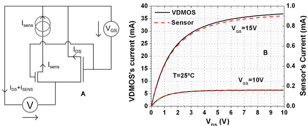
FIGURE 4.33 – Measurement configuration used to characterize the sensor and VMOS (a) and I-V curve measured at 25°C (b)
