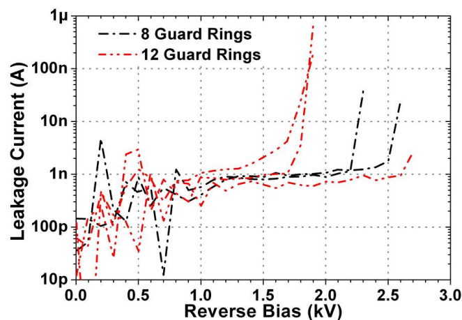
FIGURE 4.13 – Reverse characteristics of PiN diode with guard rings fabricated on ALS7
