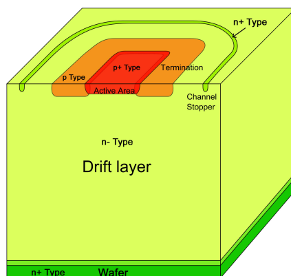
FIGURE 2.3 – Schematic view of the a PiN diode with a JTE termination
