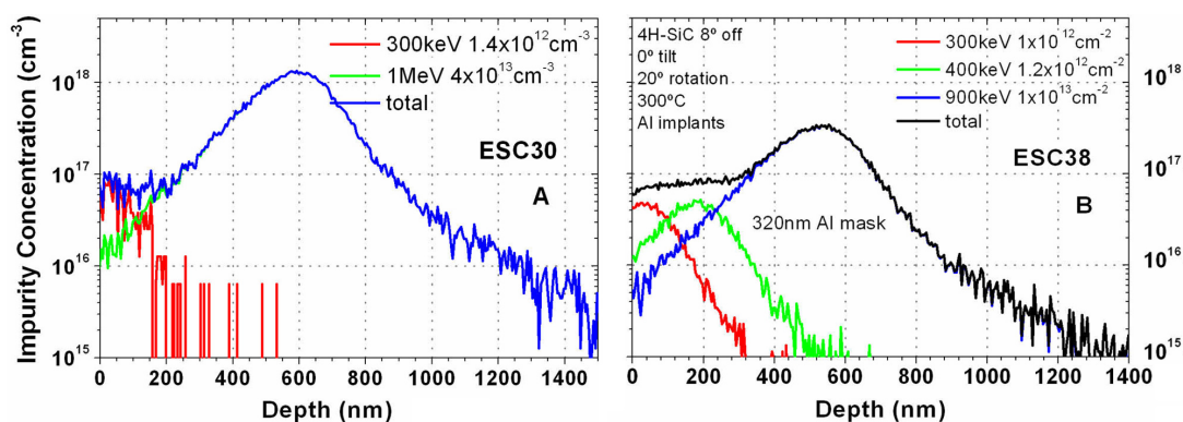
FIGURE 4.4 – Simulated implanted doping profile of the p-well on ESC30 (a) and ESC38 (b)
