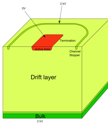
FIGURE 2.1 – Representation of vertical chip when reverse biased at 2kV
