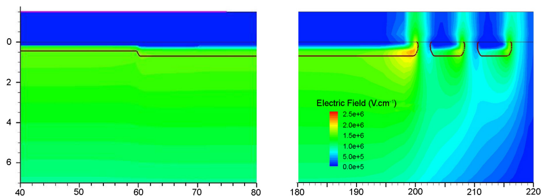
FIGURE 2.19 – Simulated electric field at V_{KA} = 1.2\text{kV} in a termination with JTE and JTE Rings implanted with at 1.3 \cdot 10^{13}\text{cm}^{-2} on a 4H-SiC PiN diode with a 12 \mu\text{m} 2 \cdot 10^{15}\text{cm}^{-3} n-type drift layer
