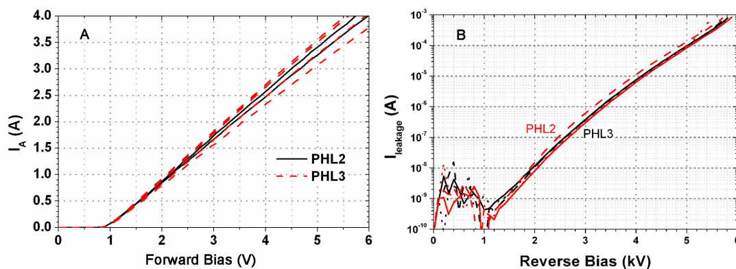
FIGURE 3.11 – (A) Forward and (B) reverse characteristics of Schottky diodes on PHL2 and PHL3 wafers
