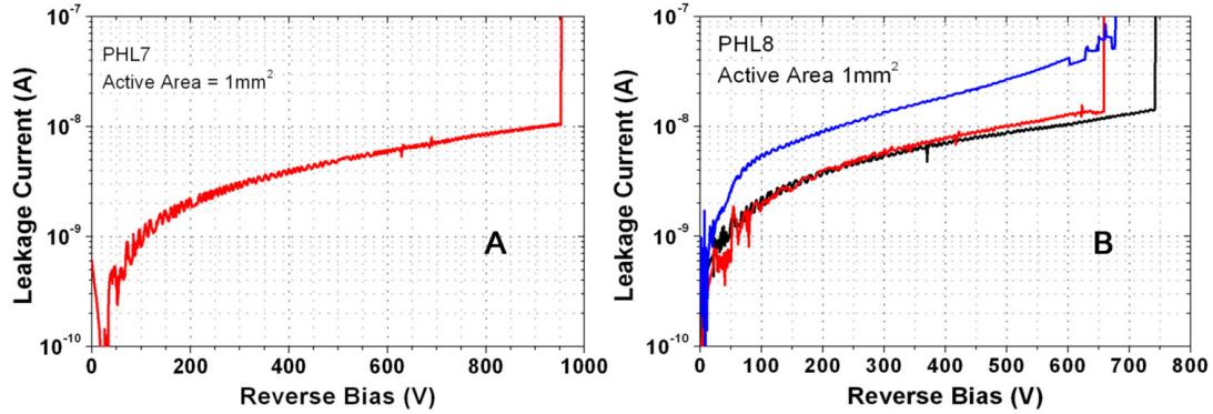
FIGURE 4.16 – Typical reverse characteristics of VMOS on PHL7 and PHL8
