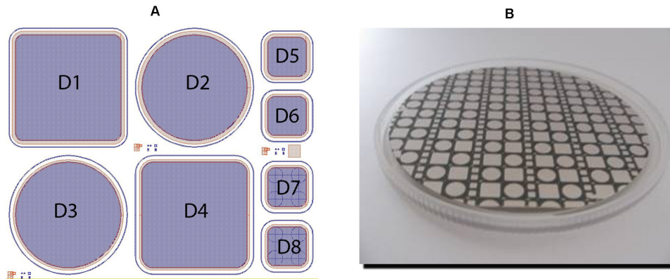
FIGURE 3.2 – Basic field (a) of the layout CNM_SIC016 used on ALS5 wafer (b)
