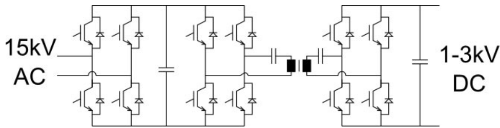
FIGURE 1.2 – Electronic schematic of a high voltage solid-state converter for railways application [2]
