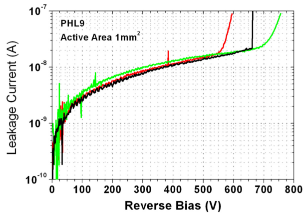
FIGURE 4.17 – Reverse characteristics of VMOS devices on PHL9
