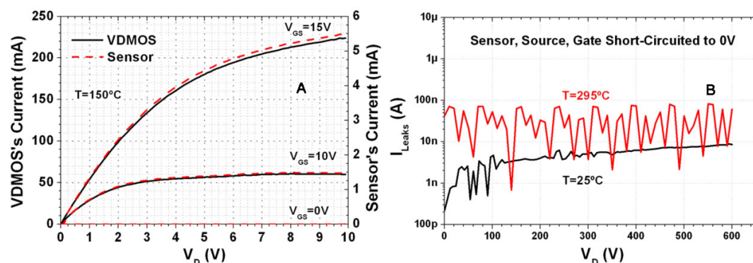
FIGURE 4.34 – VMOS and its Current sensor (a) forward characteristics at 150°C and (b) reverse characteristics up to 600V at room temperature and 295°C with source, sensor and gate shortcut
