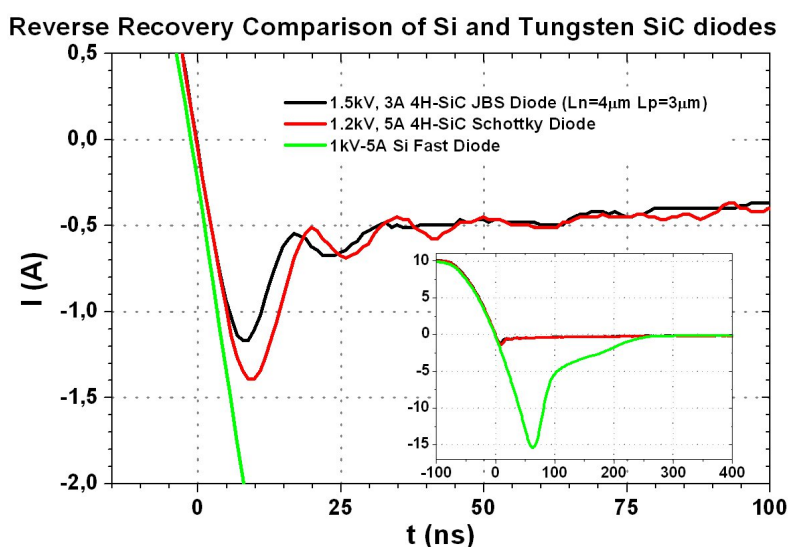
FIGURE 3.28 – Comparison of JBS1 and Schottky diodes from ALS11 with a 1kV fast recovery Si Diode
