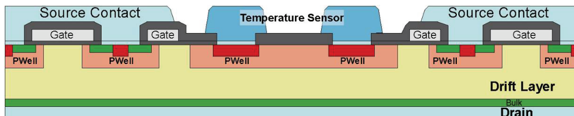
Figure 11 - Temperature Sensor
