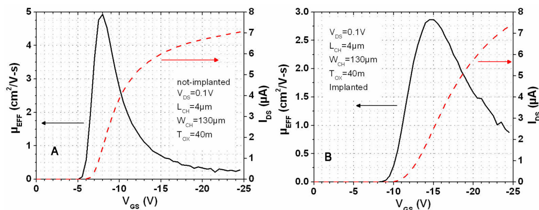
FIGURE 4.41 – Effective mobility in a PMOS of a ALS7 (a) and ALS8 (b)
