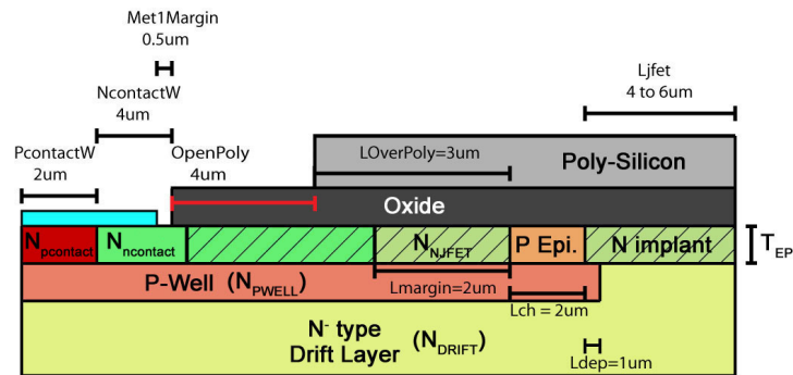
FIGURE 2.25 – Schematic cross section of the VIEMOS cell. The Red and orange areas are the p-type areas, the green and yellow are the n-type ones. The blue is used for the metallic layer, the dark grey for the gate oxide and the light grey for the polysilicon gate
