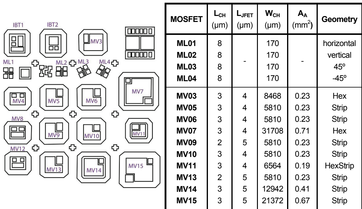
Figure 1 - ESCAPEE Layout for VDMOS fabrication
