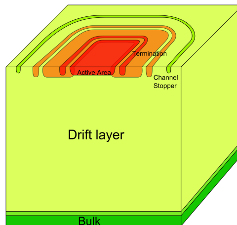
FIGURE 2.23 – Combination of JTE, AGR and JTE Rings on a PiN diode
