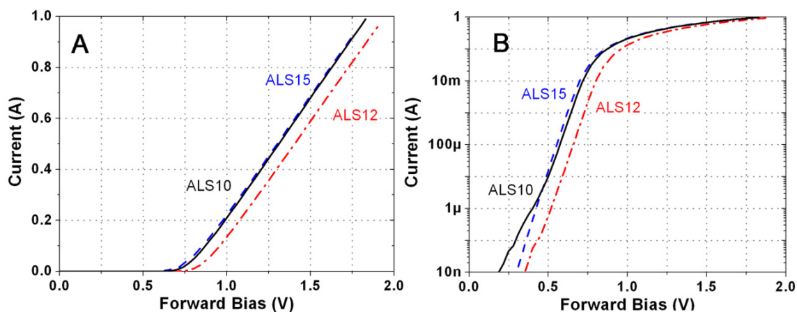
FIGURE 3.13 – Typical Forward characteristics of 4.41\text{mm}^2 Schottky diodes on ALS10, ALS12 and ALS15 represented in linear scale (A) and logarithmic scale (B)
