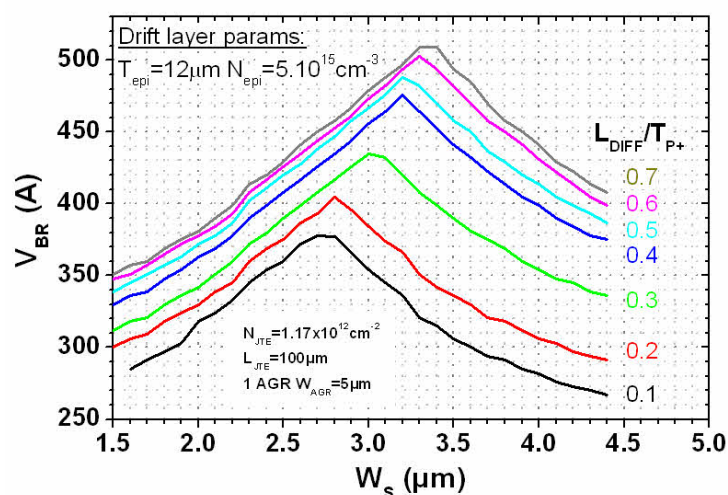
FIGURE 2.8 – Guard ring distance influence on breakdown voltage on termination with one guard ring for a 12\mu\text{m} 5 \cdot 10^{15} \text{cm}^{-3} drift layer with different values of lateral straggling
