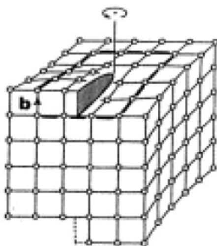
FIGURE 1.22 – Schematic view of a screw dislocation
