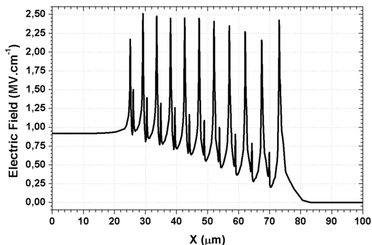
FIGURE 2.10 – Electric field cuts at 400nm from the surface
