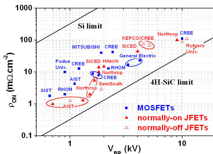
FIGURE 1.13 – Best unipolar power switches in the literature represented on the \rho_{ON} vs V_{BR} graph
