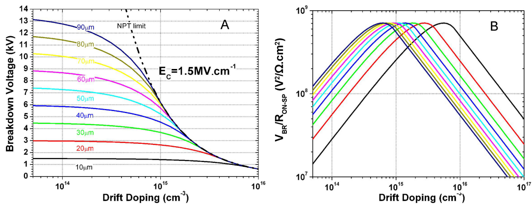
FIGURE 3.1 – Blocking voltage (A) and Baliga Factor of Merit (see table 1.2) (B) vs drift epilayer doping for a low critical electric field and for different drift layer thicknesses. The colours of the curves on figure 3.1B correspond to the same epitaxial layer thicknesses of the curves on figure 3.1A
