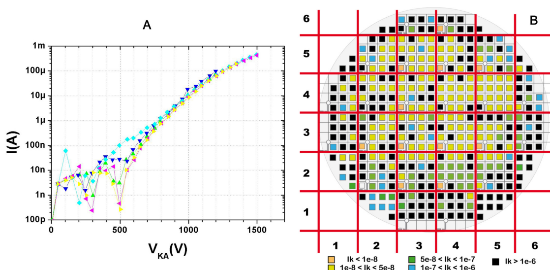
FIGURE 3.8 – (A) Reverse characteristics of 5 Schottky diodes with the same termination design and (B) mapping of the reverse leakage current at 600V on ALS11 wafer
