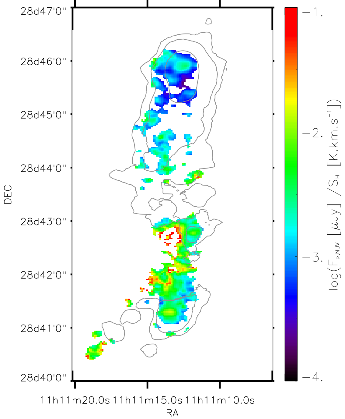
Figure 9.11: Distribution of the NUV/HI ratio across Arp 105, at 4.5 kpc resolution. A logarithmic scale was used for the colour coding, such that the highest value of the ratio is 3 dex higher than the smallest value. Density contours at 0.5 \text{ M}_{\odot} \text{ pc}^{-2} , 1.5 \text{ M}_{\odot} \text{ pc}^{-2} and 5.0 \text{ M}_{\odot} \text{ pc}^{-2} of a 21'' resolution map have been overlaid in grey. Regions of low gas column density can produce high values of the NUV/HI ratio, like in the South-East detached region of the map.
