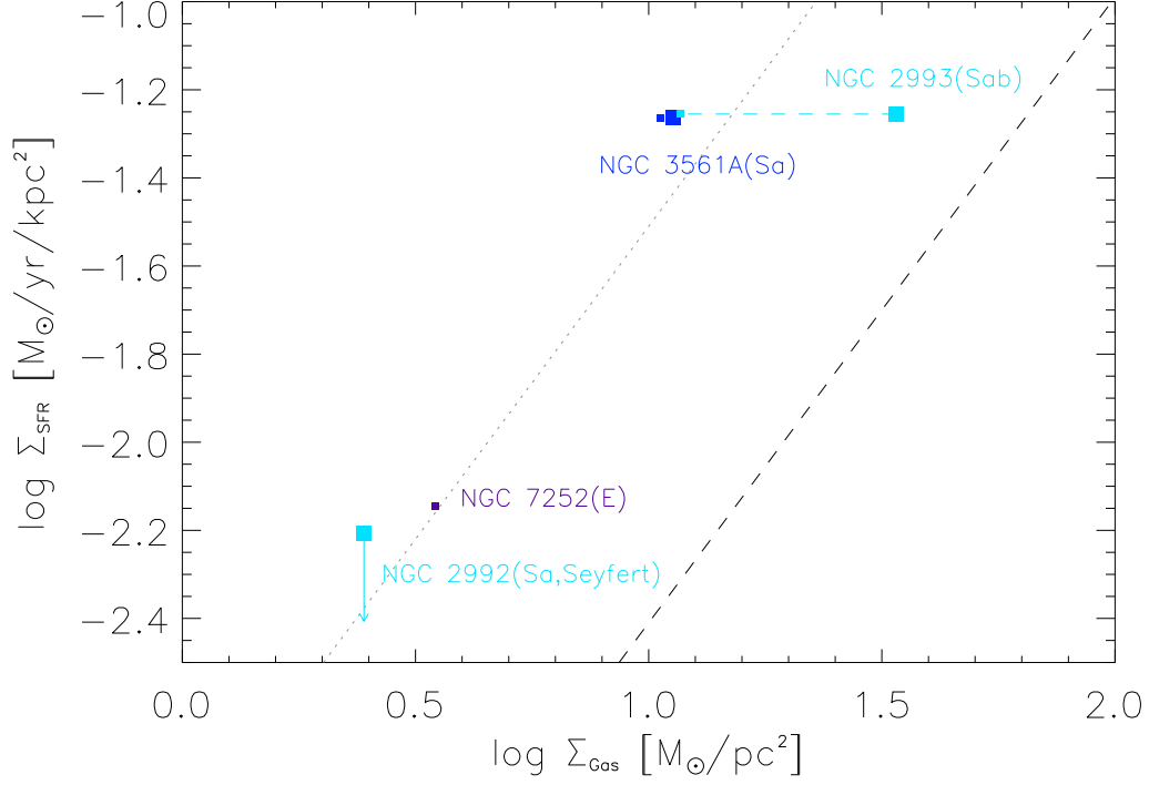
Figure 9.4: Location of the interacting systems on the SK-relation. The integrated values of the total gas, \text{H I} + \text{H}_2 plus helium contribution (large squares), the molecular gas, \text{H}_2 plus helium contribution (small squares), and SFR within R_{25} are plotted. The dashed line shows the locus of regular star-forming galaxies, whereas the dotted line corresponds to the starburst sequence, as defined by Daddi et al. (2010b) .
