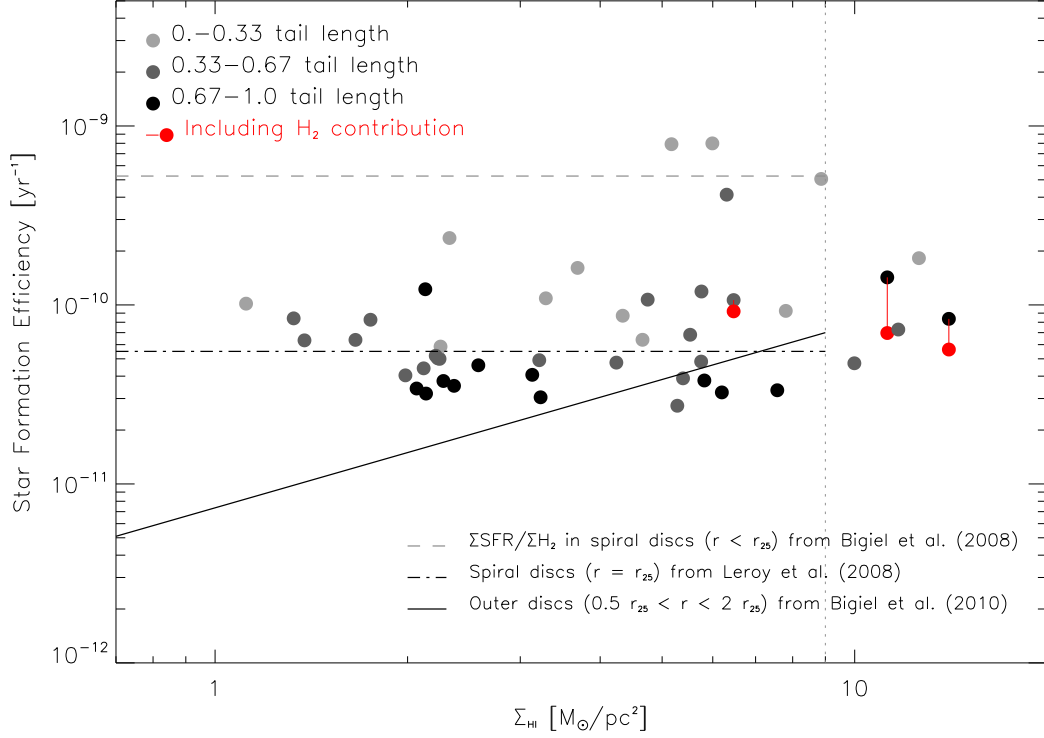
Figure 11.2: Star Formation Efficiency versus H I surface density in our merger sample, grouped into three bins of increasing distance to the central galaxy. Black and grey filled circles represent SFEs computed using the atomic gas component only, instead of the total gas mass. We checked the validity of this approximation for the outer regions of mergers for three star-forming regions with available CO data and thus for which we could determine the H I+H 2 mass (red points). The solid line corresponds to a power-law fit to the SFE versus \Sigma_{\text{HI}} relation for the H I-dominated regime that prevails in the outer discs of spirals (Bigiel et al., 2010). The slope is about \sim 0.7 . The dashed horizontal lines represent various estimates of the SFE at several galactocentric radii in isolated spirals computed using the total gas (H I+H 2 ) (Leroy et al., 2008) or H 2 only (Bigiel et al., 2008). All SFEs plotted in the figure take into account the contribution of Helium (a factor of 1.34 like in Bigiel et al. (2010)).
