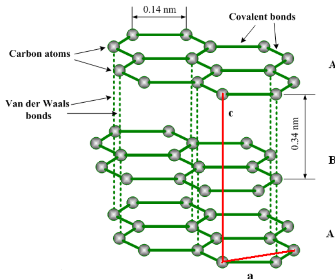
Figure 5 : Structure cristalline du graphite
