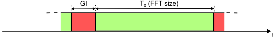
Figure 3.1: CP-OFDM timing.
