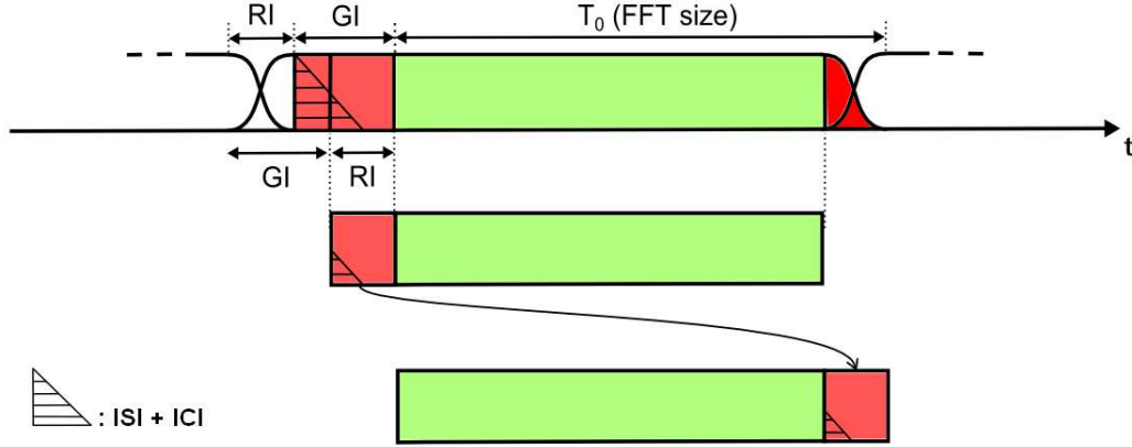
Figure 3.6: Window and GI removal at the receiver side.
