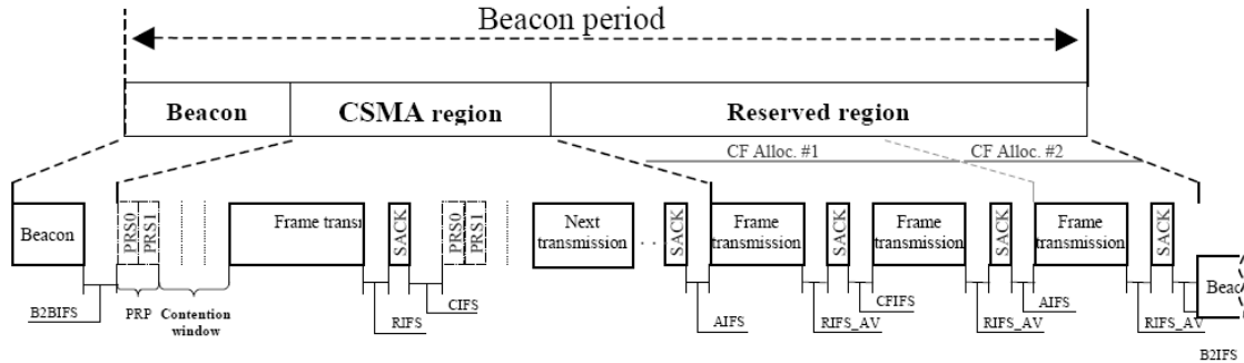
Figure 2.7: HPAV Beacon period [87].
