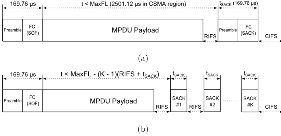
Figure 5.7: Transmission schemes: (a) HPAV unicast [7] (b) HPAV-compliant multicast.
