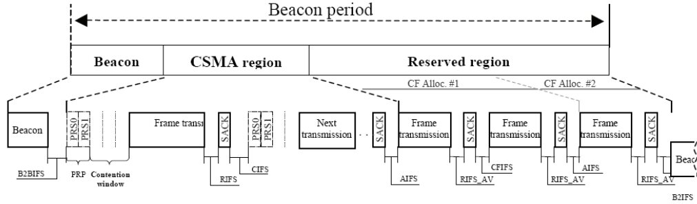
Figure 2.7: HPAV Beacon period [87].
