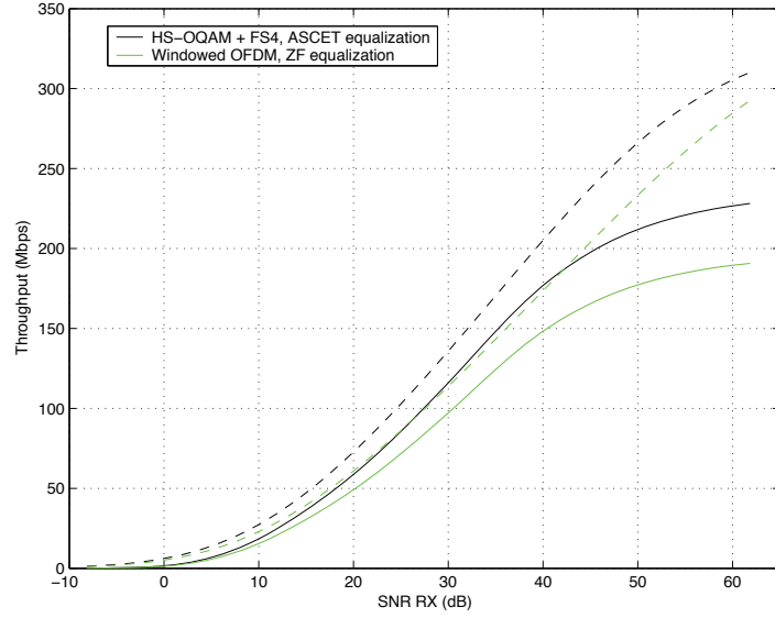
Figure 3.19: Transmission capacities (dotted curves) and PHY data rates (continuous curves) in the HPAV 1 context on Class 5 channels.
