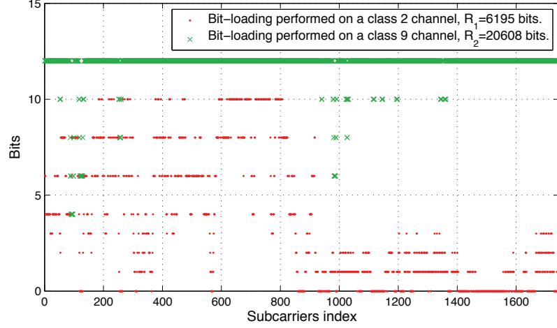
Figure 4.2: Bit-loading performed in the [1.8, 50] MHz frequency range, following the IEEE P1901 specification.
