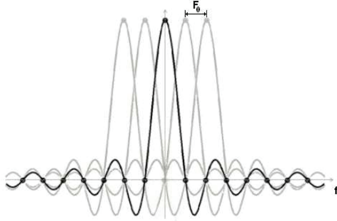
Figure 3.3: Frequency Orthogonality of an OFDM Signal.
