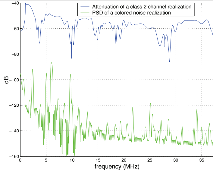
Figure 3.12: Example of class 2 channel and colored noise realizations.
