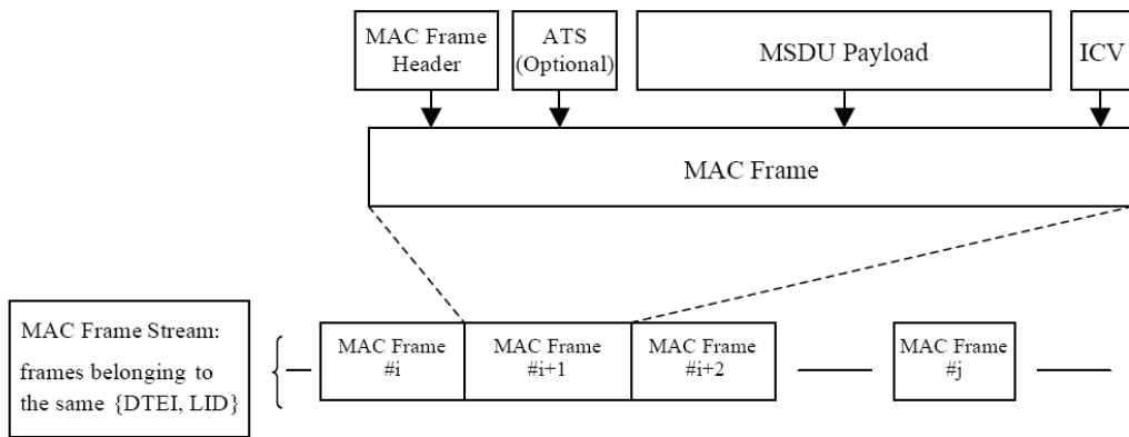
Figure 2.10: MAC frame format [4] [7].
