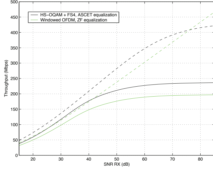
Figure 3.18: Transmission capacities (dotted curves) and PHY data rates (continuous curves) in the HPAV 1 context on Class 9 channels.
