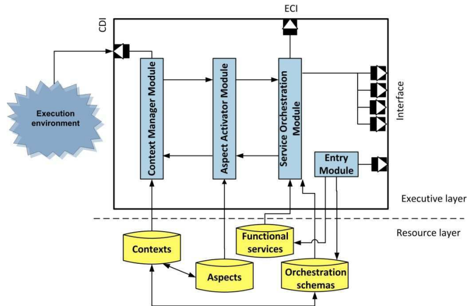
Figure 4.1. Architecture générale du service domaine [Boukadi et al., 2008b]
