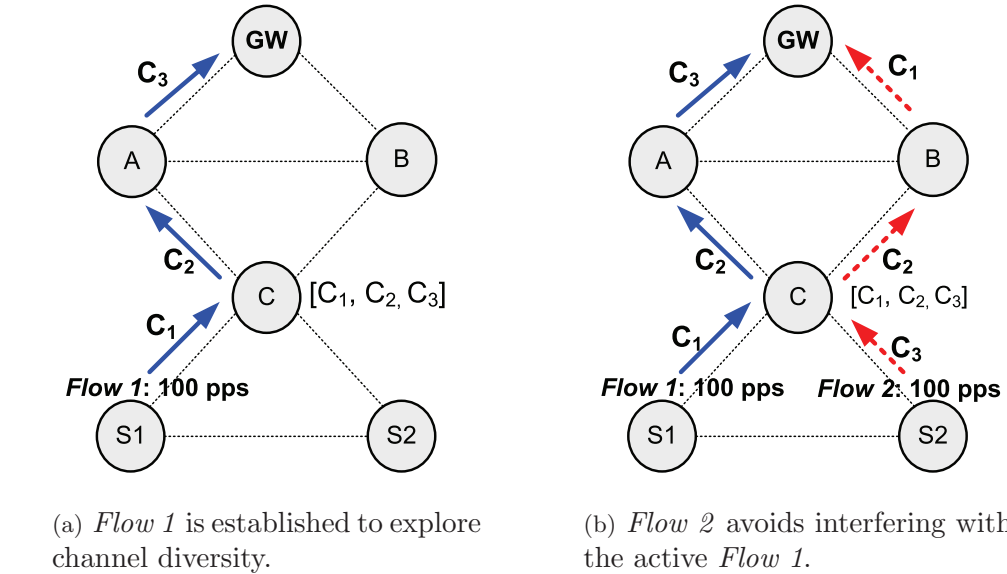
Figure 6.5: Operation of our Path Selection Protocol.
