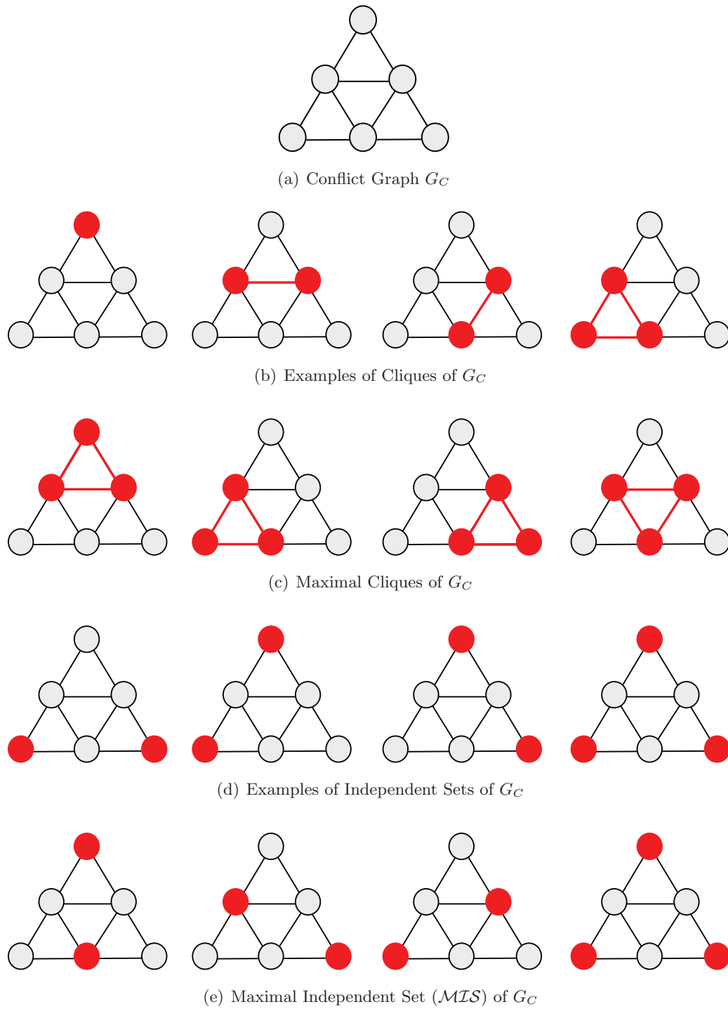
Figure 5.1: Understanding Some Concepts of Graph Theory used in our MILP Formulations.
