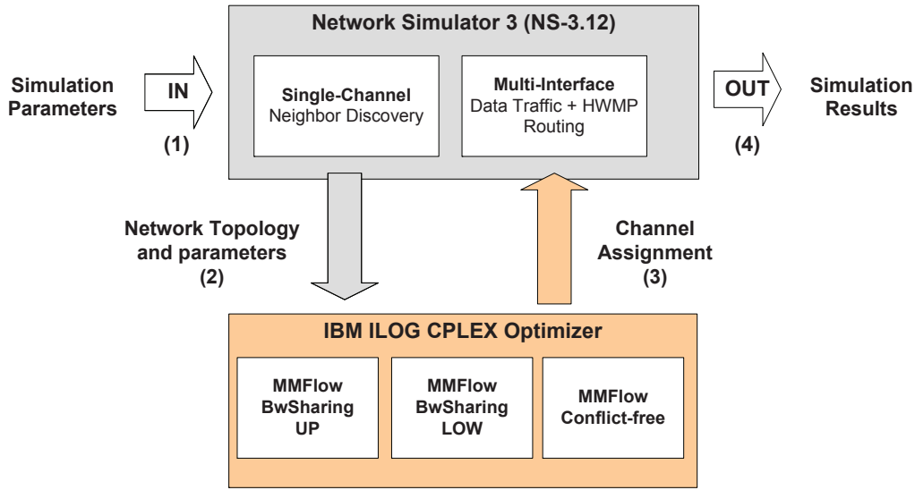
Figure 5.3: A diagram that depicts the interaction between NS-3.12 and the IBM ILOG CPLEX Optimizer.
