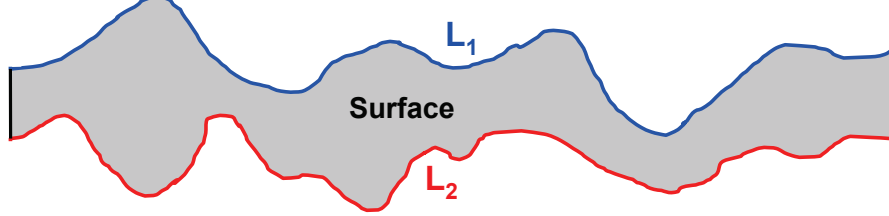
Figure 2.4: Surface representation between two lines.
