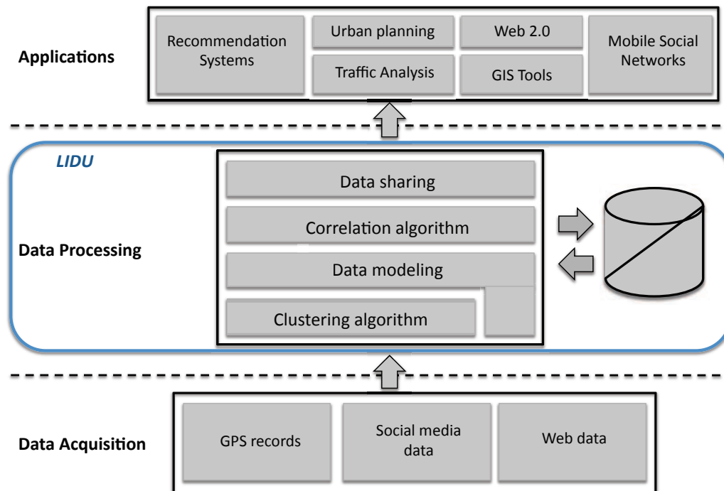
Figure 5.1: Architecture overview.
