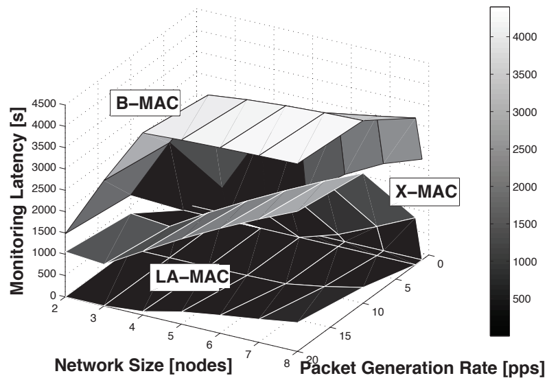
(a) Latency vs. traffic load.
