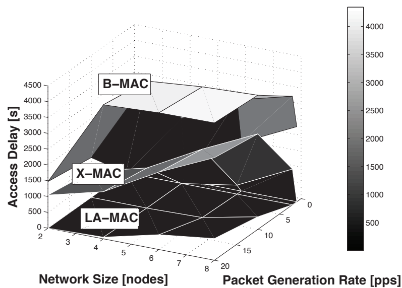
(b) Access delay vs. traffic load.
