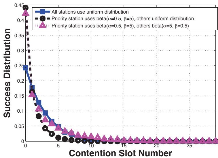
FIGURE 5.14 – Distribution of success when random slots are allocated following the Beta distribution. Comparisons of several differentiation scenarios for N=10, K=30 .
