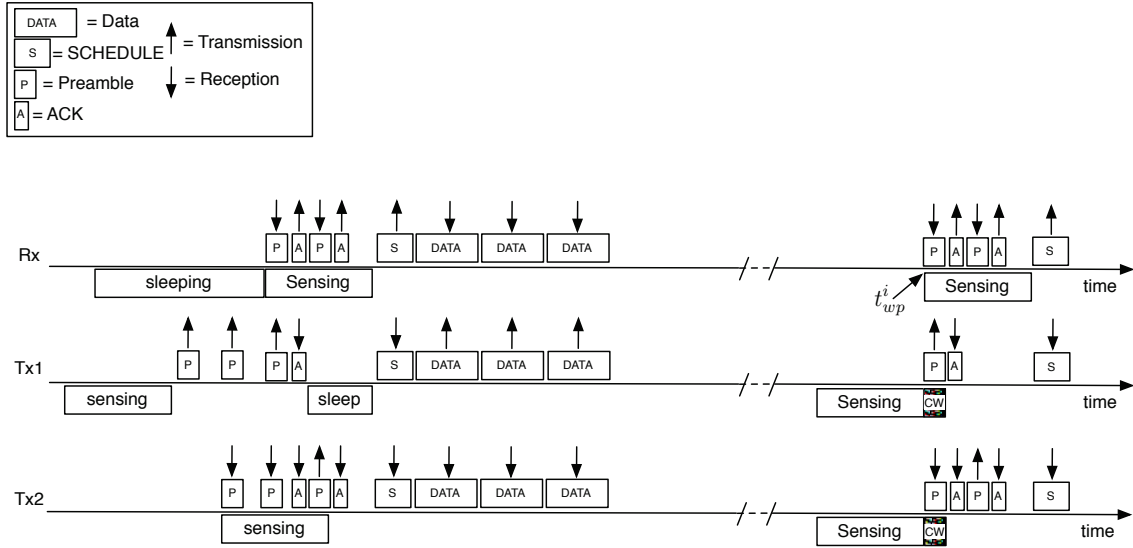
FIGURE 3.5 – LA-MAC operation during the transmission of a burst of broadcast data frames with adaptive wake-up schedule mechanism enabled.
