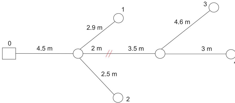
Figure 2.17: Example of a network with two junctions and matched terminations. The red line indicates the path along which we will observe the ZT diagram.
