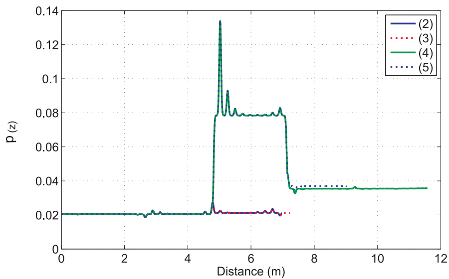
Figure 4.29: The power summation diagram along the four branches of the network illustrated in Fig. 4.28.
