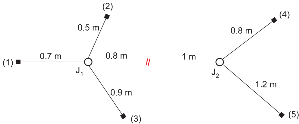
Figure 4.18: A double-junction network with testing ports at each of the extremities, representing the network we used to illustrate the derivation of the fault location method.
