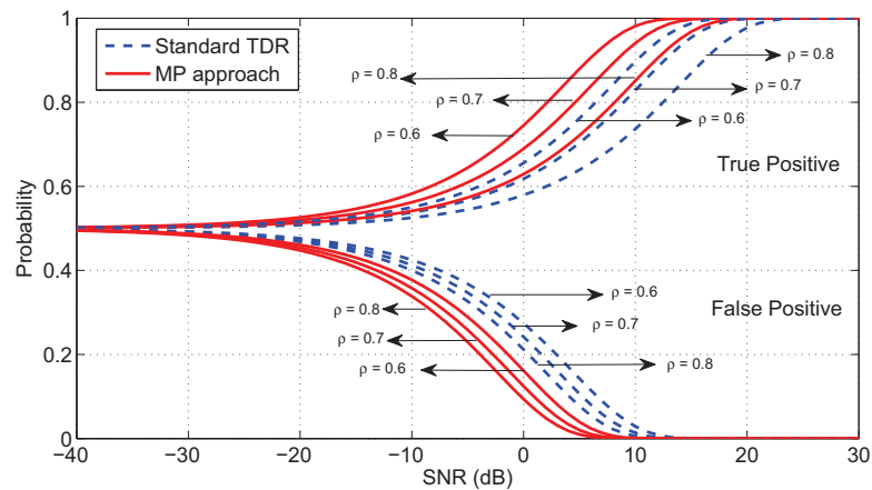
Figure 3.19: The detection probabilities corresponding to the case Fig. 3.6(a) with open circuit ends and a fault value of 250 \Omega . Three values of the detection threshold were considered: 0.6, 0.7 and 0.8.
