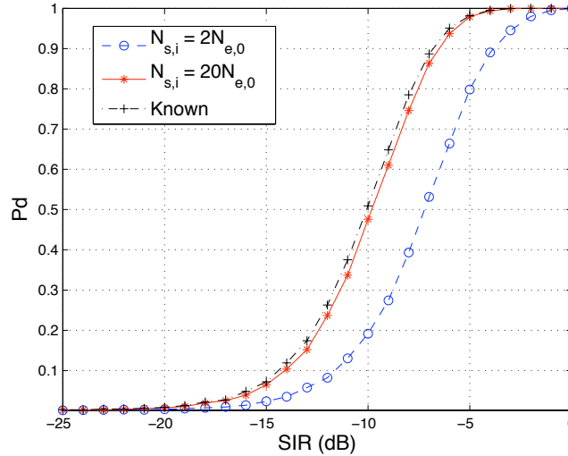
Figure 2.17: P_d against \text{SIR}_{\text{pre}} with the adaptive MIMO GLRT-LQ using FPE and interference with Gamma-distributed texture ( a = 2 ). Stationary target model.
