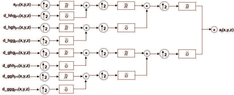
Figure 4.5: Reconstruction of an image A_{2^{j+1}}^d f from A_{2^j}^d f and D_{2^j}^i f . The x ( y , z )-direction samples are convolved with one dimensional filters \tilde{H} and \tilde{G} .
