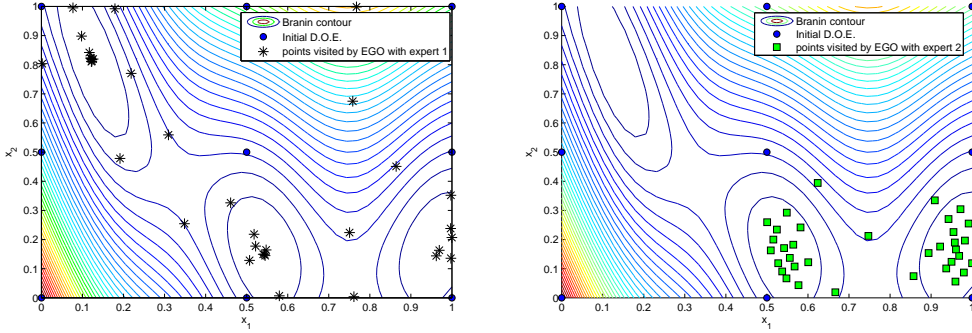
Figure 2: 25 iterations of the EGO algorithm applied to the Branin-Hoo function, with both experts \mathcal{E}_1 and \mathcal{E}_2 (see eq.(3)) and initial design \mathbf{X} (in dark dots). Left: the path of EGO with expert \mathcal{E}_1 is represented by dark thin stars. Right: the path of EGO with expert \mathcal{E}_2 is represented by light squares. One of the three zones of minimum (upper left) is not visited.
