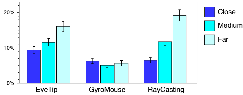
Figure B.3: Error rate ( Outside Clicks ) per GAP × TECHNIQUE.
