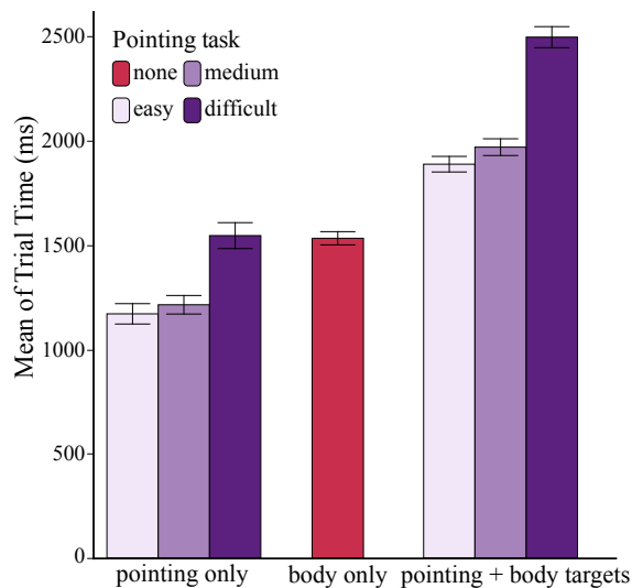
Figure 3.8: TRIAL TIME for all tasks (pointing only, body only, combined pointing + body) by pointing difficulty.
