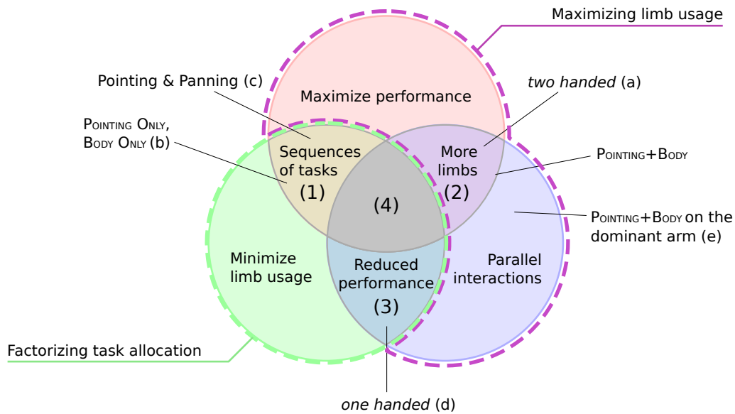
Figure 3.13: Trade-off between limb usage, performance and parallelization of interactions, within the Task Allocation taxonomy developed in Chapter 1. one handed and two handed refer to the corresponding conditions from Chapter 2. POINTING ONLY, BODY ONLY and POINTING+BODY refer to the corresponding conditions from Chapter 3. “Pointing & Panning” refers to the sequential arrangement of pointing and panning in Chapter 2.
