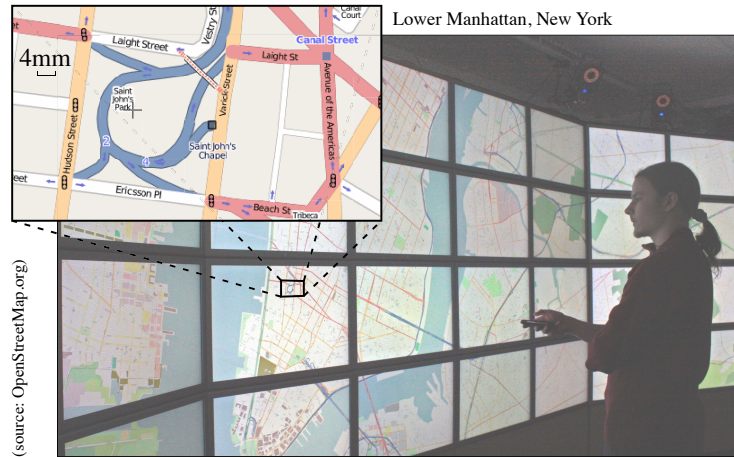
Figure 4.1: The interactive wall-sized (5.5m × 1.8m) ultra-high-resolution (20 480 × 6 400 = 131 million pixels) display used for our studies. Inset: magnification of a 9cm × 5cm area.
