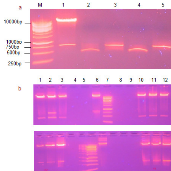
Figure E8: PVP binding scFv:: streptavidine (a) Before ligation of streptavidine gene and PVP ScFv, M- DNA marker, 1- pUX SF9 :: streptavidine clone (Nco I- Not I digested, dephosphorylated) expected insert (10kb and 750bp), lane 2- B1 scFV (expected size 500bp), lane 3- A2 ScFv(750bp), lane 4- C11 ScFv (500bp), lane 5- F1 ScFv (750bp) (b) Screening of positive clones for PVP ScFv:: streptavidine, digestion with Nco I- Not I
